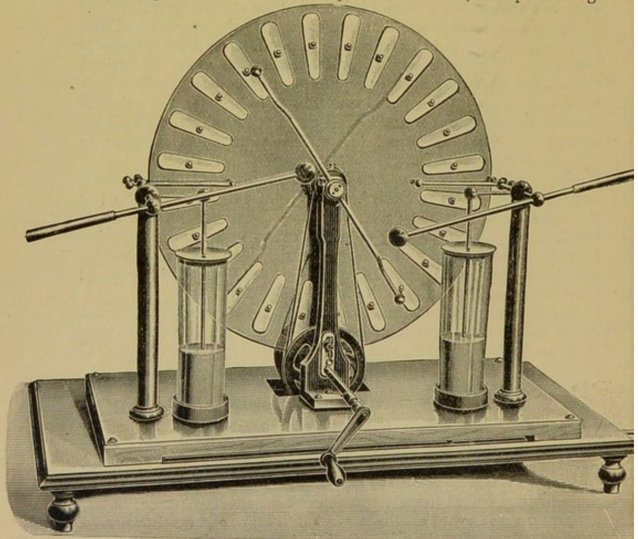
Fig. 59.—Wimshurst Machine.—Modified by Schall.
