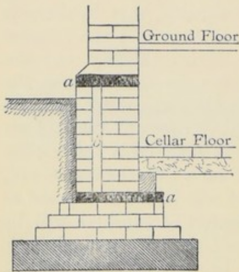
FIG. 74.— a , damp-proof courses ; b , air-space.
