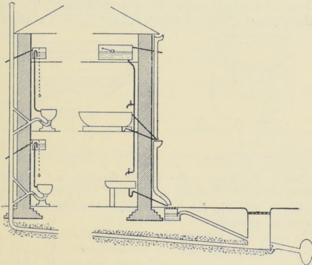
FIG. 92.—House with good sanitary arrangements.
