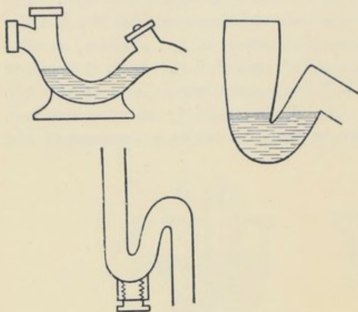
FIG. 90.—Various forms of syphon trap.
