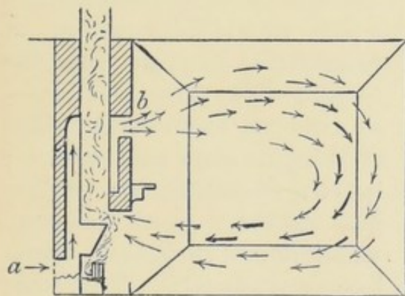
FIG. 82.—Galton's fire grate.
