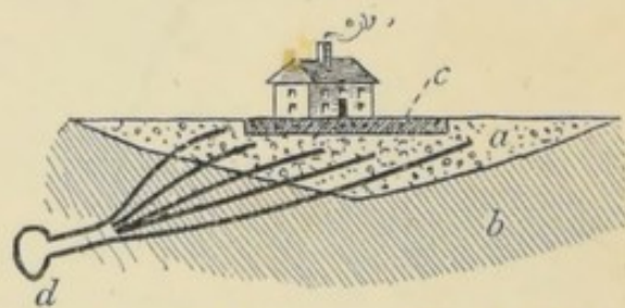
FIG. 73.—Bad site improved. a , refuse; b , clay; c , concrete; d , drain.
