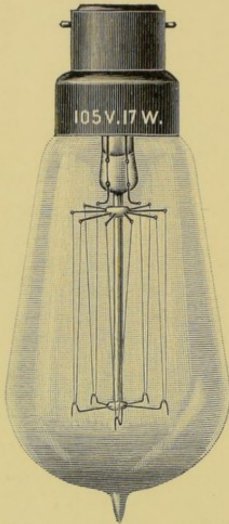
FIG. 197.—An "Osram" Lamp with Tungsten Filament.
