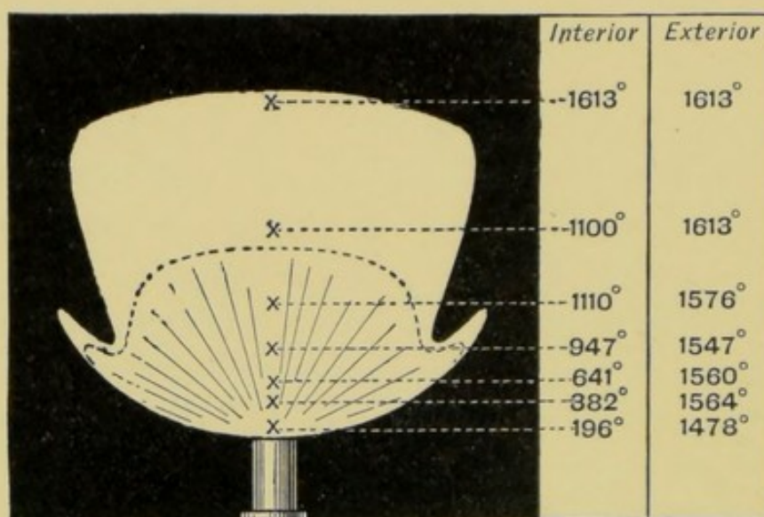
FIG. 172.—Temperatures in Gas Flame (Smithells).
