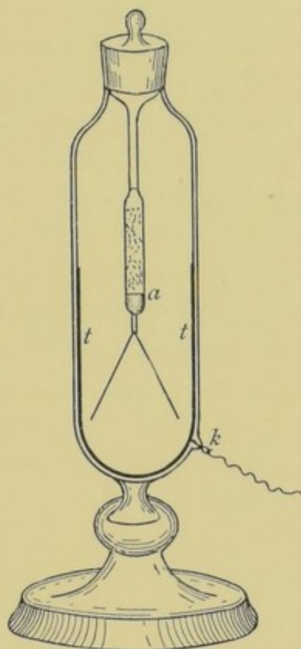
FIG. 170.—Strutt's "Radium Clock."
