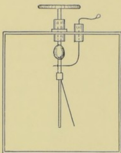
FIG. 161.—Electroscope suitable for Observation of Radio-Activity.
