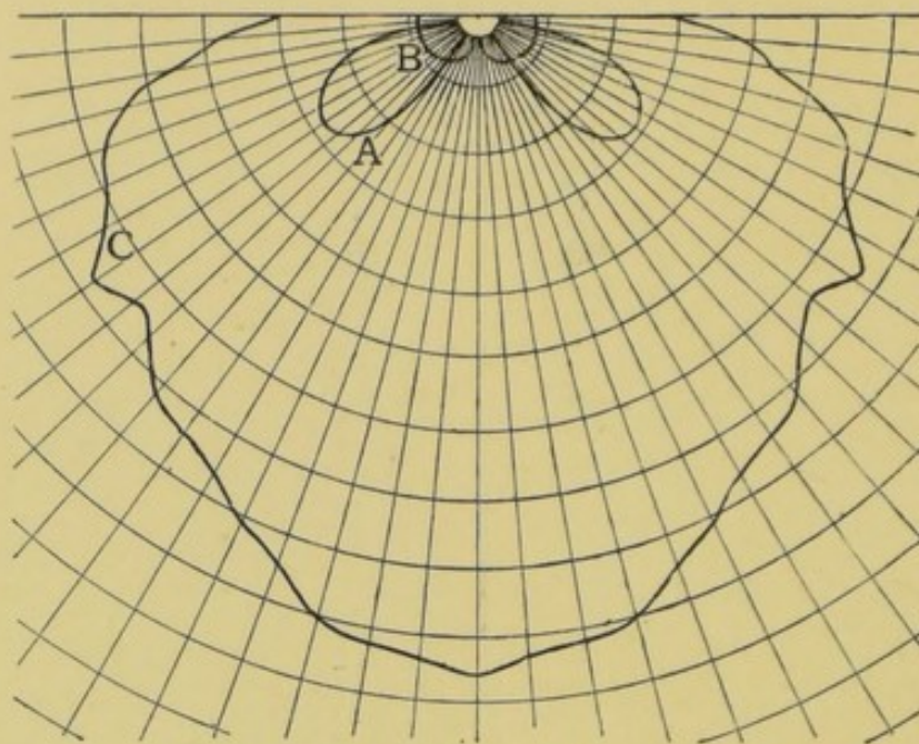
FIG. 199.—Curves of Distribution of Light of Arc-lamps.
