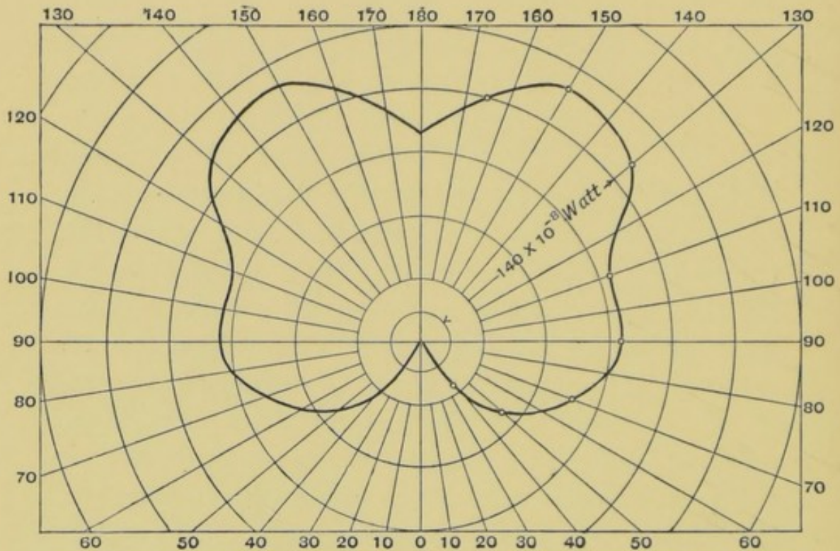
FIG. 175.—Distribution of Luminous Rays of Paraffin-Lamp (Wedding).
