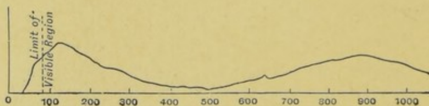
FIG. 190.—Rubens' Curve for Emissivity of Welsbach Mantle.
