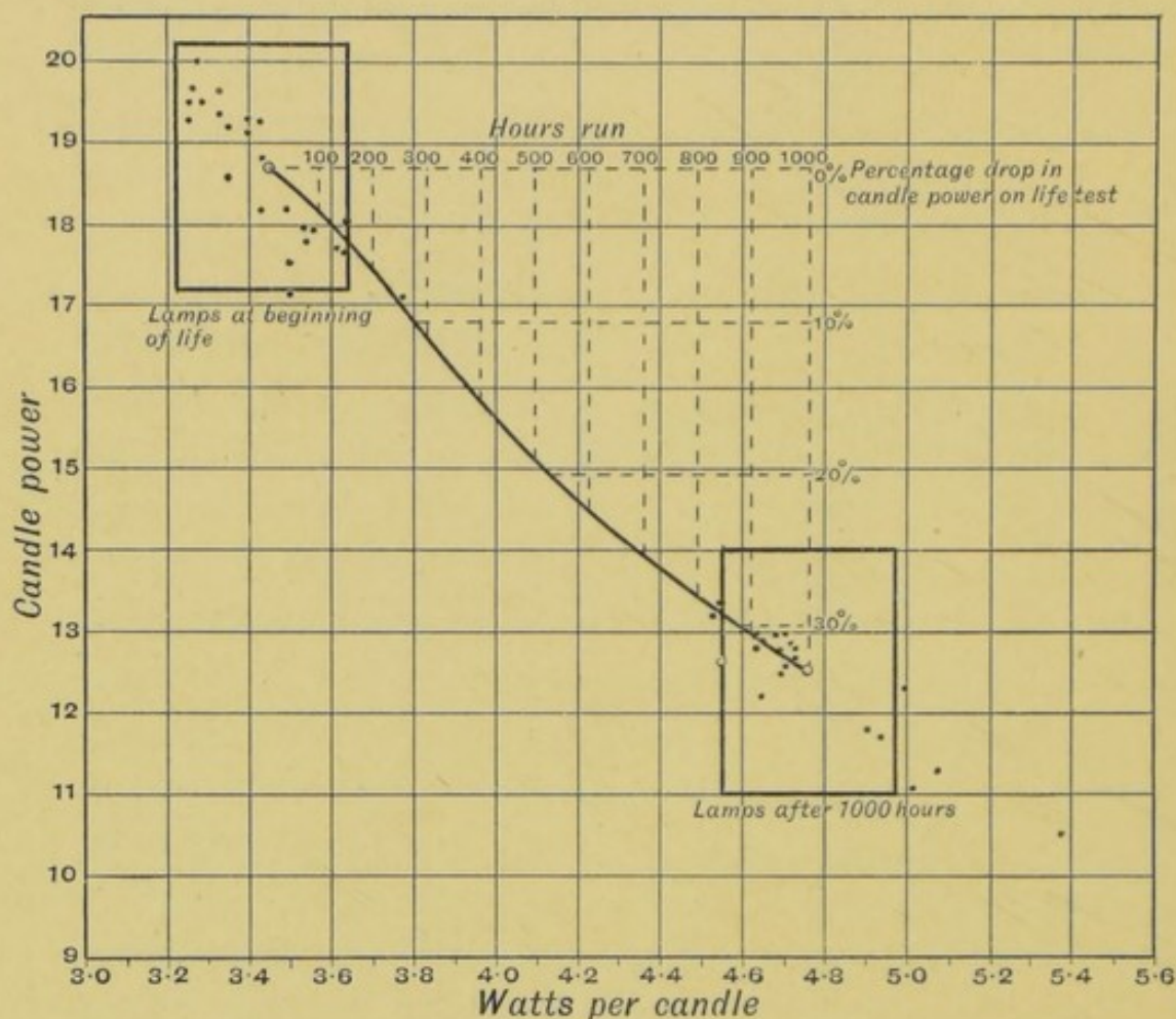
FIG. 193.—Test-chart of Twenty-four Electric Glow-lamps.
