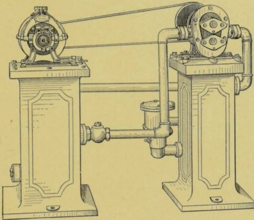
FIG. 191.—Colonia Gas Compressor for High-pressure Incandescent Gas-lighting.
