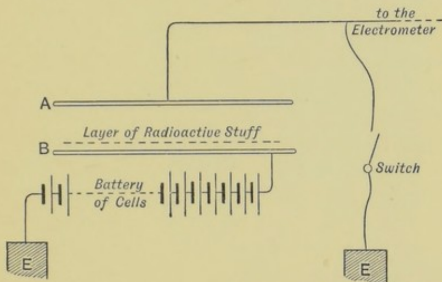
FIG. 162.—Madame Curie's Apparatus for detecting Radio-Activity.
