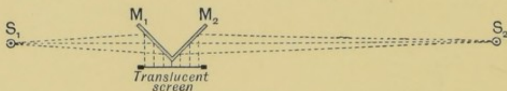
FIG. 173.—Diagram of Simple Photometer.
