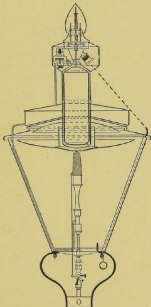
FIG. 192.—Scott-Snell self-contained High-pressure Gas Lamp.
