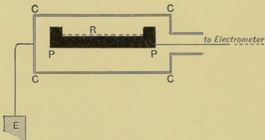
FIG. 169.—Experiment on electrification by Alpha-rays.
