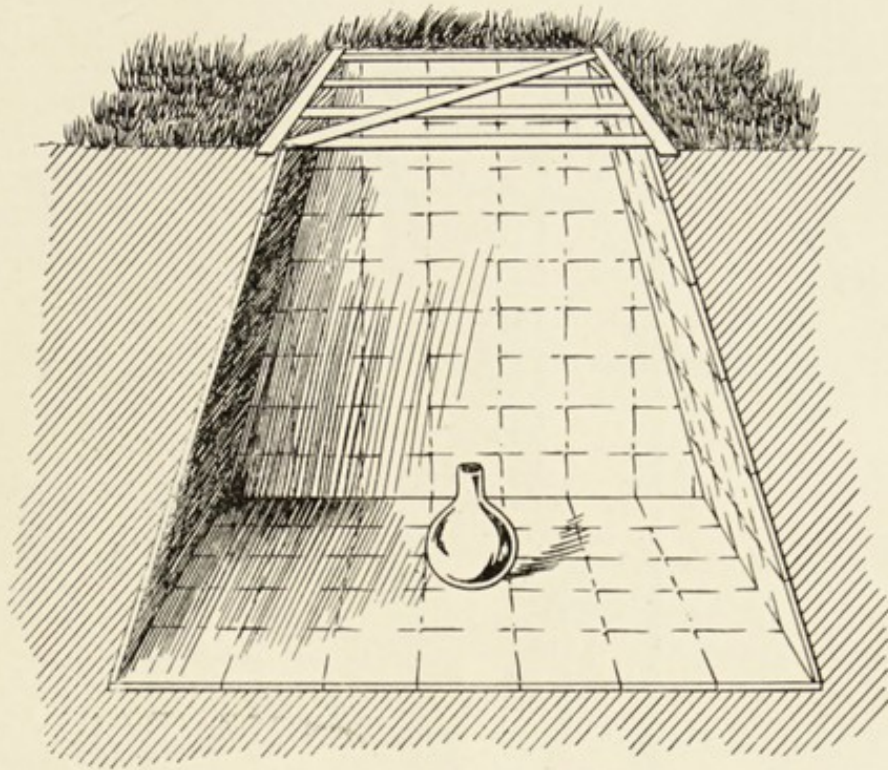
“ RAT-PIT.”
