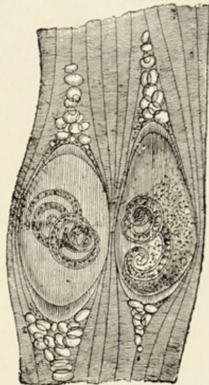
ENCYSTED TRICHINA.
