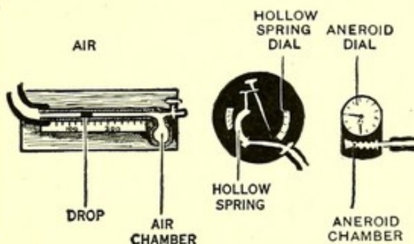
FIG. 21.—Types of manometer used for determining blood-pressure.
