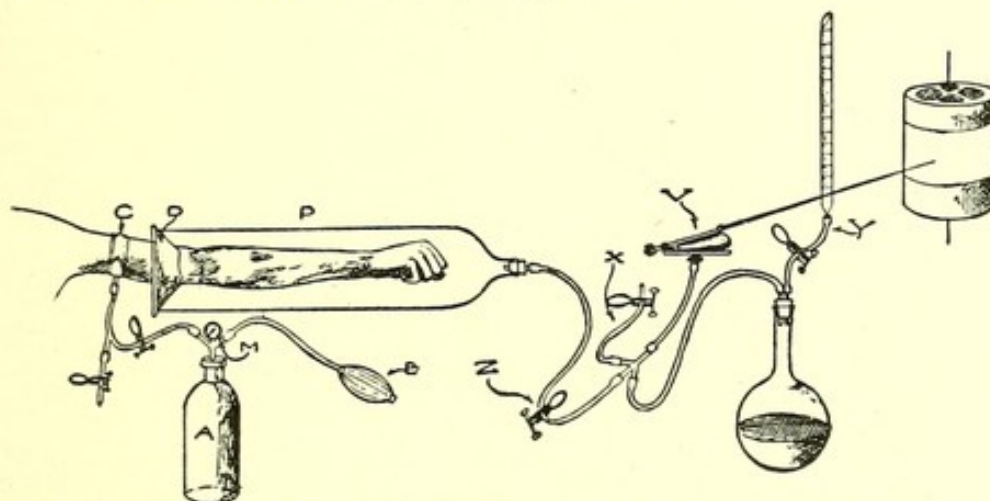
FIG. 28.—Diagram of apparatus for determining the rate of blood flow through the arm. (A. W. Hewlett and G. Van Zwaluwenburg.) The arm is placed in the plethysmograph, P , the opening of which is closed by a piece of rubber dam, D , and the connection with the skin made tight with soapsuds. The narrow pressure cuff, C , is placed around the arm about 3 cm. above the opening into the plethysmograph. The pressure cuff is inflated by opening the stop-cock connecting it with the large bottle, A , in which the pressure has previously been raised by the rubber bulb, B . Pressures are read by the spring manometer, M . The plethysmograph is connected with the volume recorder, V , which writes upon a moving drum. Air can be let out of the system by the stop-cock, X , and water can be introduced from the burette, Y , so that the writing point of the volume recorder can be adjusted at will. The stop-cock, Z , serves to disconnect the plethysmograph from the recording apparatus during adjustments of the former. The recording apparatus is graduated by allowing 5 cc. of fluid at a time to flow in from the burette, and marking the elevation of the volume recorder thus produced.
