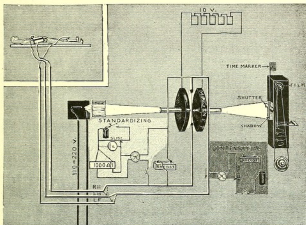
FIG. 58.—Diagram showing the main connections for the electrocardiograph. The heaviest lines (110-220 V) mark the electric light connections; the medium lines indicate the main circuit from right hand (RH), left hand (LH) or left foot (LF) of the patient through the galvanometer, showing the shunt through the rheostat (RHEOST). The galvanometer is shown between the two poles of the MAGNET, which is charged by the storage battery circuit (10 V). The connections for the compensating current, shown in the darkly shaded area; those for the standardizing current are shown in the lightly shaded area. The construction of the photo-registration apparatus is shown upon the right of the figure.
