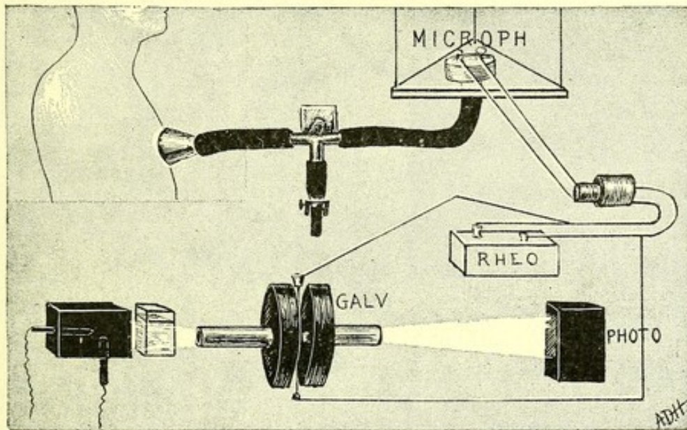
Diagram showing the connections for taking graphic records of the heart sounds by means of the Einthoven galvanometer; MICROPH, microphone suspended upon a Julius suspension; GALV, galvanometer; RHEO, rheostat; PHOTO, photoregistration apparatus. The telephone induction coil is shown upon the right of the figure.
