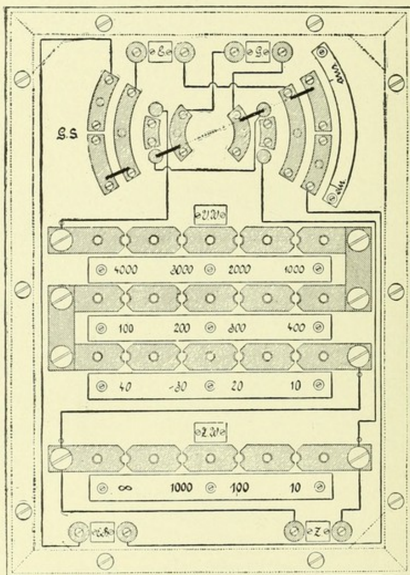
FIG. 57.—Edelmann's convenient switchboard and short-circuiting keys.
