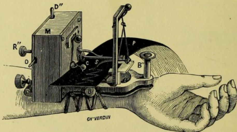
FIG. 123.—Dudgeon's sphygmograph.
