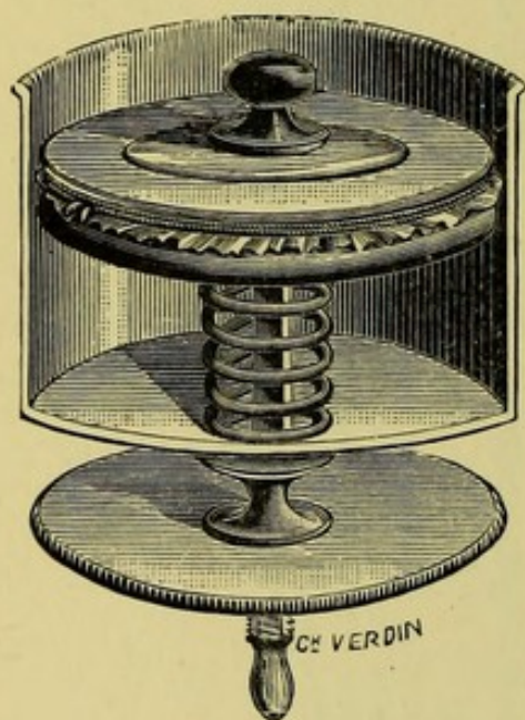
FIG. 106.—Marey's cardiograph.
