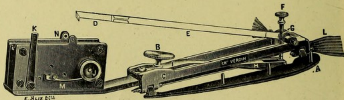
FIG. 120.—Marey's sphygmograph.
