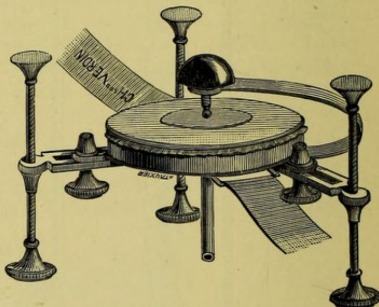
FIG. 107.—Burdon-Sanderson's cardiograph for the apex beat.
