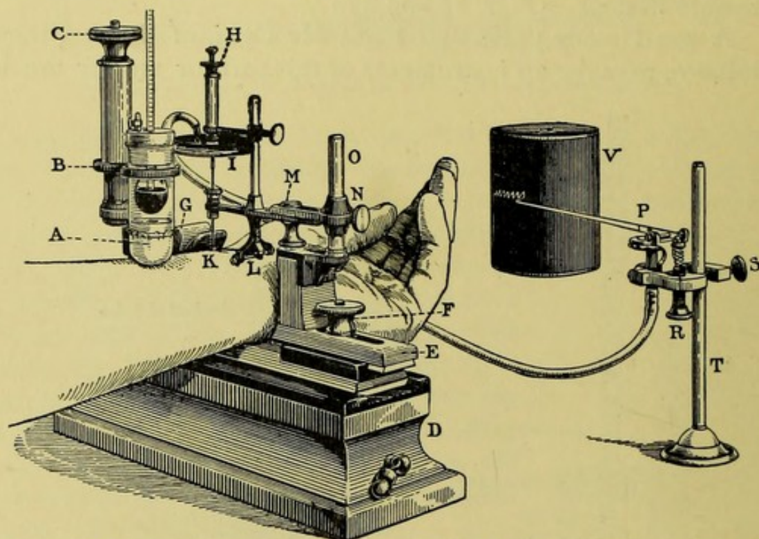
FIG. 83.—Von Basch's sphygmomanometer and stand. Drawn from one in the author's possession. A is the india-rubber cap of the sphygmomanometer resting on the radial artery. B is a metal ring which holds the sphygmomanometer, and can be raised or lowered at will by the screw C. D is the stand in which the arm rests. E is a sliding piece which holds the arm in position, and also supports the sphygmograph I. F is a screw to fix E in position. G is a fixed projection at the other end of D, and the wrist is clamped between E and G. G consists of two parts, one of which is quite fixed; the other, indicated by K, can be pressed more or less firmly against the arm by a fine screw not shown in the drawing. H is a fine screw by which the tambour of the sphygmograph can be raised or lowered so that it rests with more or less pressure on the top of the rod which passes up from a small pad which rests in the artery. K indicates the position of this pad as well as of the movable piece of G. L is a joint in which a lever plays, the outer end of which is fixed to the pad K, and keeps it moving in a perpendicular line. M is a joint allowing of considerable horizontal play backwards, forwards, laterally, and circularly, so that the sphygmograph may be accurately adjusted over the artery. N is a screw by which the whole sphygmograph may be moved up and down on the stand O. P is one of Marey's tambours, communicating by a piece of elastic tubing with the tambour of the sphygmograph, and writing the pulse on the blackened cylinder V. R is a screw working on a spring, by which the resistance of the lever resting on the tambour may be adjusted. S is a screw by which the tambour may be moved up and down on the stand T. V is a revolving cylinder covered with blackened paper, on which the tracing is taken. It is moved by clockwork, which is not shown in the drawing.
