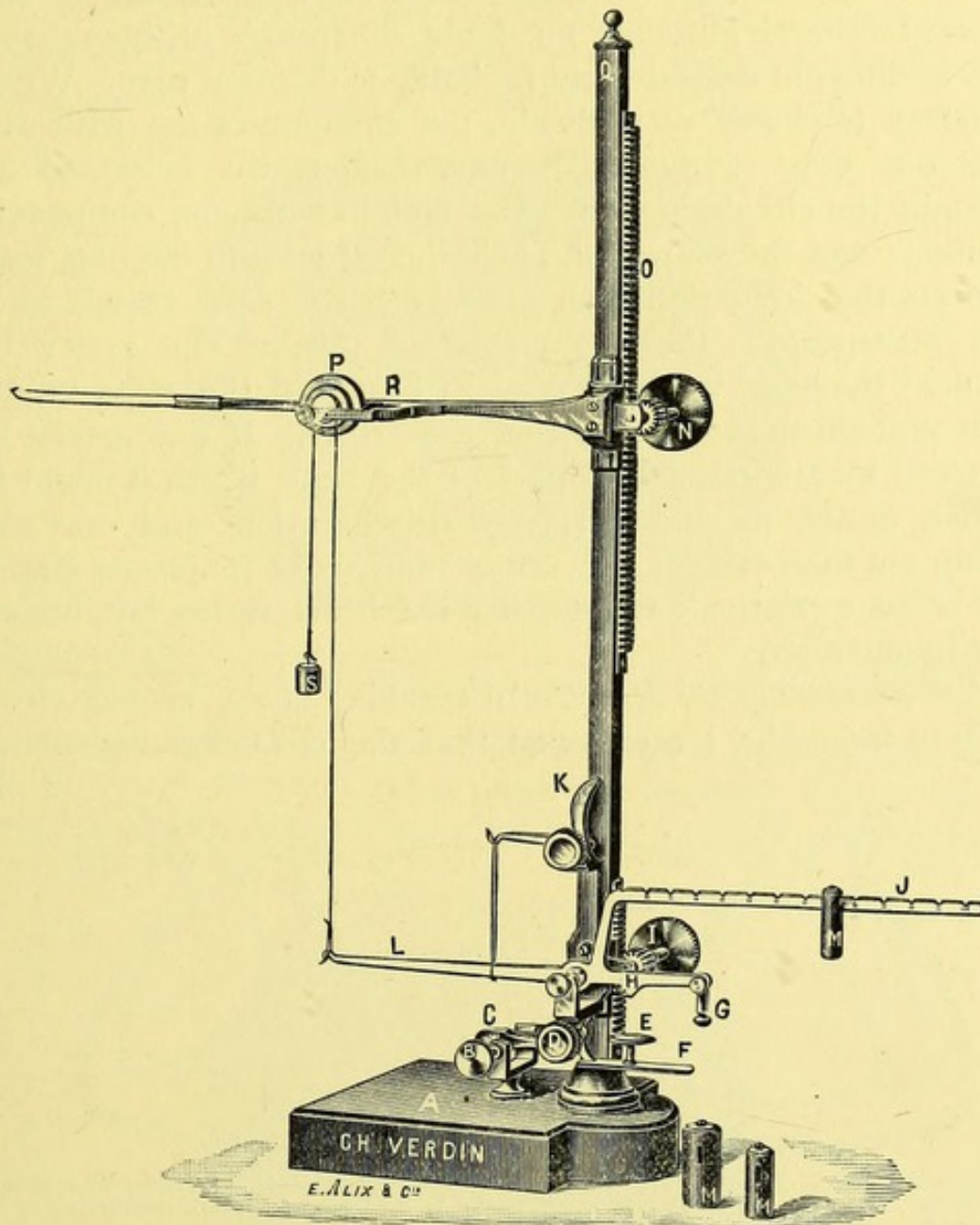
FIG. 124.—Laulanié's digital sphygmograph. E, disc on which the pulp of the finger rests. L, aluminium lever which rests by its projection H on the root of the nail. M is a movable counterpoise which can be moved along the rod J so as to exert on the finger the proper amount of pressure required to obtain the maximum oscillations of the lever. P, pulley with a writing point to magnify the movements of the lever L. G is a rod terminating in a button for taking the radial pulse. In doing this the disc E and the rod F which carries it are moved out of the way, and a heavier counterpoise is employed. K is a bent rod which permits of an india-rubber band being employed instead of the counterpoise. N is a milled head which allows the rod R to be moved up and down on the stem O, and tracings taken at different heights on a revolving cylinder.
