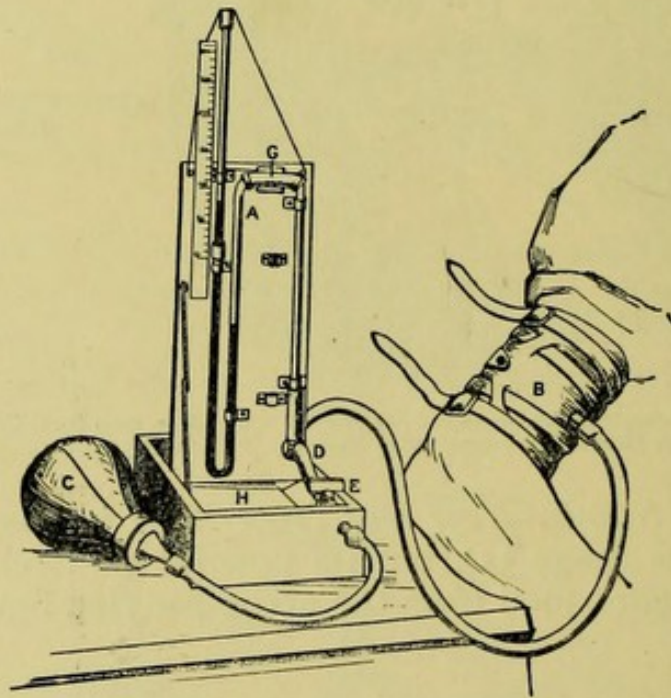
FIG. 234.—Janeway's sphygmomanometer.
