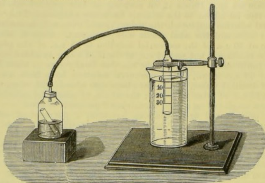
FIG. 94.—Apjohn's apparatus for the estimation of Urea by the hypo-bromite of sodium solution.
