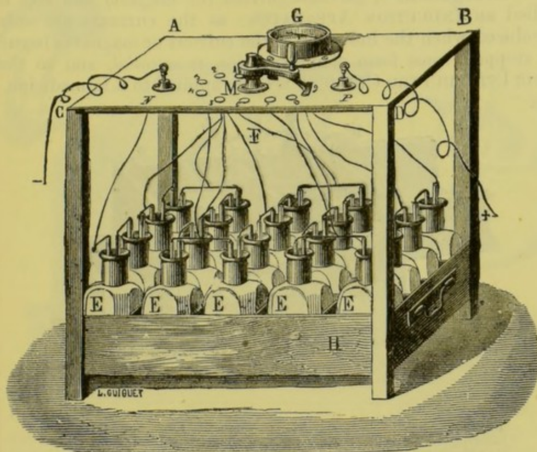
FIG. 36.—Galvanic Battery supplying the "continuous current": 20 elements (E) arranged in series; the terminal conducting wire leading up to the negative pole (N) is shown; there are other wires (F), at stated intervals, going to the studs in the dial collector (M) for making connection with the positive pole (P). A Galvanometer (G) is included.
