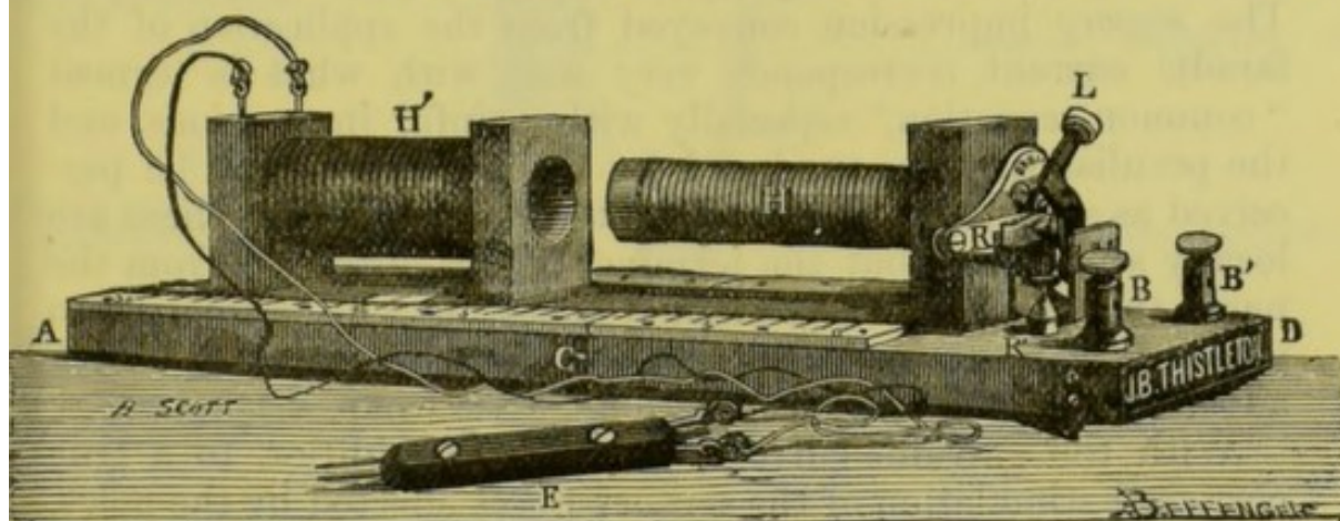
FIG. 39.—Induction Coils, with sledge arrangement, for regulating the strength of current, and a graduated scale: Lever (L) for giving single shocks. Such coils may be driven by a Bichromate or a Leclanché element.
