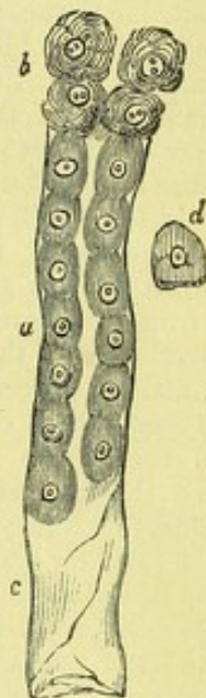
Human Kidney Tubule, magnified 300 diameters.
