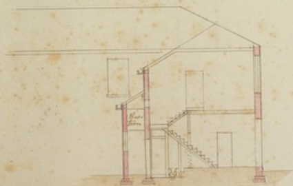
Section showing the stairs &c for the building house.
