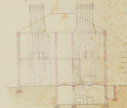
Section of the secretaries' house from the south showing the flues
