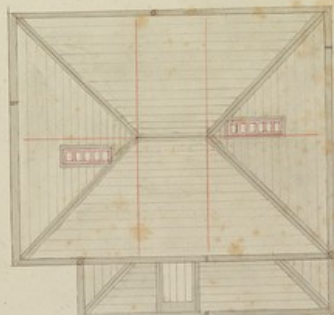
Roof plan for the secretaries' house
