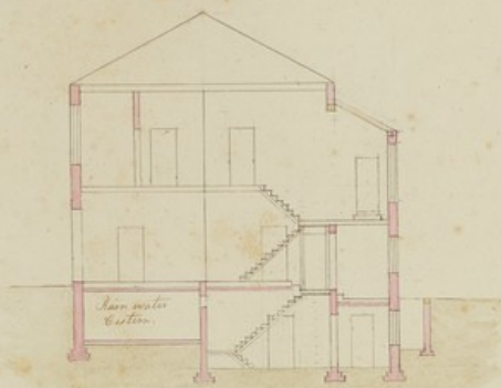
Section through the passage looking east
