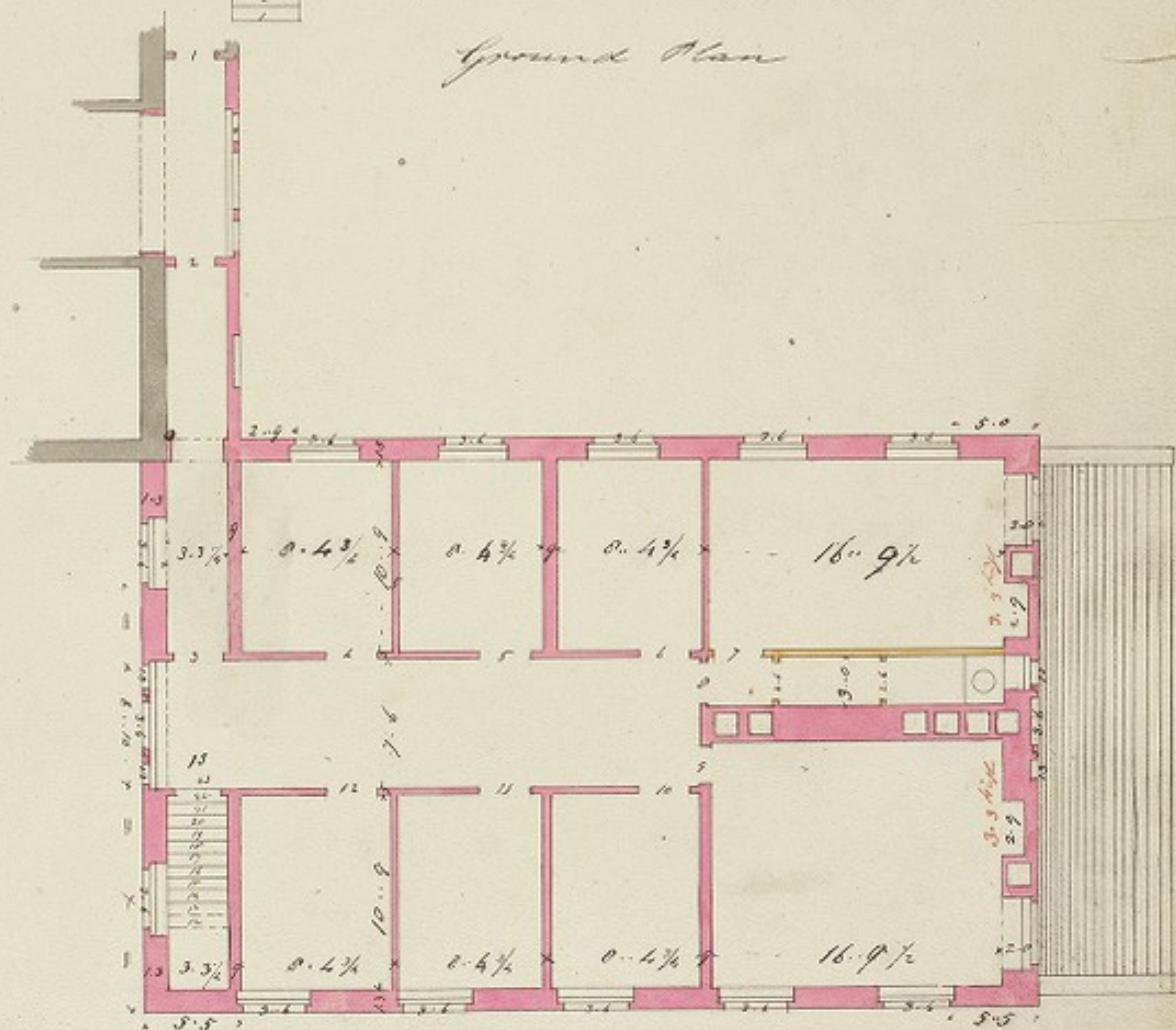
Chamber Plan
