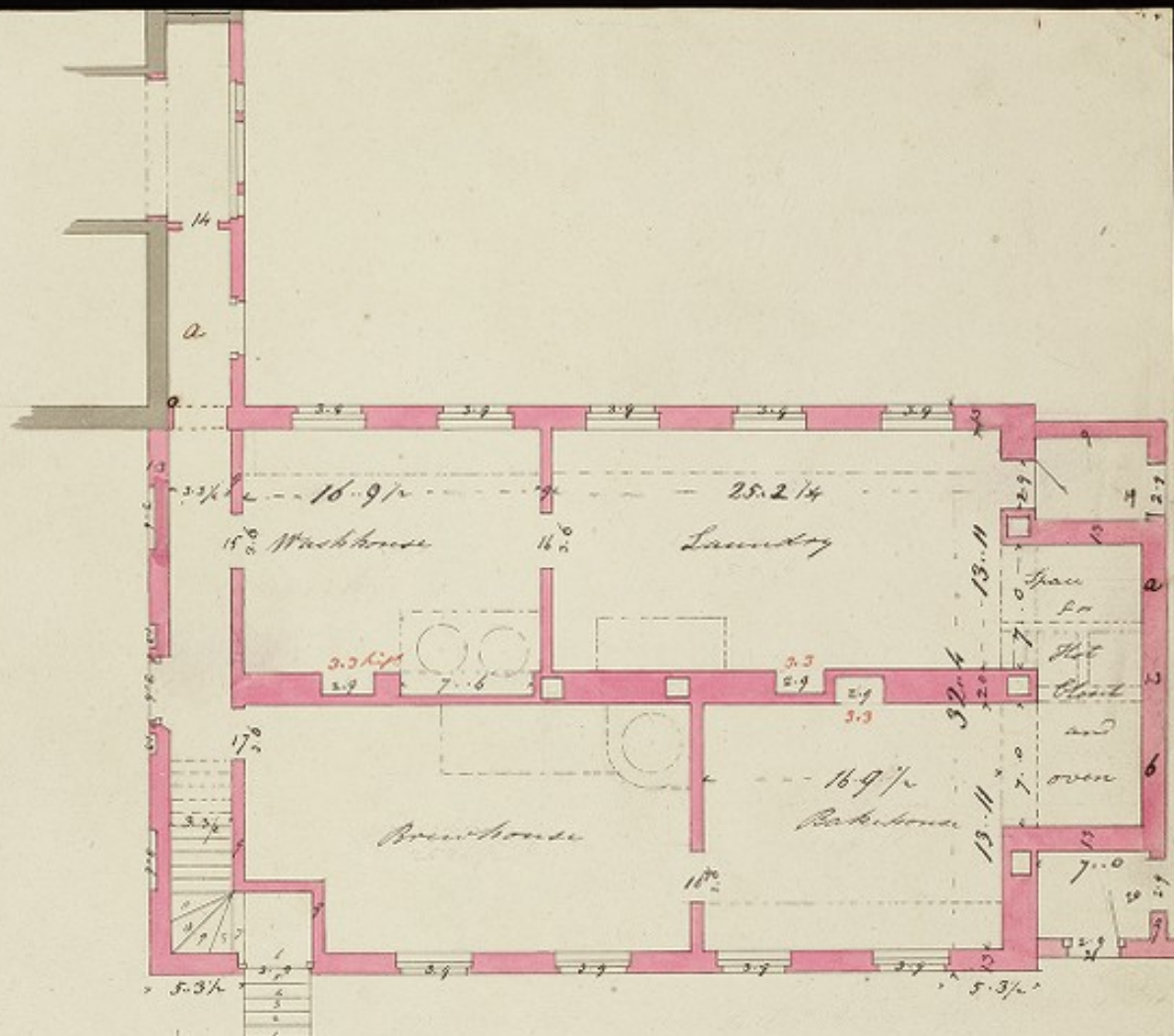
Ground Plan
