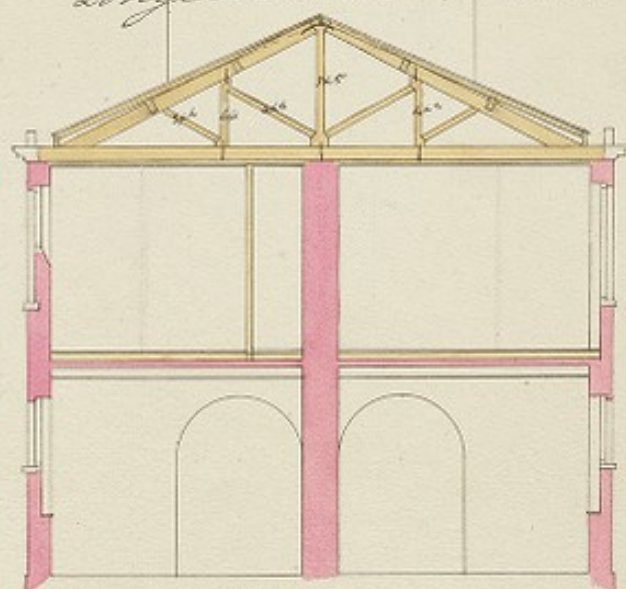
Transverse Section
