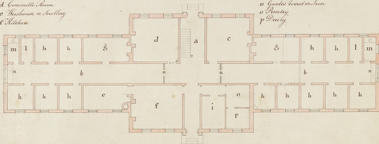
Ground story Plan
