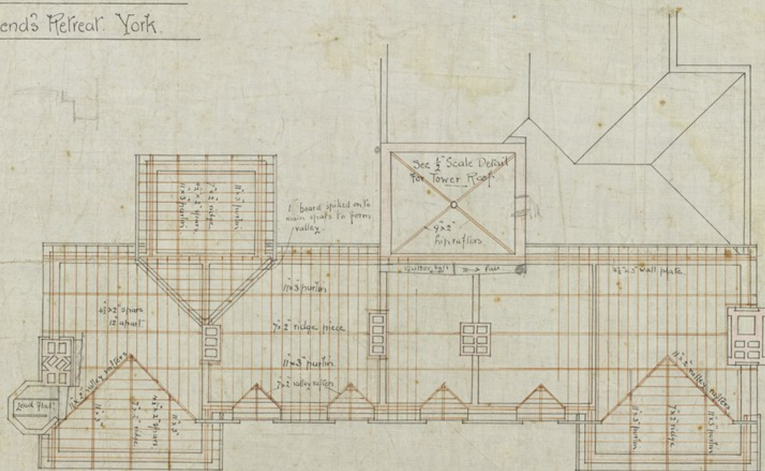
The Roof Plan. \frac{1}{8} " Scale.
