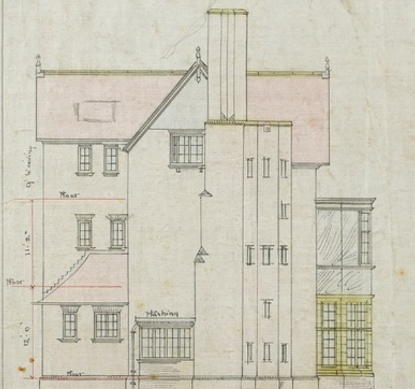
North Elevation:
