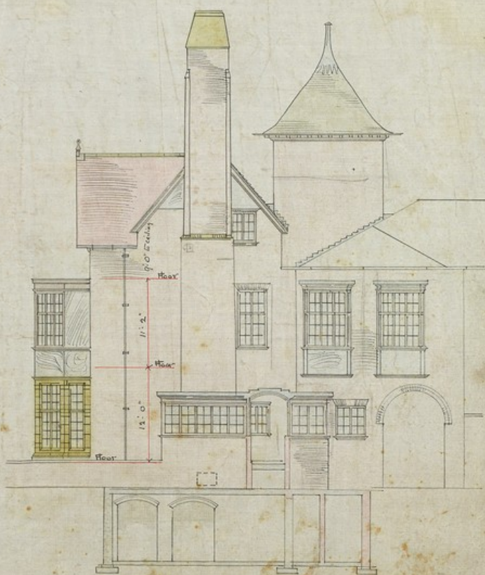
South Elevation:
