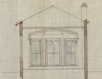
SECTION AT A.B.
