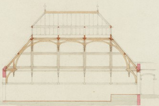
— LONGITUDINAL SECTION. — AT C.D.
