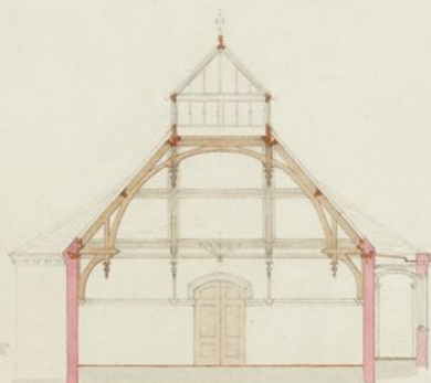
— TRANSVERSE SECTION. — AT A.B.
