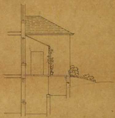
- SECTION OF VERANDAH -
