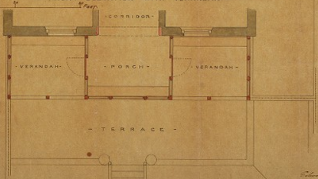
- PLAN OF PORCH AND VERANDAH -
