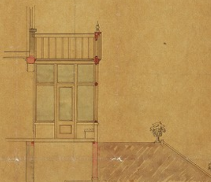
- TRANSVERSE SECTION -
