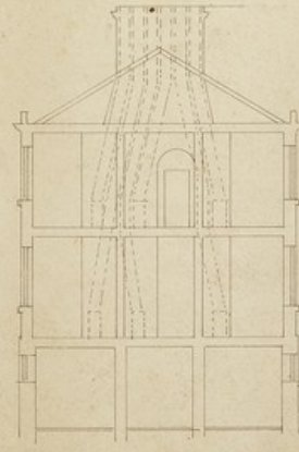
SECTION OF FLUES ON LINE M.N.
