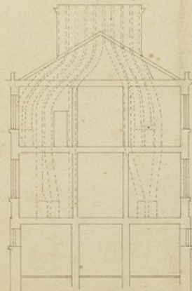
SECTION OF FLUES ON LINE K.L.
