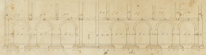
SECTION OF THE BASEMENT
