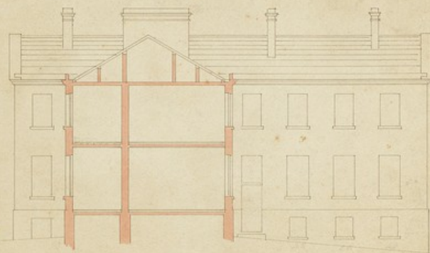
WEST ELEVATION
