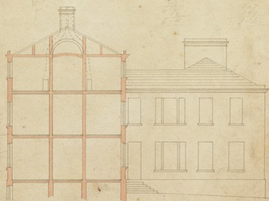
SECTION OF THE ADDITION TO MAIN BUILDING AND END ELEVATION OF NEW WING.
