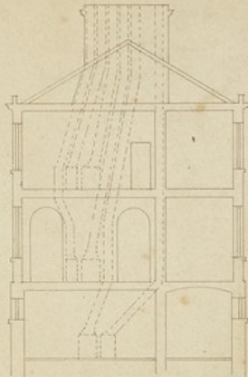
SECTION OF FLUES ON LINE C.D.
