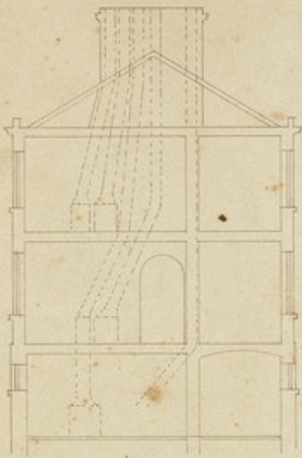
SECTION OF FLUES ON LINE A.B.
