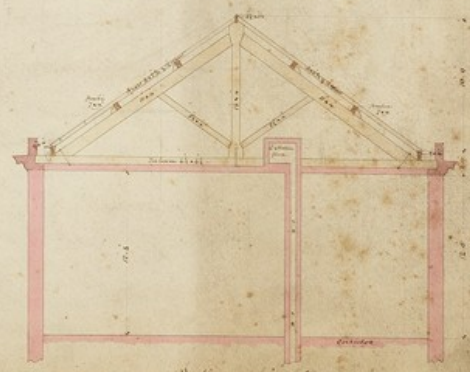
Section on line C-D
