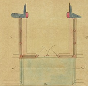
PLAN Corner Sec. 470.
