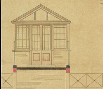
FRONT ELEVATION. SECTION W.W.
