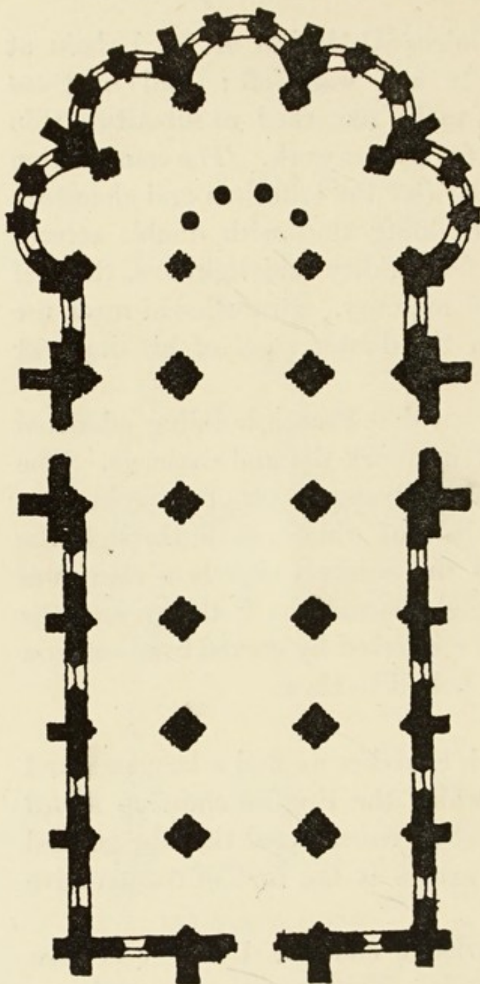
FIG. 68. Plan of church at Chars, Oise.
