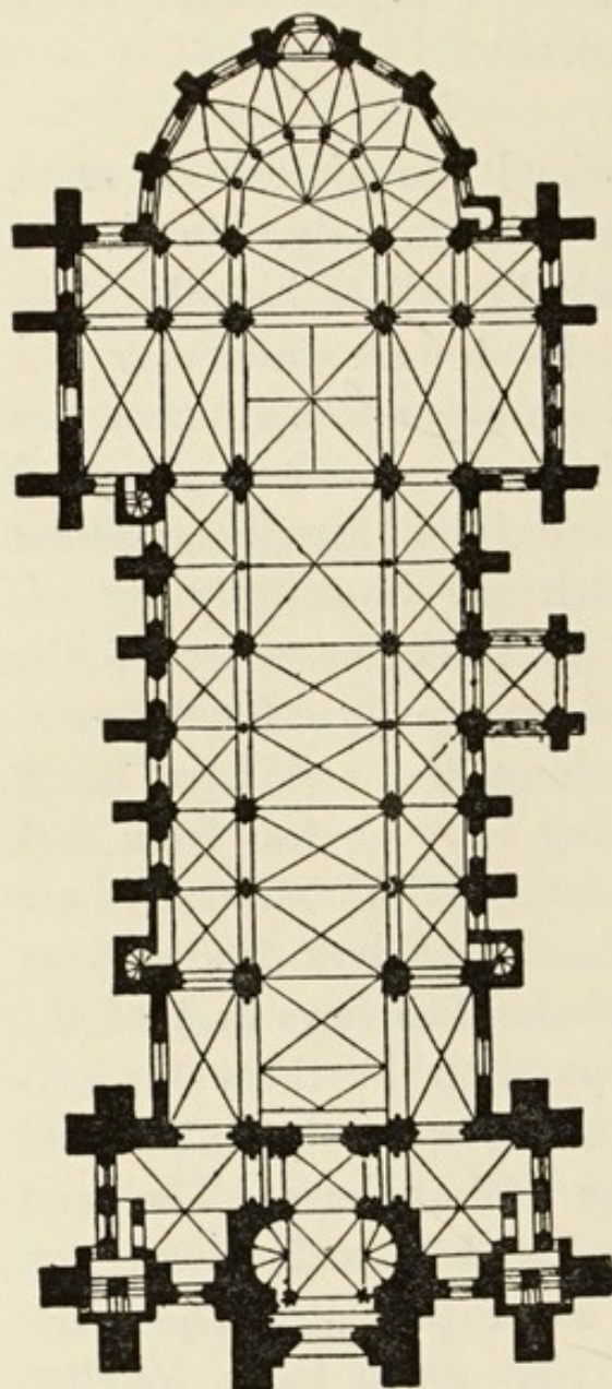
FIG. 119. Lausanne Cathedral, ground plan.
