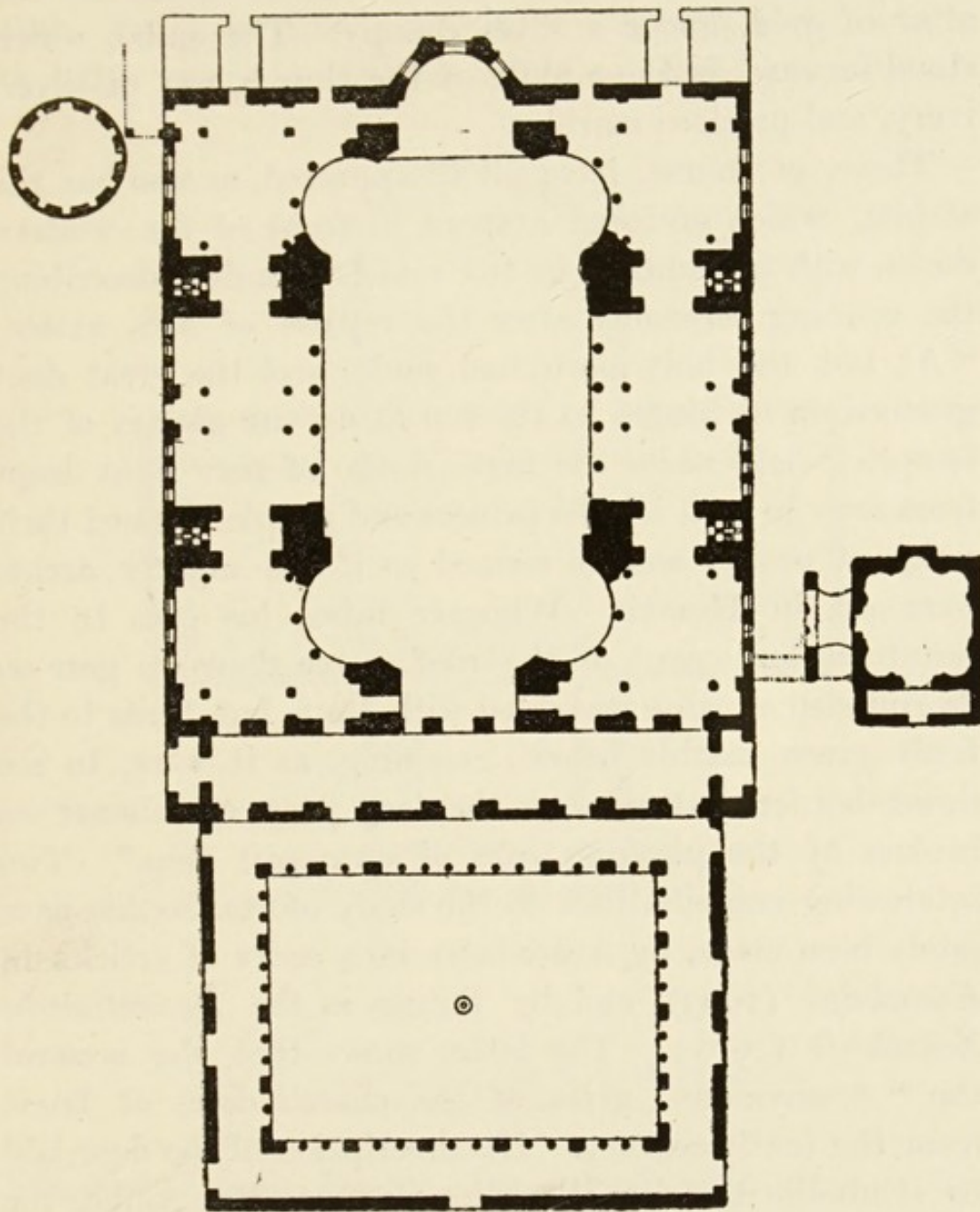
FIG. 26. Plan of Sta. Sophia, Constantinople.
