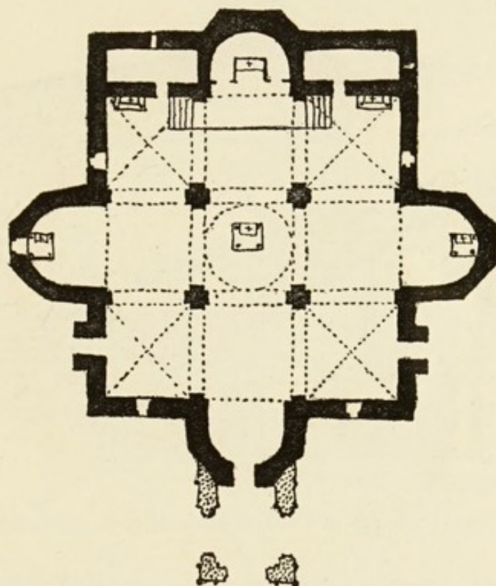
FIG. 38. Plan of the Cathedral of Etschmiadsin, Armenia.
