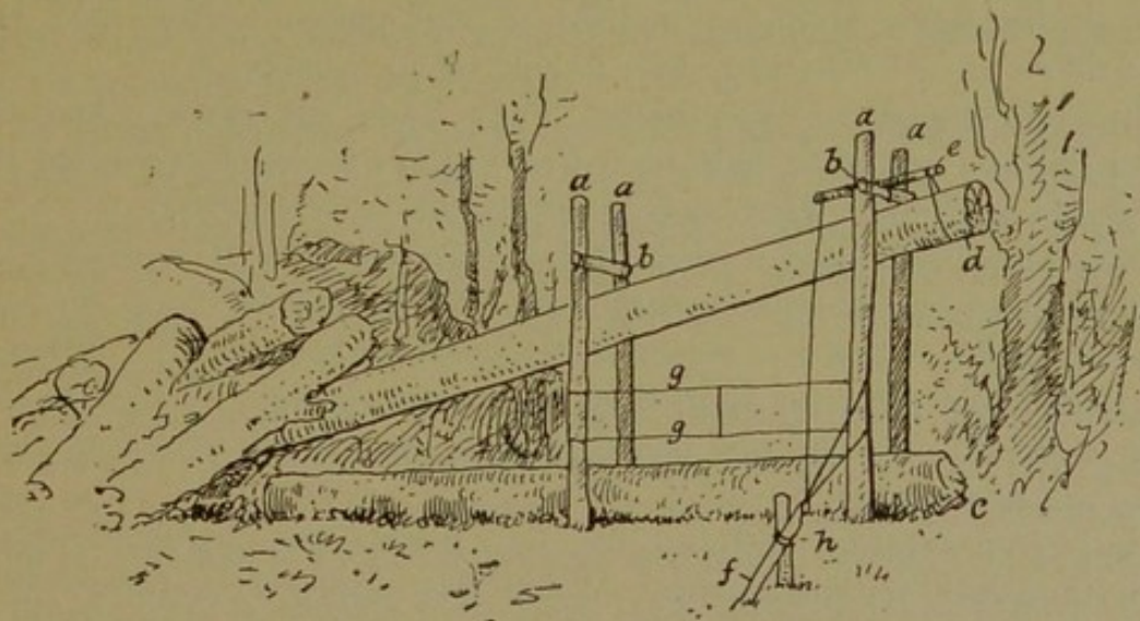
FIG. 1.—Diagram of bear deadfall.
