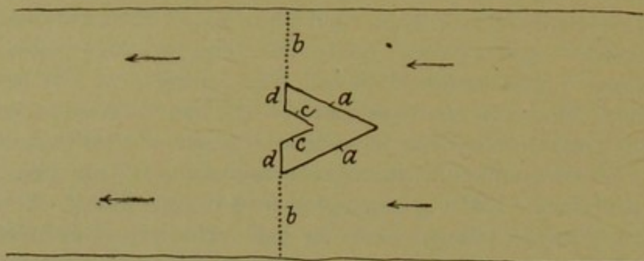
FIG. 2.—Plan of large salmon trap.
