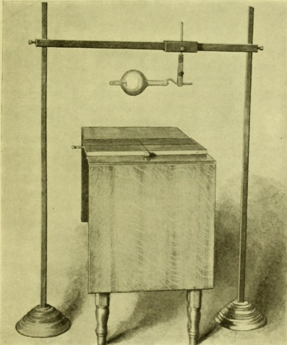
FIG. 11.—Mackenzie-Davidson exposer. The photographic plate is placed beneath the crossed wires on the board. The wires are inked and leave marks on the skin of the part and the image of the wires appears on the negative. This gives lines for localization. The tube is suspended vertically above the transverse wire and equidistant at each exposure from a point vertically above where the wires cross.
