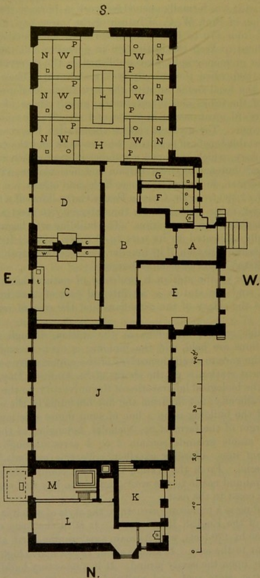
FIG. 37.—Plan of Gatty marine laboratory, St. Andrews.
