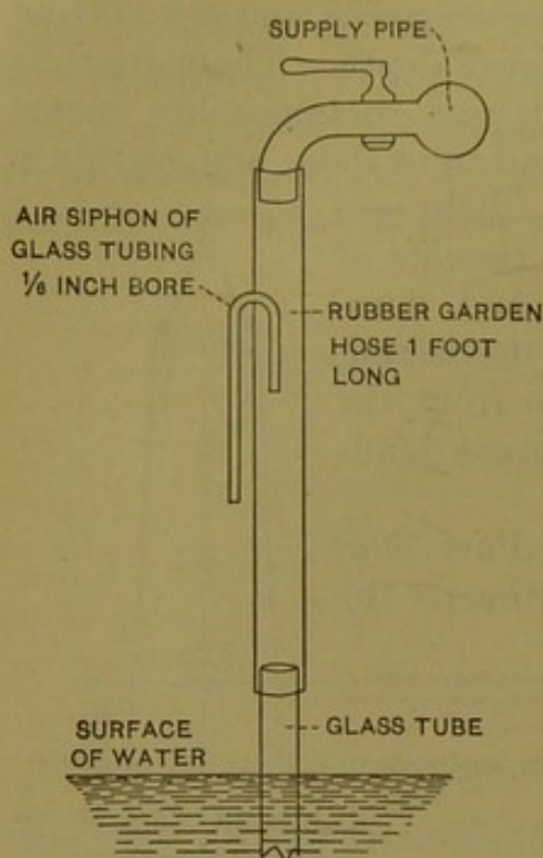
FIG. 28.—Aerating device in Port Erin aquaria.
