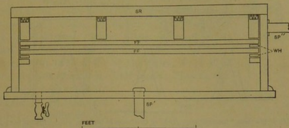
FIG. 23.—Sectional view of filter box (F, fig. 21).
