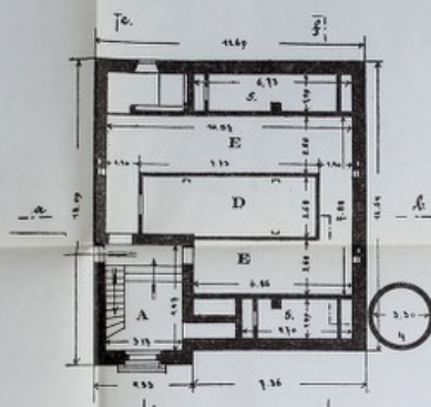
FIG. 2.—GROUND FLOOR, AT LEVEL OF FILTER BEDS.
