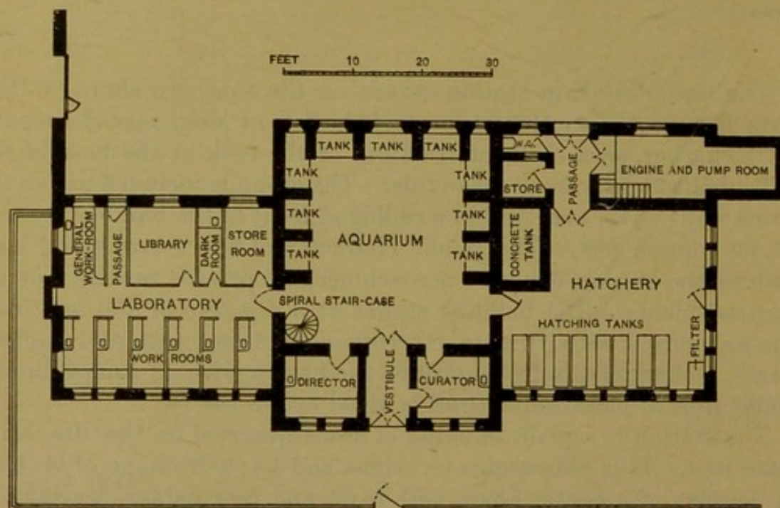
FIG. 20.—Ground floor of Port Erin biological station; after Herdman (1903).
