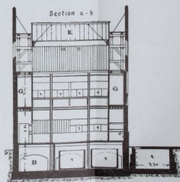
FIG. 8.—SECTION AT a-b (FIG. 2).
