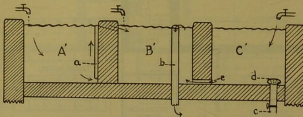
FIG. 31.—Plans of large concrete exhibition aquaria, Millport biological station. Longitudinal section through tanks A' B' C' , showing circulation and siphon ( a ), standpipe ( b ) for outflow, washout ( c ), with strainer ( d ) and bottom connection ( e ) between C' and B' .
