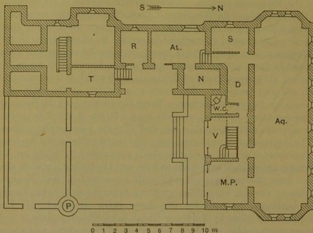
FIG. 11.—Basement floor, zoological station at Wimereux.
