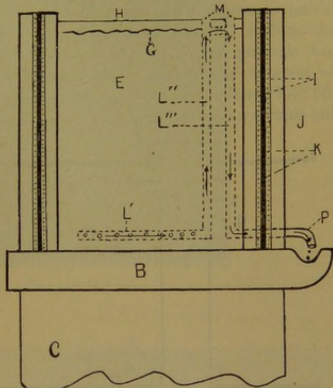
FIG. 46.—Cross section with projection of partition wall.
