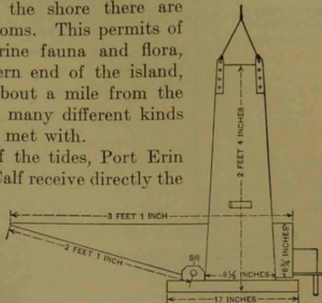
FIG. 27.—Side view of tipping box and frame.
