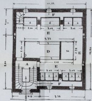
FIG. 3.—GROUND FLOOR, AT LEVEL OF EXHIBITION AQUARIA.
