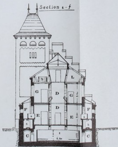
FIG. 7.—SECTION AT e-f (FIG. 1).
