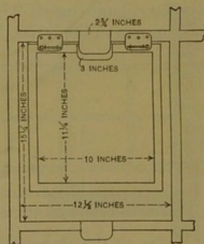
FIG. 26.—One compartment of hatching tank, with box hinged in position, seen from above.
