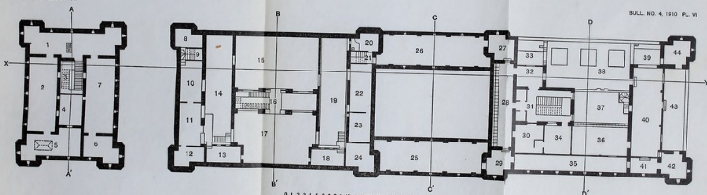
FOURTH-FLOOR PLANS, NAPLES STATION.
