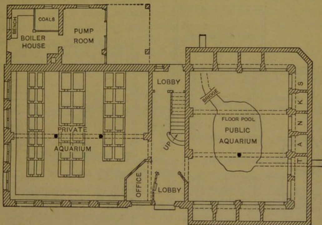
FIG. 18.—Ground floor, Dove marine laboratory. Cullercoats.
