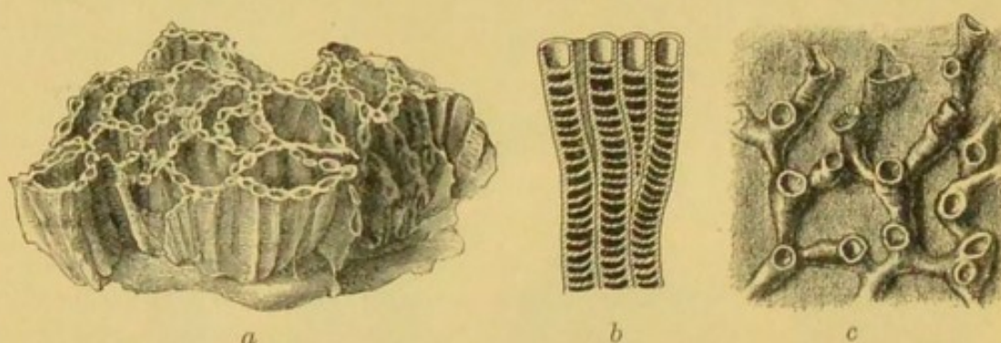
FIG. 21.—Silurian Anthozoa, possibly Alcyonaria, from the Wenlock Limestone of Dudley. a , Halysites catenularius , natural size; b , some of its tubes seen in section, to show the tabulae, slightly enlarged; c , Aulopora , growing on a shell, enlarged \frac{3}{2} diameter. (From specimen R 2067, Table-case 8.)
