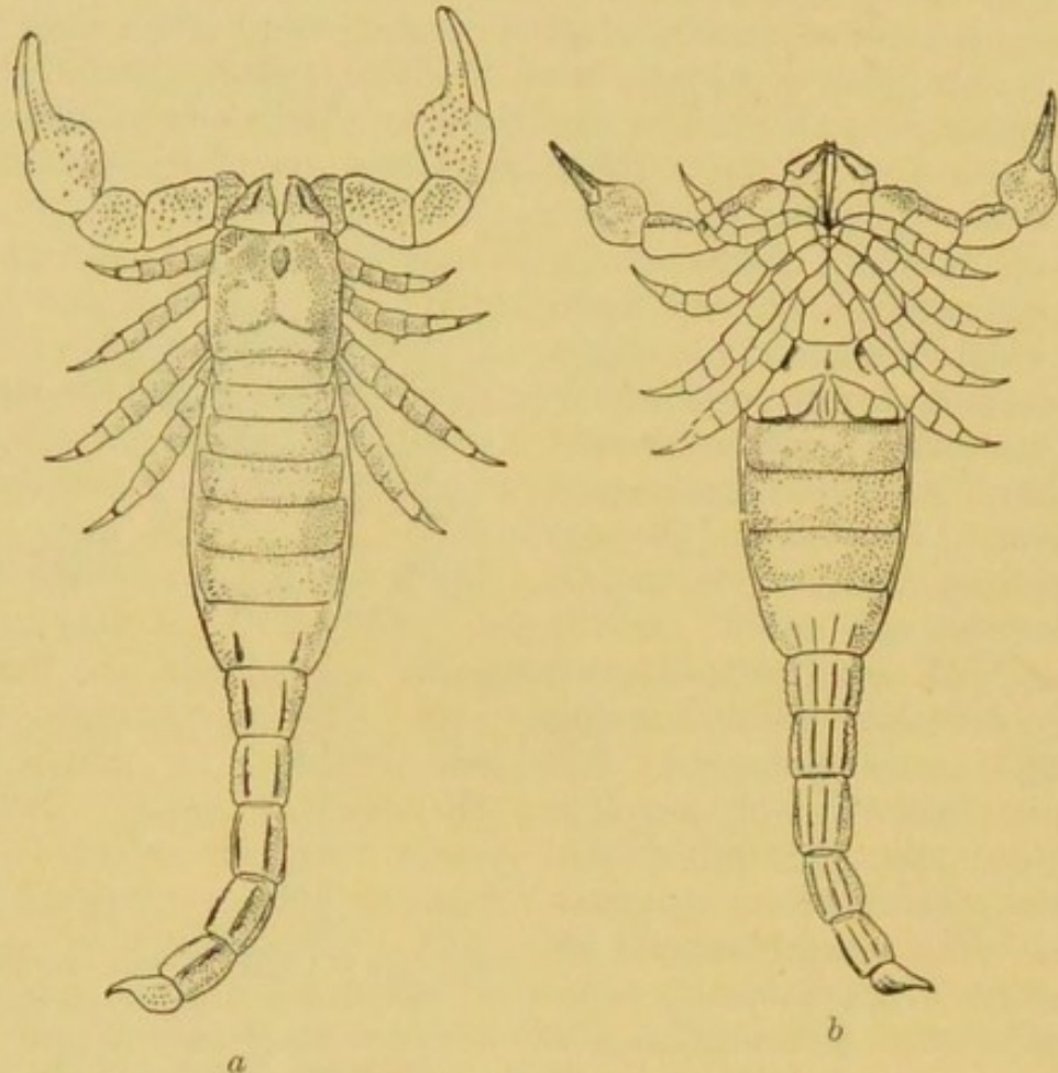
FIG. 43.—Silurian primitive Scorpions, Palæophonus . a , P. nuntius , Ludlovian of Gotland, upper surface. \frac{1}{3} nat. size. (R. I. Pocock, after Thorell & Lindström.) b , P. caledonicus [ Hunteri ], Ludlovian of Lanarkshire, under surface, about twice nat. size. (R. I. Pocock.) (Both blocks lent by Messrs. Constable, from Lankester's "Extinct Animals.")
