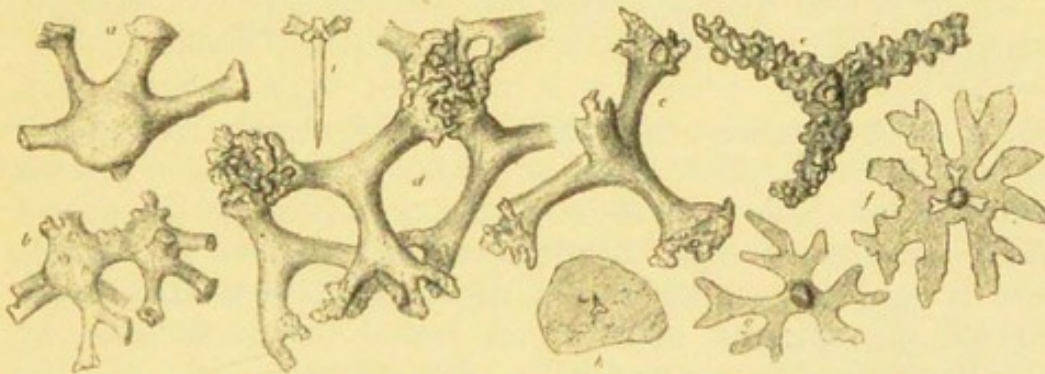
FIG. 13.—Fossil sponge spicules: Silicispongiae, Tetractinellida. Skeletal ( a – e ) and dermal ( f – i ) spicules of Lithistida. Eutaxi cladina: a , Mastusia . Anomocladina: b , Cylindrophyma . Tetracladina: c , d , Callopegma ; e , Plinthosella . e , enlarged 26 diam.; the rest 40 diam. (After Hinde.)
