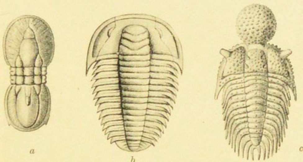
FIG. 40.—Examples of Trilobites. a , Hypoparia, Agnostus princeps , Olenidian Age; enlarged 2\frac{1}{2} times. b , Opisthoparia, Olenus cataractes , Olenidian Age. c , Proparia, Staurocephalus Murchisoni , Wenlockian Age.
