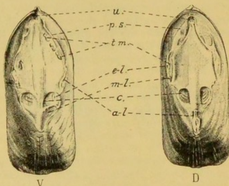
FIG. 57.—The muscle-scars of the Recent Lingula anatina . Interior of V, ventral or peduncular valve, and D, dorsal or brachial valve. u , umbonal; p.s. , parietal; tm , transmedian; e-l , externo-lateral; m-l , medio-lateral; c , central; a-l , antero-lateral.
