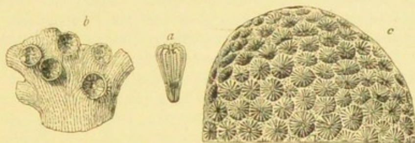
FIG. 27.—Perforate Zoantharian corals from the Lutetian of Bracklesham. a, Turbinolia Dixoni ; b, Dendrophyllia dendrophyllodes ; c, Goniopora Websteri . Natural size. (From Prestwich's "Geology.") (See Table-case 1.)
