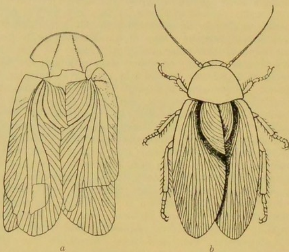
FIG. 52.—Cockroaches of the Coal Measures. a , Etoblattina mazona from Illinois, enlarged 2 diameters. (After Seudder.) b , restoration of Progonoblattina helvetica from Switzerland. Natural size. (After Heer.)
