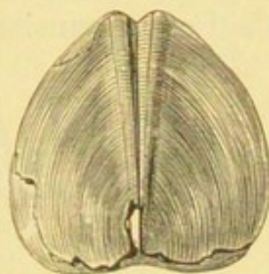
FIG. 83.—Aptychus of an ammonite.
