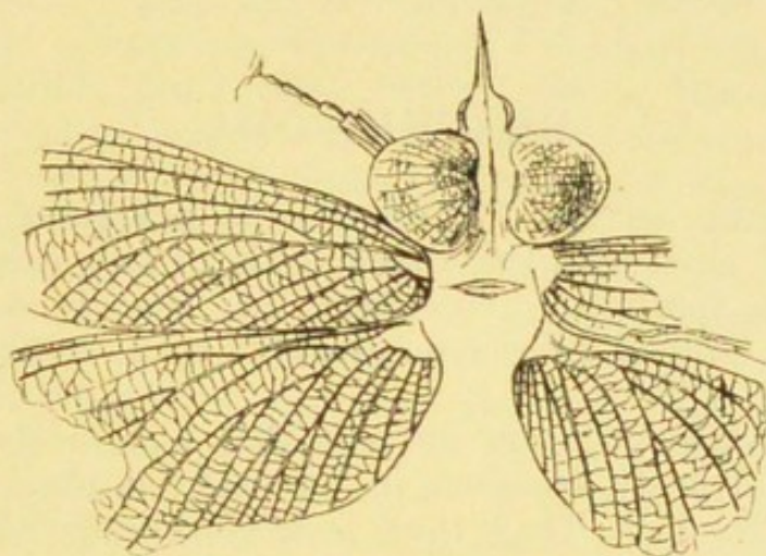
FIG. 54.—An Insect from the Coal Measures of Ayrshire, Lithomantis carbonarius , probably a Neuropteran. \frac{3}{4} natural size. (After H. Woodward.) (Table-case 20.)
