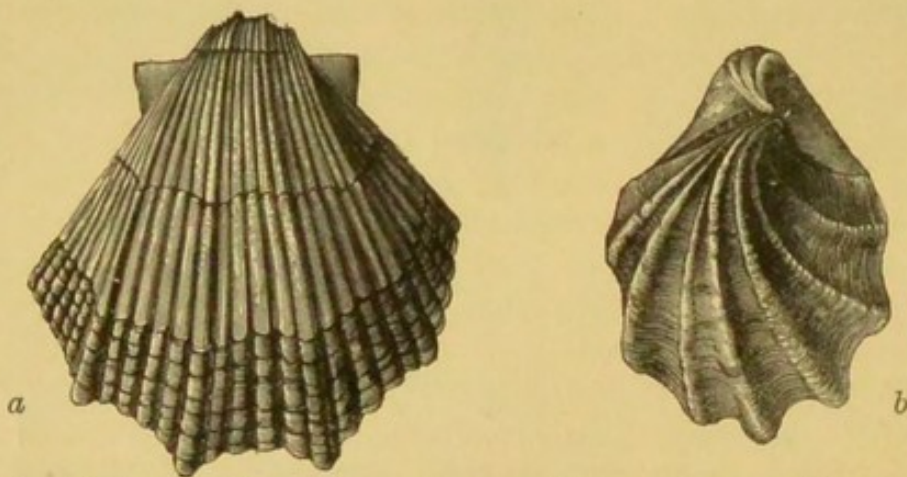
FIG. 71.—Cretaceous Lamellibranchs. a , Neithea quinquecostata , common in Senonian Chalk; b , Actinoceras sulcatus , from the Gault. Natural size.
