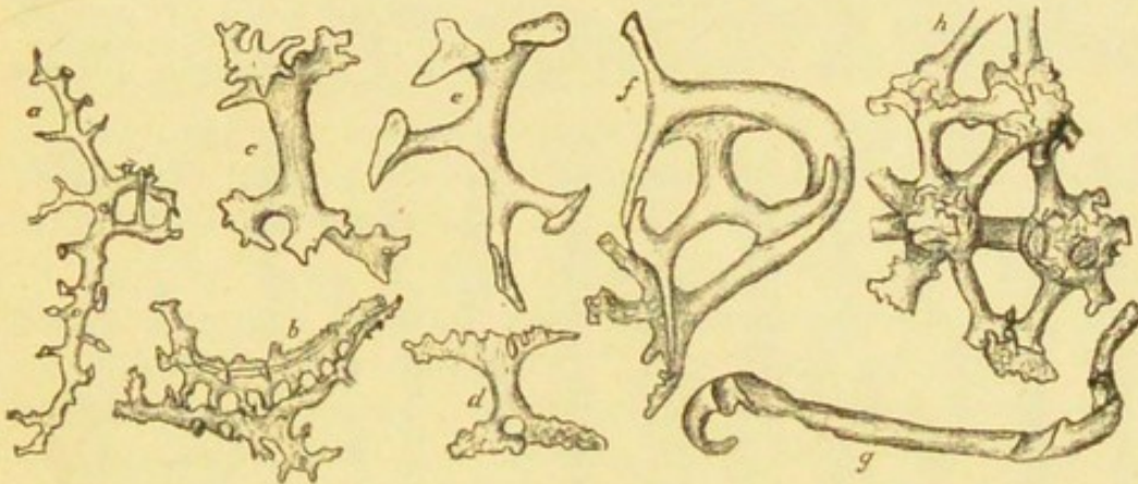
FIG. 12.—Fossil sponge spicules: Silicispongiae, Tetractinellida. Skeletal spicules of Lithistida. Rhizomorina: a , b , Seliscothon ; c , Cnemidiastrum . Tetracladina: d , Aulocopium megamorina ; e , f , Doryderma ; g , Carterella . Eutaxi cladina: h , Astylospongia . a , b , c , d , h , enlarged 40 diam.; e , 26 diam.; f , g , 20 diam. (After Hinde.)
