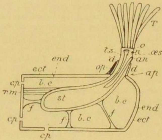
FIG. 61.—Diagram of structure of a typical Bryozoan zooid, as seen in a vertical cut down the middle. an , anus; ap , aperture; b.c , body-cavity; c.p , communication pore; d , diaphragm; ect , ectocyst; end , endocyst; f , funiculi; n , nerve-ganglion; o , orifice; æs , cesophagus; op , operculum; r.m , retractor muscle; st , stomach; T , tentacles; t.s , tentacle sheath.
