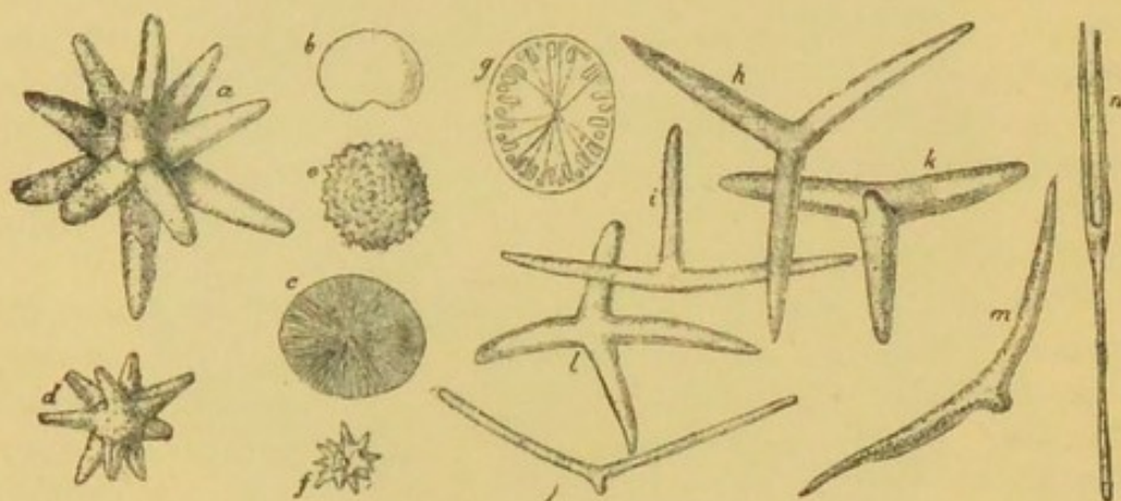
FIG. 8.—Fossil sponge spicules: Silicispongiae, Heteractinellida, skeletal spicule (a); Silicispongiae, Tetractinellida and others, flesh spicules (b-g); Calcispongiae, skeletal spicules (h-n). a is from Asteractinella ; b, c from Geodia ; j-l from Tremacystia . a is enlarged 13 diam.; b-g, 66 diam.; h, 26 diam. i, 114 diam.; j, m, n, 134 diam.; k, l, 80 diam. (After Hinde.)
