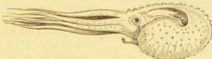
FIG. 87.—Female Argonaut swimming from left to right.
