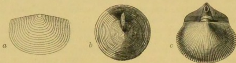
FIG. 58.—Types of Brachiopod Orders. a , Order Atremata, the Cambrian Iphidea labradorica , one of the simplest forms of brachiopod shell. b , Order Neotremata, the Ordovician Orbiculoidea lamellosa , the peduncular valve, showing the delthyrium, which has become surrounded by the valve and partly filled in from underneath by a shelly deposit. c , Order Protremata, the Ordovician Clitambonites Verneuili , seen from the side of the brachial valve, above which is the lofty hinge-area of the peduncle valve. The delthyrium is covered by a single pseudodeltidium, through which the peduncle passed by the foramen.
