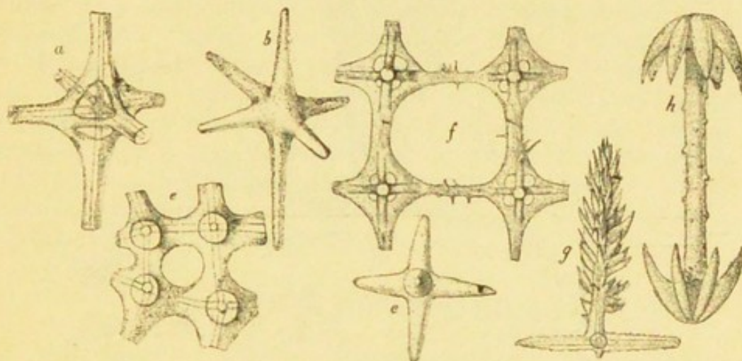
FIG. 9.—Fossil sponge spicules: Silicispongiae, Hexactinellida. a-f are skeletal spicules; g, h are flesh spicules. Six-rayed spicules are shown in a, b, e, f ; in c one ray is suppressed. Axial canals are seen in a, c and f , and a and f have lantern nodes. e and f illustrate the union of spicules to form the square mesh of Dictyonina, e being from Sestrodiction and f from Coeloptychium ; g is called a pinule, and h an amphidisc. a is enlarged 66 diam.; b, c, f , 40 diam.; e , 47 diam.; g , 134 diam.; h , 114 diam. (After Hinde.)
