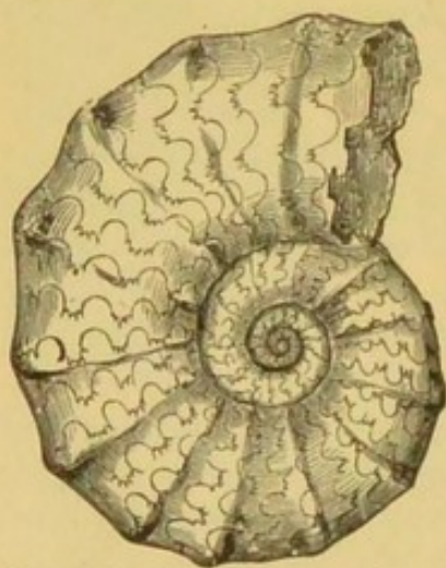
FIG. 94.— Ceratites nodosus from the Muschelkalk.
