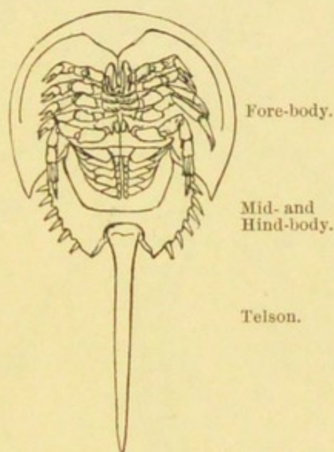
FIG. 42.—Under surface modern Xiphosura, Limulus polyphemus , the King-crab. About \frac{1}{10} th the diameter of the real animal.
