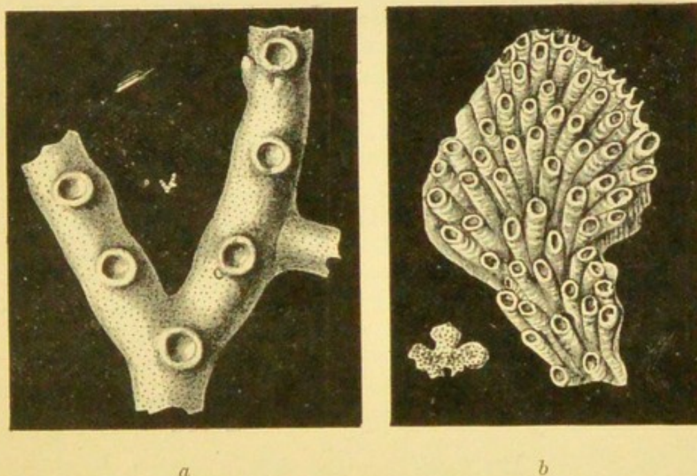
FIG. 64.—Cyclostomatous Bryozoa from the Bathonian (Bradford Clay) of England. a , Stomatopora dichotoma , part of an encrusting colony, natural size, and magnified 25 diameters. b , Berenicea compressa , an encrusting colony, natural size, and part of it magnified 12 diameters. (After J. W. Gregory.)
