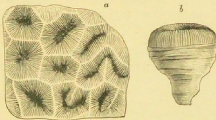
FIG. 24.—Zoantharian Corals of Bajocian Age, from the Inferior Oolite of England. a , " Latomaandraea " Flemingi. b , Montlivaltia trochoides . (From Prestwich's "Geology.")
