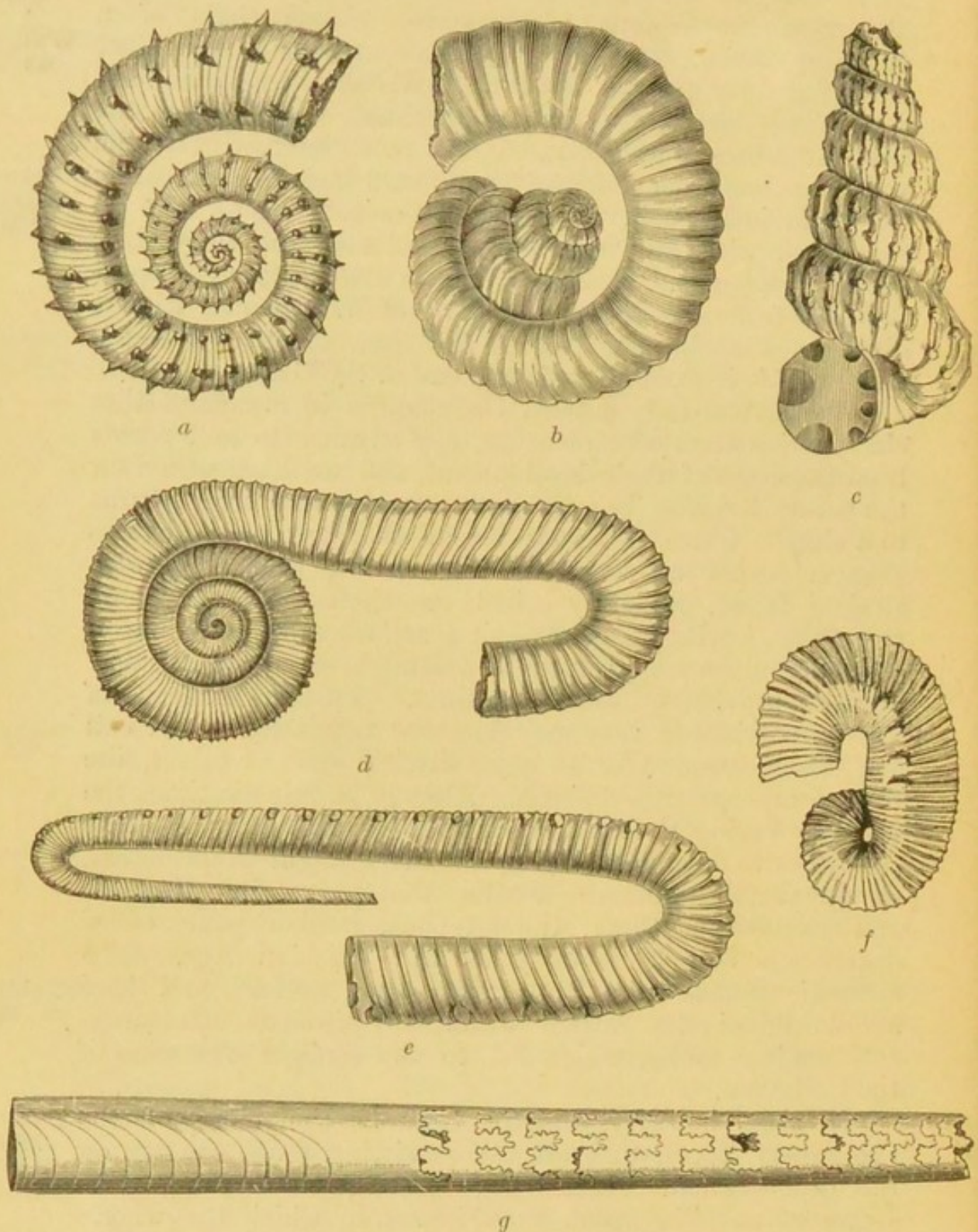
FIG. 96.—Uncoiled and Asymmetric Cretaceous Ammonoidea. a , Crioceras Emerici , Neocomian. b , Heteroceras Emericianum , Neocomian. c , Turrilites catenatus , Albian. d , Macroscaphites Ivanii , Neocomian. e , Hamites elegans , Albian. f , Scaphites Hugardianus , Albian. g , Baculites anceps , Danian. All less than natural size.
