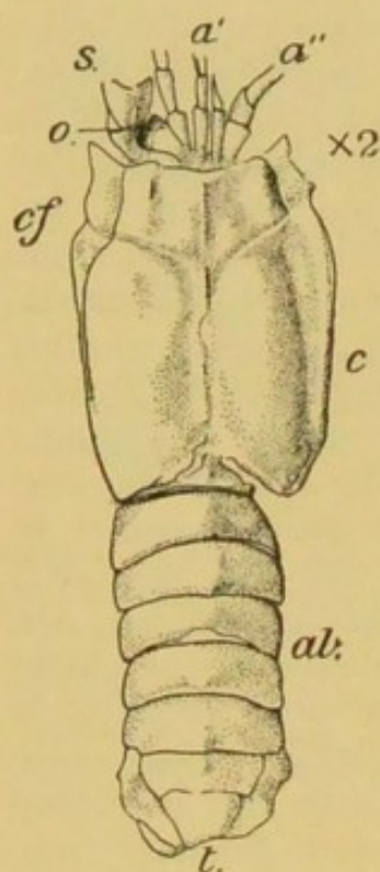
FIG. 47. — Anthrapalaemon Woodwardi , Lower Coal Measures, Lancashire. a' , antennule; a'' , antenna; o , stalked eye; cf , furrow separating head-shield from carapace, c ; ab , abdomen; t , telson. Enlarged 2 diam. (From H. Woodward, "Geol. Mag.," 1905.)
