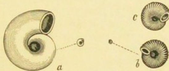
FIG. 36.—Supposed coiled tubes of Polychæta, from the Devonian of Canada. a , Spirorbis omphalodes ; b and c , Spirorbis arkonensis . The smaller drawings give the natural size of the objects (after Nicholson).
