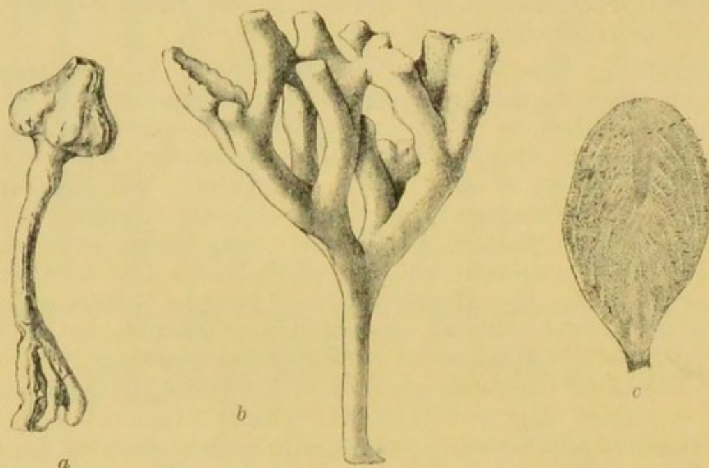
FIG. 16.—Lithistid sponges from the Upper Greensand of Warminster. a , Hallirhoa costata (specimen 48174); b , Doryderma dichotomum (specimen P 1260); c , Siphonia tulipa ; a a section through the upper part of the sponge, showing the cloaca in the middle near the top, the large excurrent canals which open into it, and the fine incurrent canals leading from the outside to these latter (specimen P 1366). a and b are reduced to \frac{1}{4} nat. size, and c to \frac{1}{2} . (After Hinde. See Table-case 13.)
