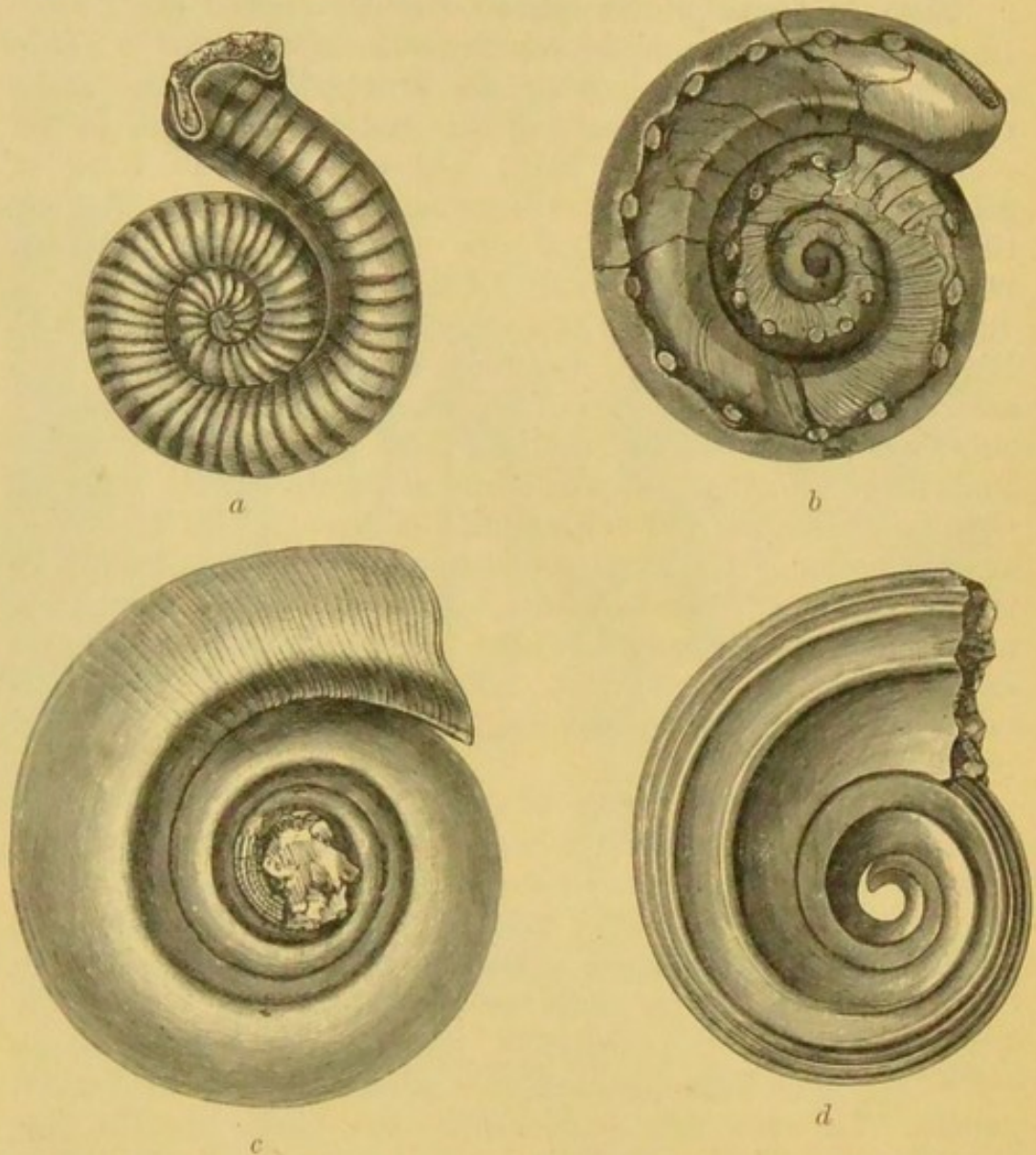
FIG. 92.—Palaeozoic Nautiloidea. a , Ophidioceras simplex , Silurian, Bohemia. b , Hercoceras mirum , Devonian, Bohemia. c , Apheloceras mutabile , and d , Vestinautilus multicarinatus , Carboniferous Limestone, Ireland. All slightly less than natural size. (From Foord.)
