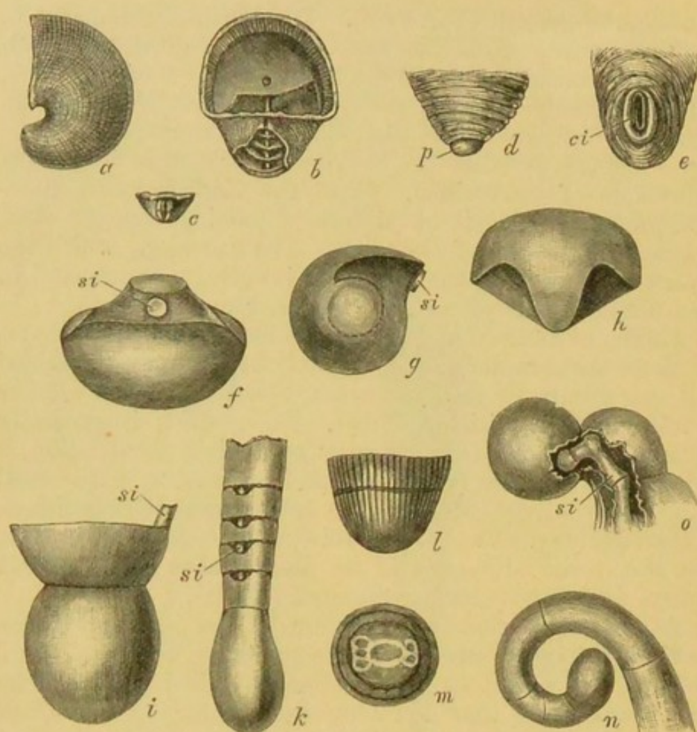
FIG. 81.—The first-formed portions of various chambered Cephalopod shells. a, b, c , Nautilus pompilius : a , side view; b , front view, the apex broken to show siphuncle passing through septa; c , apex, showing scar left by protoconch. d , a straight shell of Triassic age, with a plug ( p ) at its apex. e , a curved Carboniferous nautiloid, Meloceras , with scar ( ci ). f, g, h , front, side, and upper views of protoconch of an ammonite, Cosmoceras . i , Protoconch and first chamber of a belemnite. k , Protoconch and five chambers of Bactrites , the shell partly removed, showing siphuncle. l, m , the first two chambers of an allied form from which the protoconch has disappeared, leaving a cicatrix, shown in m . n , Protoconch and first five chambers of Mimoceras compressum , a goniatite. o , Protoconch and part of two chambers of Spirula , the shell-wall partly broken away. In g, i, k, o , the siphuncle is denoted by si . c is natural size, the rest greatly enlarged. (From Foord & Crick. After Barrande, Hyatt, & Branco.)
