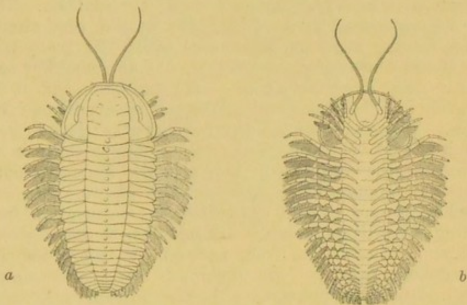
FIG. 39.—Reconstruction of a Trilobite, Triarthrus Becki , from the Ordovician, Utica Slate of New York; a, upper side; b, under side; slightly enlarged. (After Beecher. Table-case 25.)
