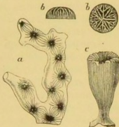
FIG. 26. — Zoantharian corals from the British Chalk. a and c are Madreporaria Aporosa : a , Synhelix Sharpei ; c , Parasmilia centralis . b is a Perforate Madreporarian , Stephanophyllia Bowerbanki . Nat. size. (From Prestwich's "Geology.") (See Table-case 1.)
