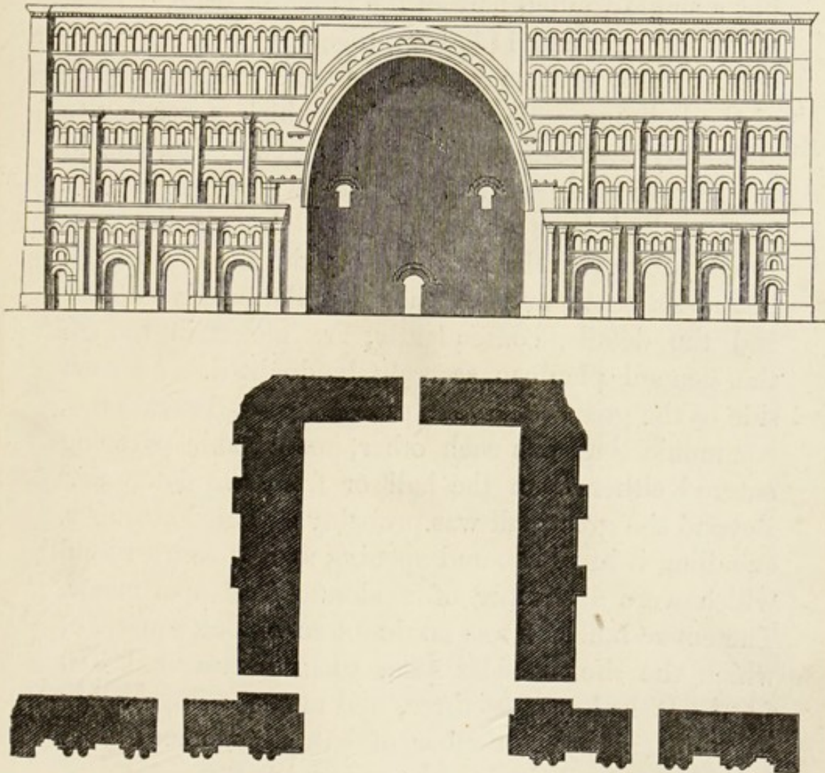
ELEVATION AND GROUND PLAN OF THE PALACE AT CTESIPHON (after Flandin). Scale, 1 inch to 100 feet.
