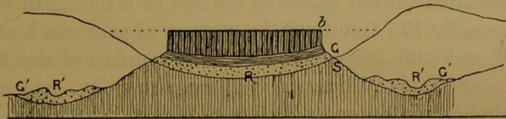
SECTION ACROSS TABLE MOUNTAIN, TUOLUMNE COUNTY, CALIFORNIA.
