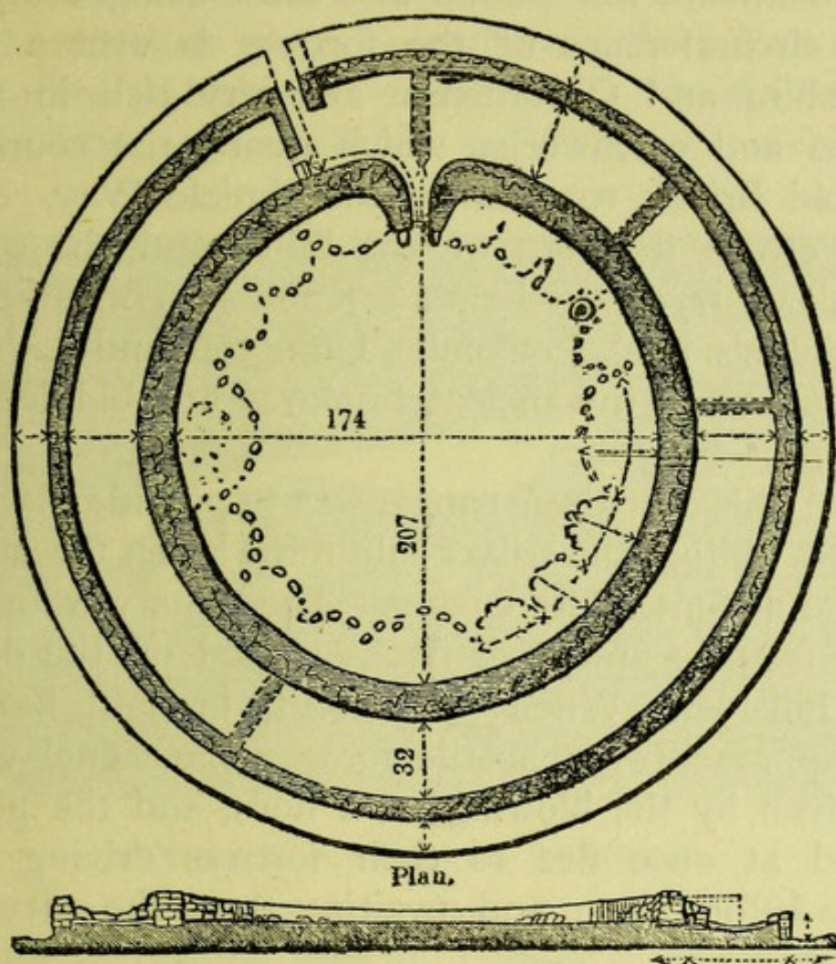
PLAN AND SECTION OF CHUN CASTLE
