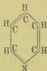
Pyridin
