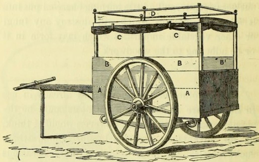
Ambulance.—A. Dotted line showing the position of seat. B B. Wooden flap on hinges, which can be put up or down as required. C. Canvas curtains. D. Iron railings for the protection of baggage.
