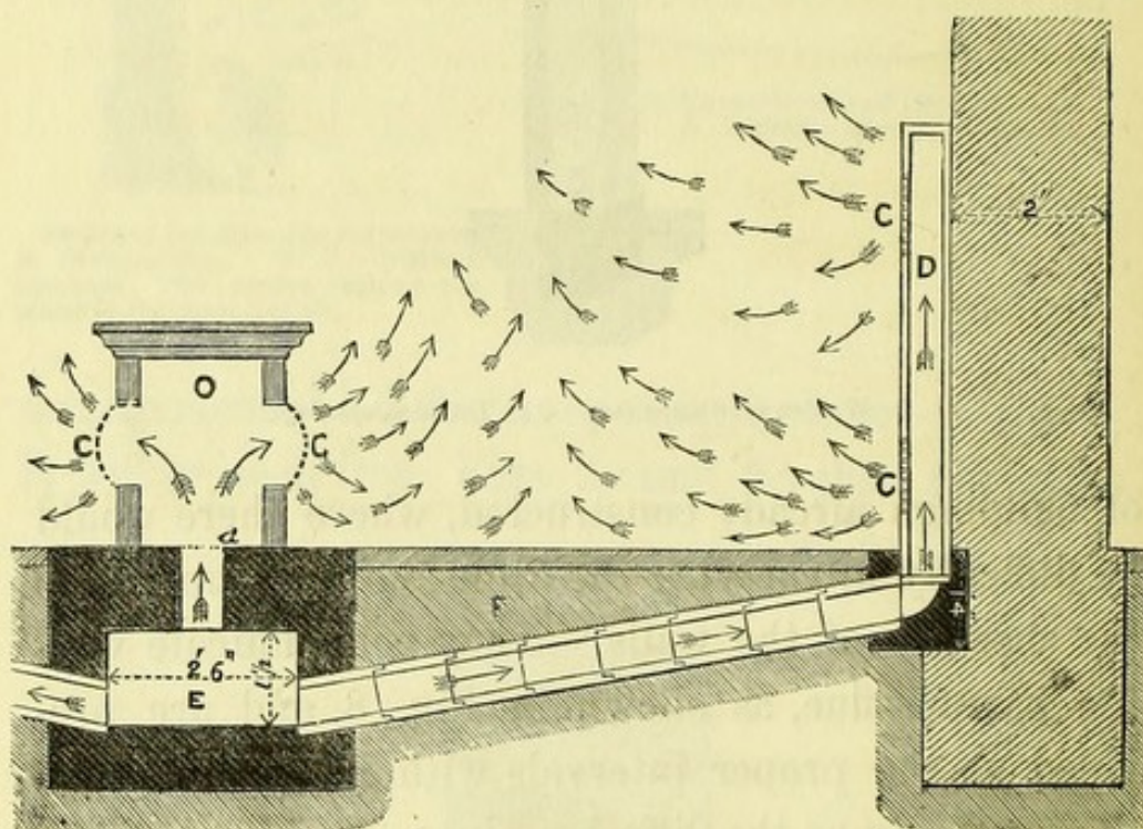
Sectional view of ventilating diffusion-apparatus, showing course of currents of air. C C. Exit-openings, covered with perforated metal. D. Ventilating case. E. Section of barrack. F. Diffusion-pipe. O. Section of central diffusion-case. a . Trap-door valve..
