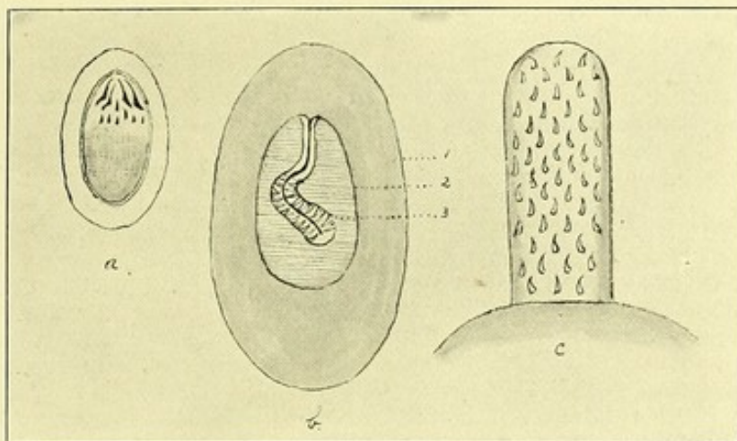
Development of Gigantorynchus moniliformis .
