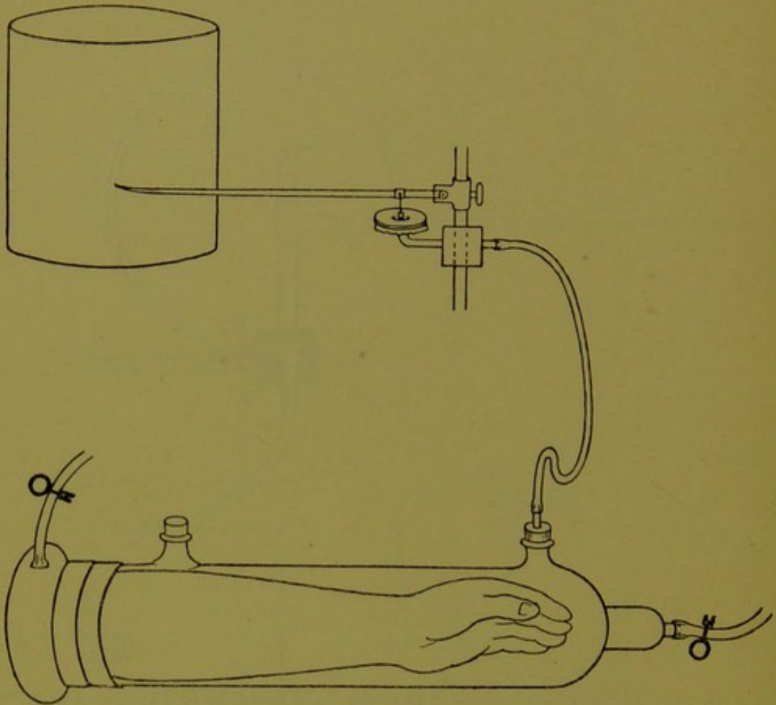
FIG. 67.—MOSSO'S ARM-PLETHYSMOGRAPH.
