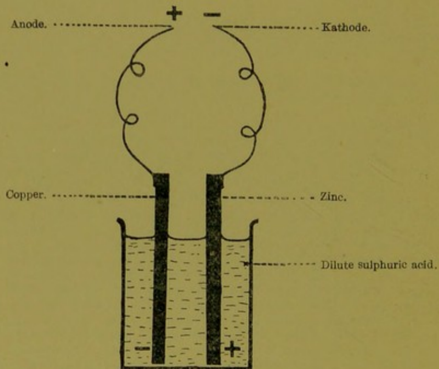
FIG. 1.—VOLTAIC COUPLE.
