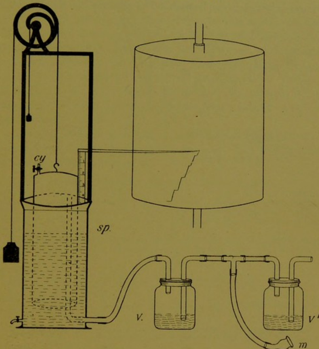
FIG. 75.—SPIROMETER ARRANGED TO REGISTER, UPON A SLOWLY REVOLVING DRUM, THE AMOUNT OF AIR RESPIRED. sp. , BODY OF SPIROMETER; cy , MEASURING CYLINDER WITH SCALE AND WRITER ATTACHED; v. , v' ., WATER VALVES; m , MOUTHPIECE.
