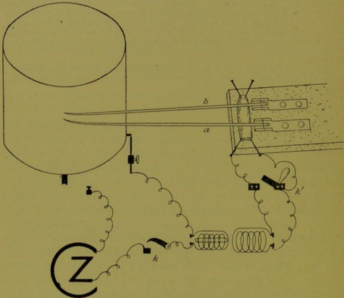
FIG. 35.—DIAGRAM OF AEBY'S EXPERIMENT FOR RECORDING THE MUSCLE WAVE. a , b , LIGHT STRAW LEVERS RESTING ON THE MUSCLE, WHICH IS CURARIZED; k , k' , KEYS IN PRIMARY AND SECONDARY CIRCUITS.
