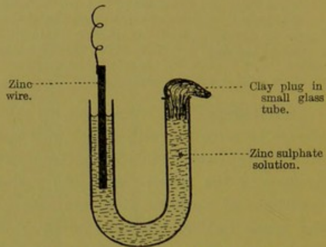
FIG. 8.—SANDERSON'S PATTERN OF NON-POLARISABLE ELECTRODE.
