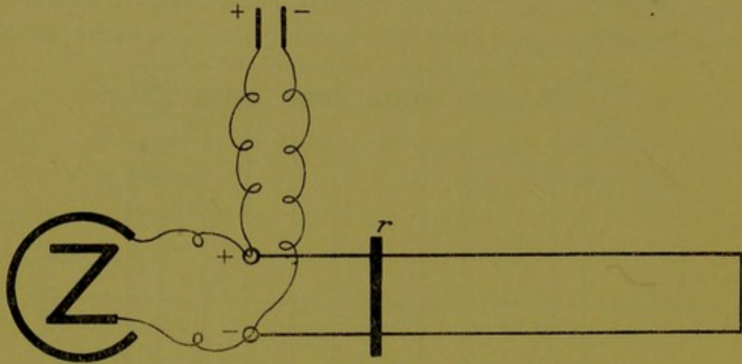
FIG. 21.—DOUBLE-WIRE RHEOCHORD.
