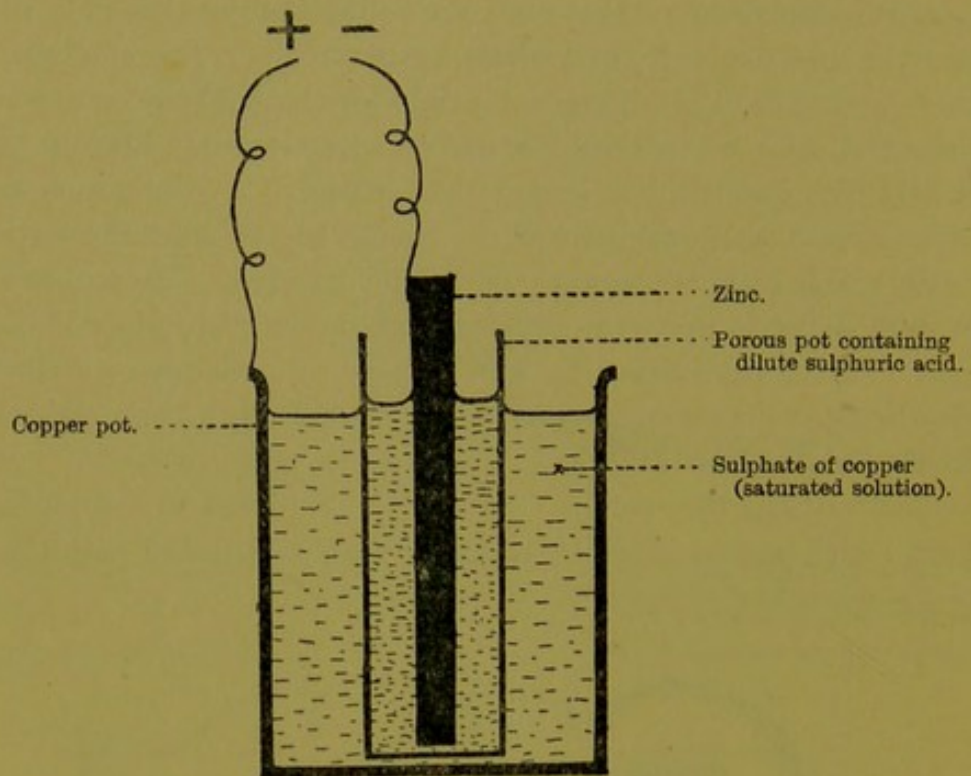
FIG. 3.—DANIELL CELL.
