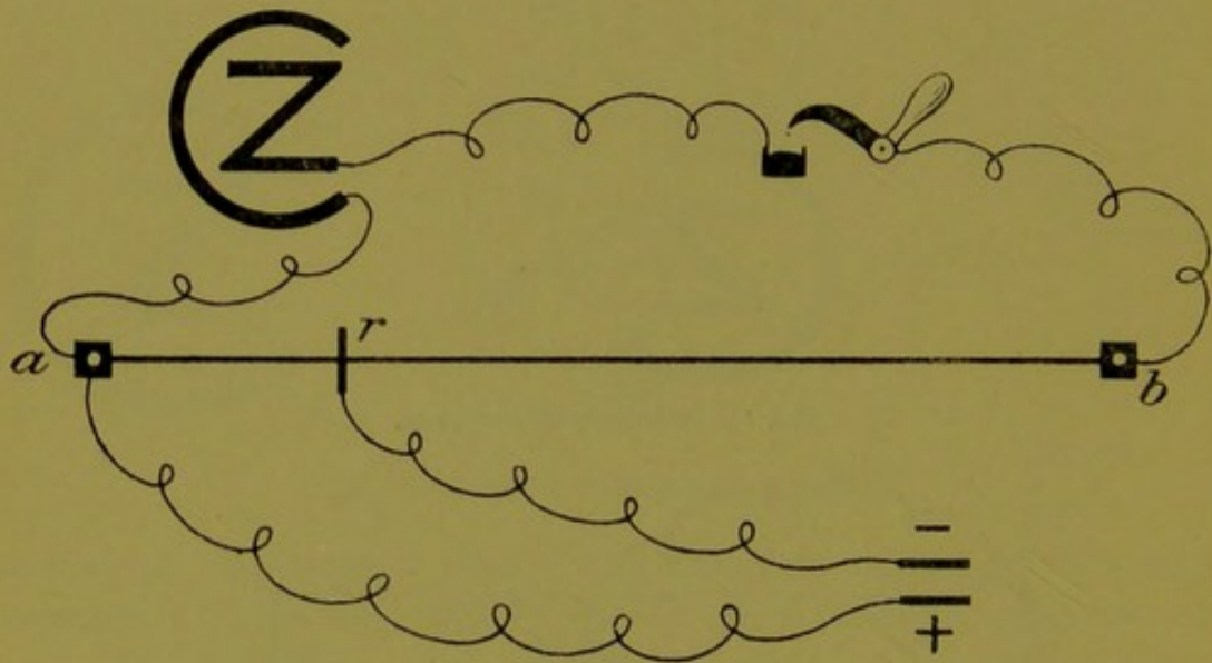
FIG. 19.—DIAGRAM OF RHEOCHORD.
