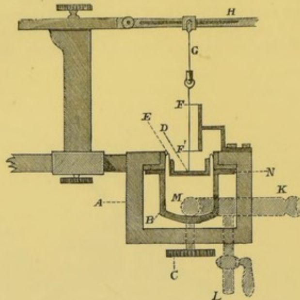
FIG. 89. SEMI-DIAGRAMMATIC SECTIONAL VIEW OF ONCOGRAPH. Half natural size. K tube connecting instrument with oncometer. D piston floating on oil contained in the cavity M ; the oil is prevented from escaping by the side of the piston by the delicate flexible membrane E , which does not interfere with the movements of the piston. H , recording lever connected with the piston by a needle G passing through the guides F , F' . The screw C is for the purpose of clamping the edge of the membrane between the two ring-shaped surfaces at N , while the side tube L is for the purpose of filling the instrument.
