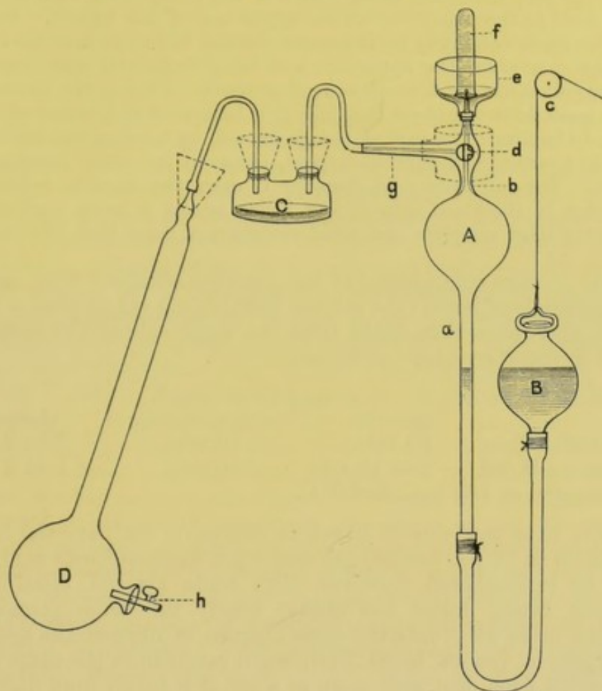
FIG. 74. DIAGRAM OF ALVERGNIAT'S PUMP.
