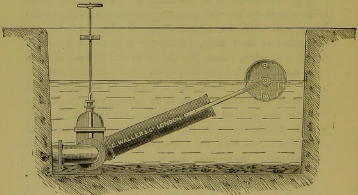
Fig. 3.—Waller's valves.
