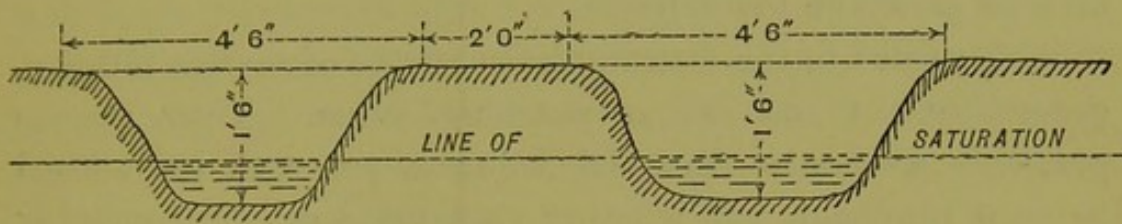
Fig. 12.—Ridge and furrow filtration areas.
