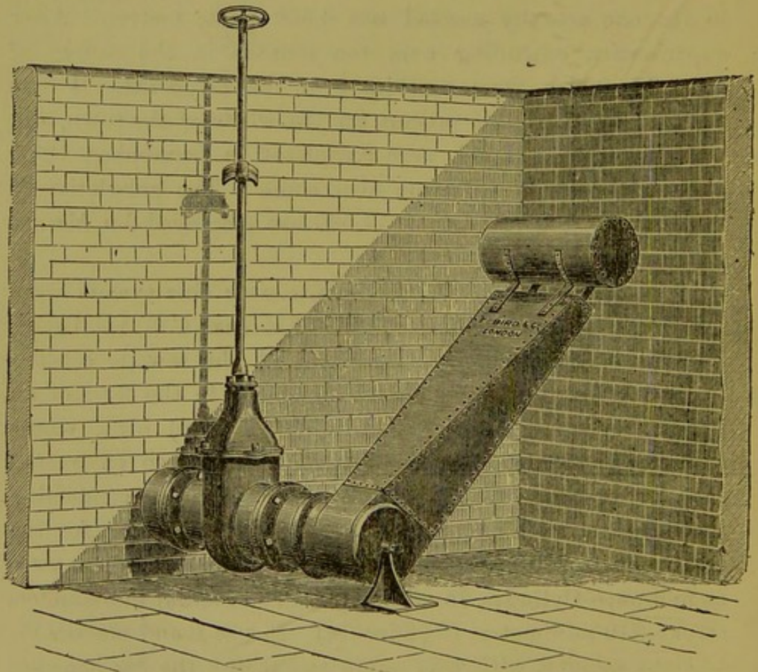
Fig. 4.—Floating arm used in settling tanks.
