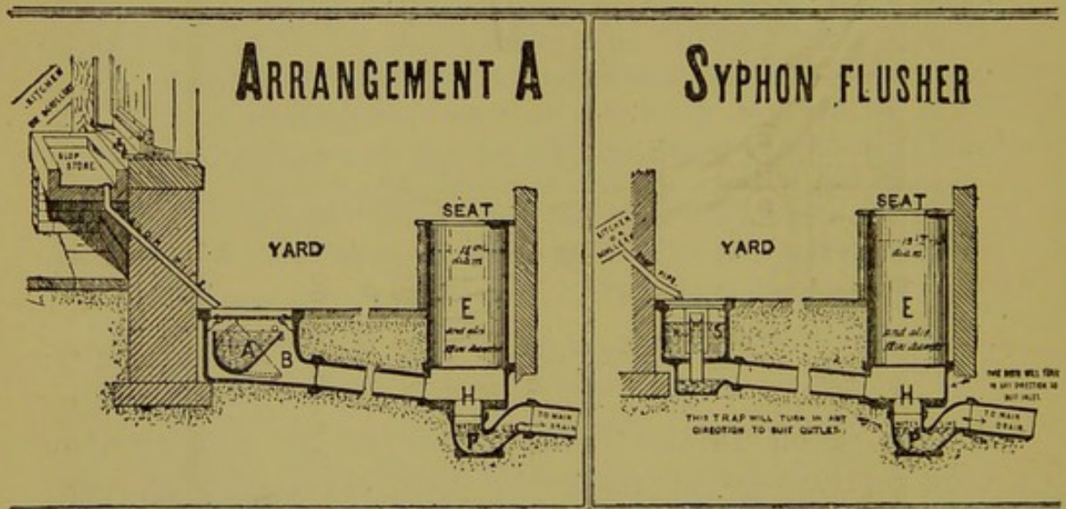
Fig. 1.—Duckett's Closet.
