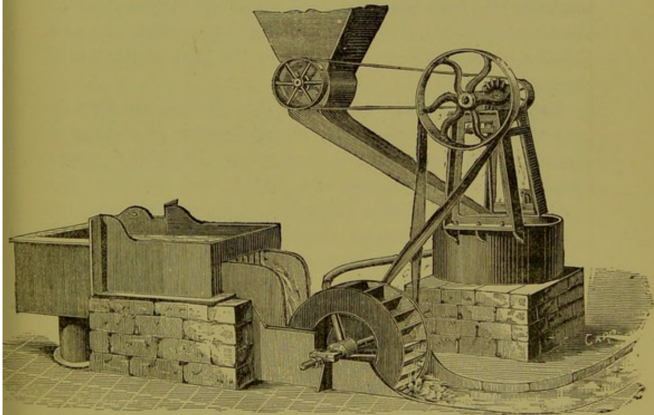
Fig. 6.—Bradley's sewage clarifier.
