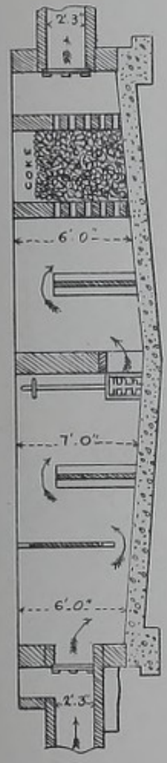
SECTION OF STRAINING TANK
