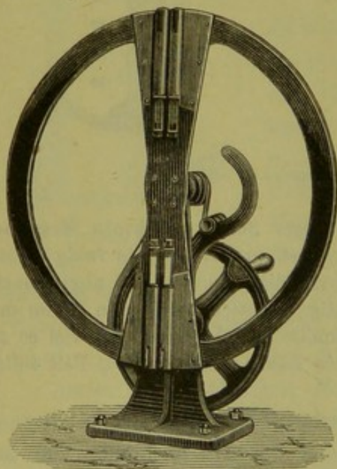
Lefeldt's Centrifugal-Milchprober.
