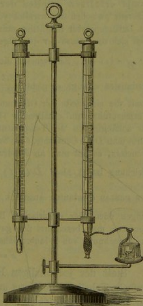
August's Psychrometer.
