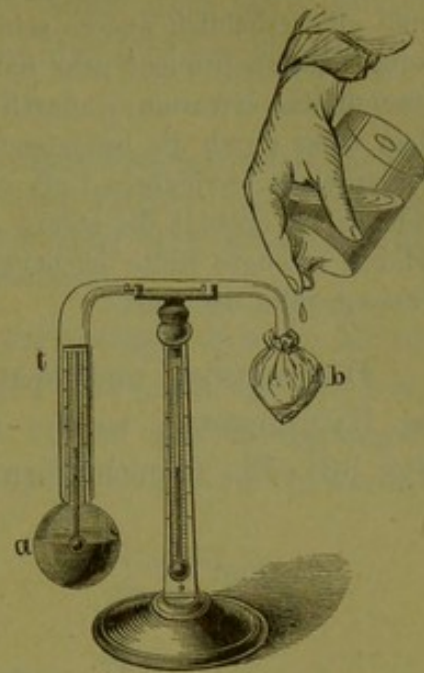
Daniell's Hygrometer.
