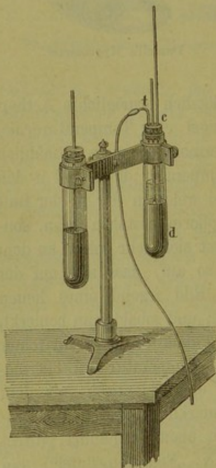
Regnault's Hygrometer.
