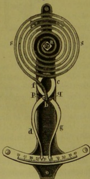
Metall-Maximum-Minimum- thermometer.
