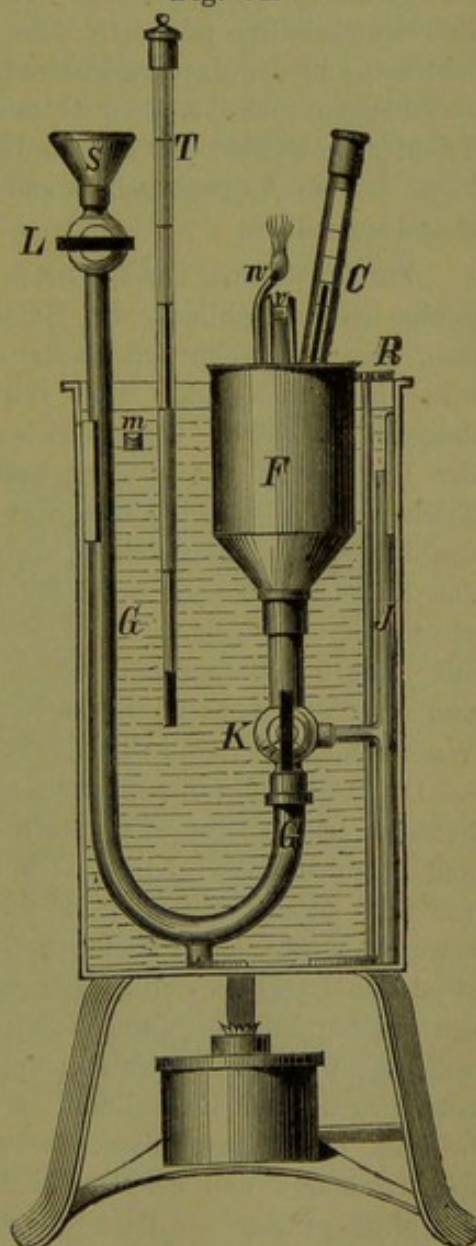
Bernstein's Petroleumprüfer.
