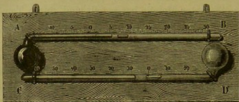
Rutherford's Thermometrograph.
