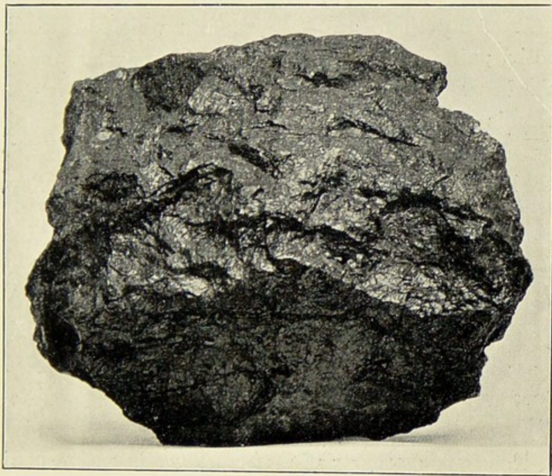
FIG. 4.—PITCHBLENDE.
