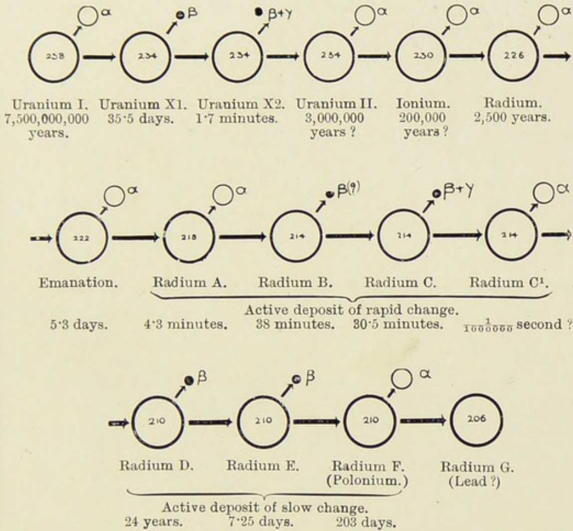
FIG. 7.—DISINTEGRATION SERIES (PROFESSOR SODDY).
