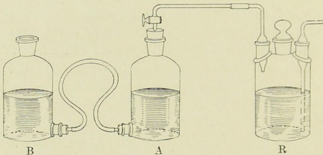
FIG. 11.—SIMPLE EMANATION APPARATUS.
