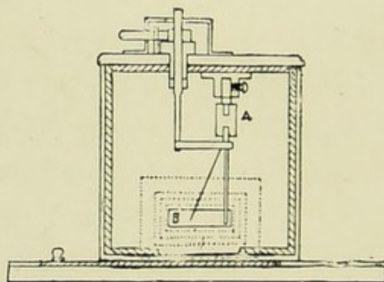
FIG. 9.—GAMMA-RAY ELECTROSCOPE.
