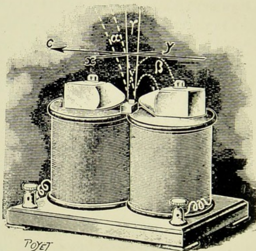
FIG. 5.—MAGNETIC DEFLECTION.
