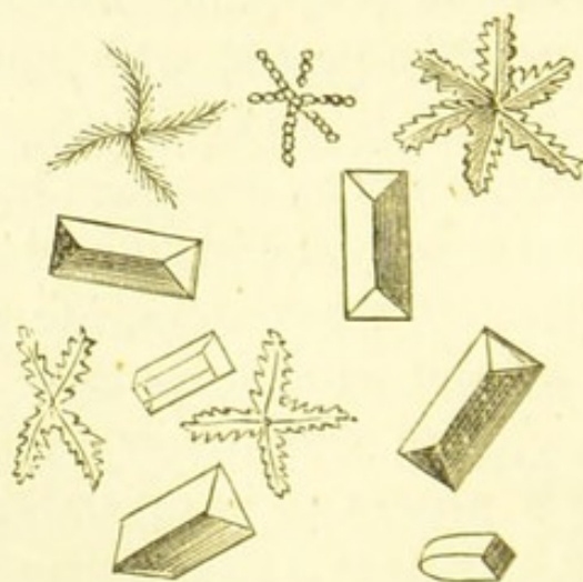
Fig. II. Crystals of Ammonio-magnesium Phosphate
