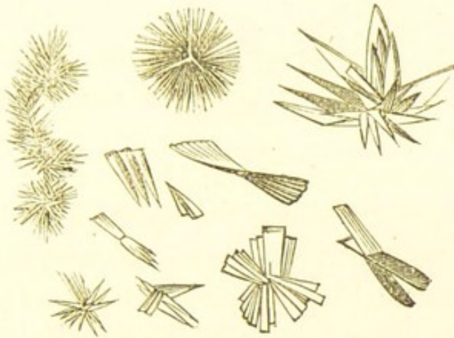
Fig. 12. Crystallized Phosphate of Lime.
