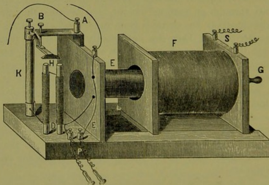
FIG. 17.—INDUCTION COIL.
