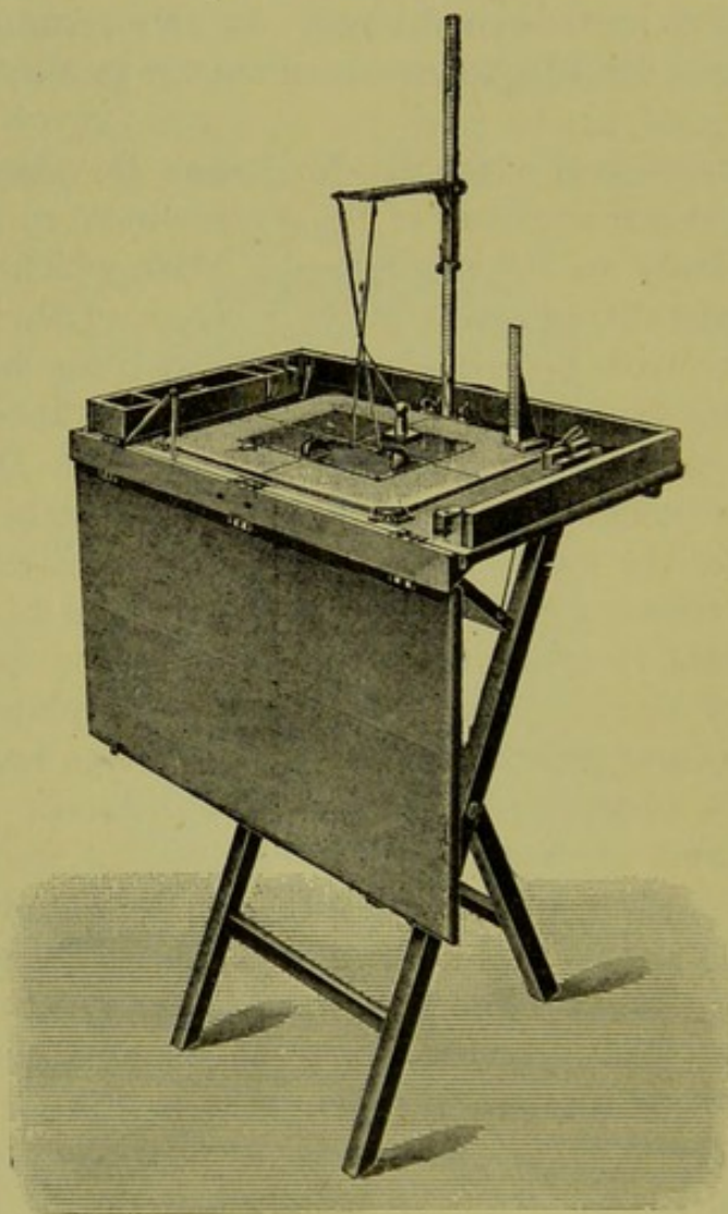
FIG. 153.—DAVIDSON LOCALIZER.
