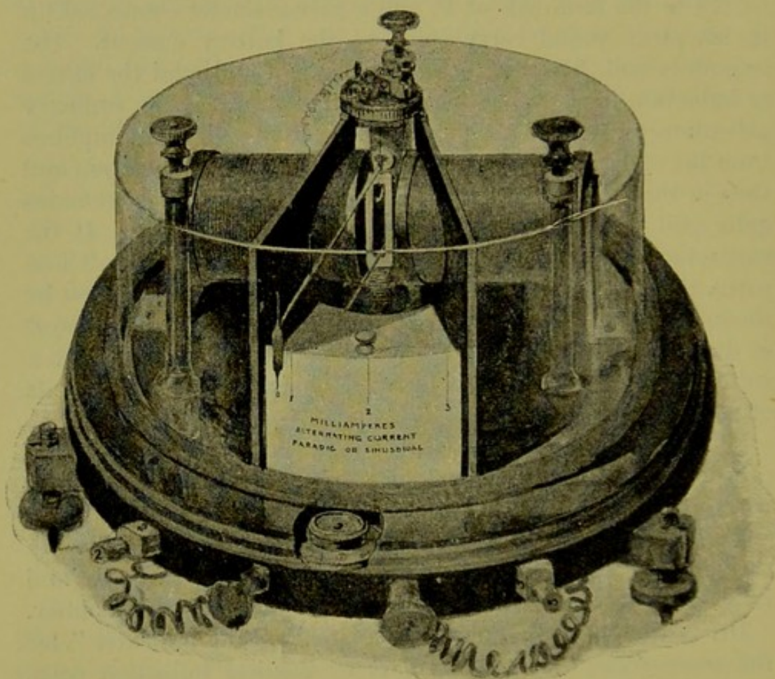
FIG. 32.—THE SLOAN FARADIMETER.
