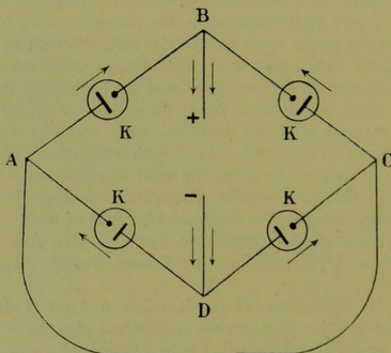
FIG. 90.—ARRANGEMENT OF ALUMINIUM CELLS IN NODON VALVE.
