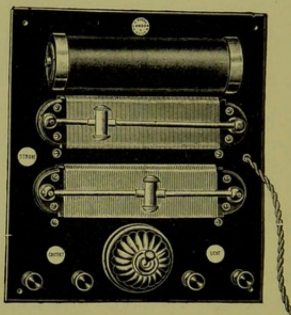
FIG. 83.—TRANSFORMER, WITH TWO SLIDING RESISTANCES, ONE FOR CAUTERY INSTRUMENTS AND ANOTHER FOR SMALL LAMPS.
