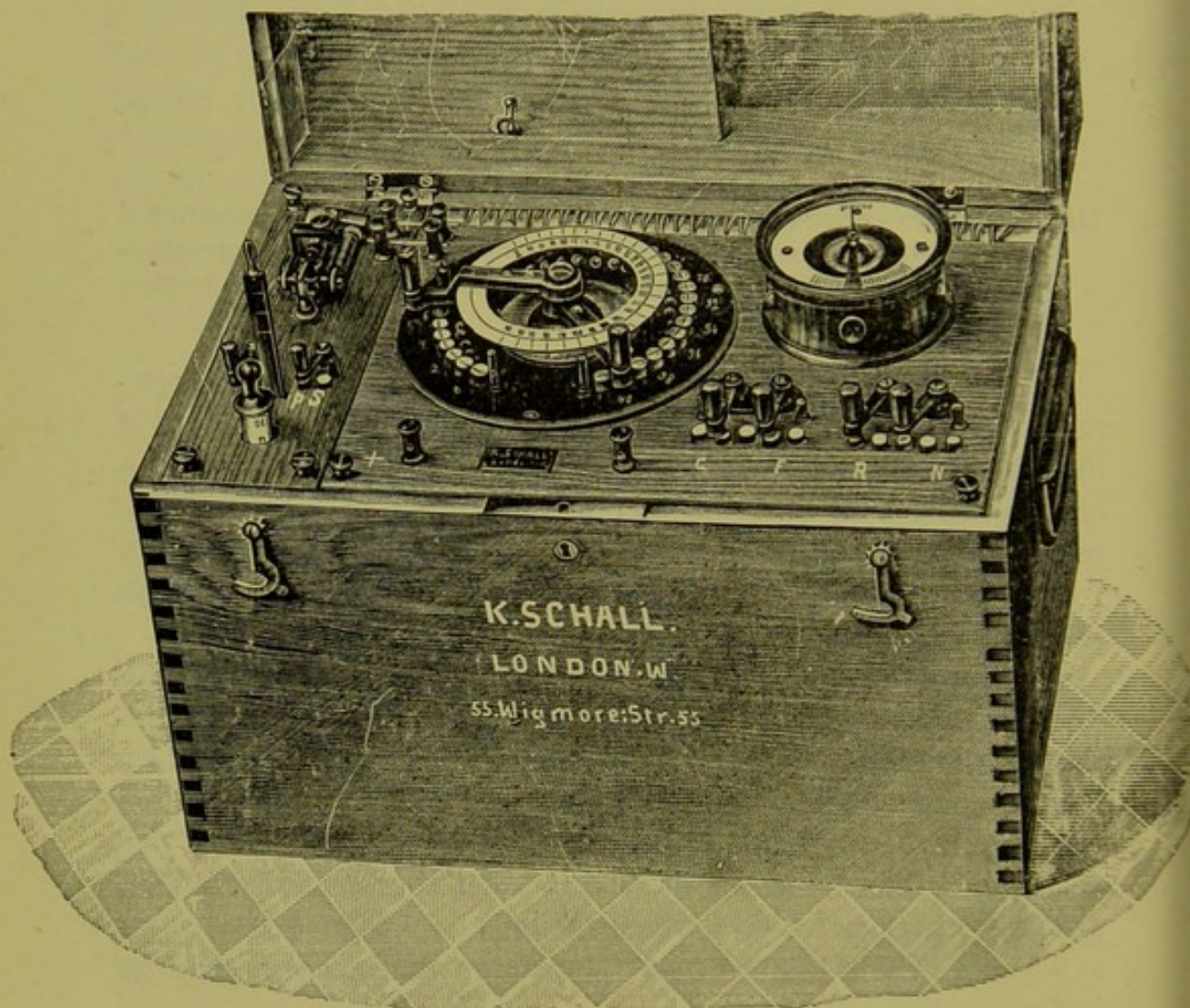
FIG. 22.—COMBINED MEDICAL BATTERY, SHOWING CURRENT COLLECTOR, GALVANOMETER, COMMUTATOR, AND SWITCH.
