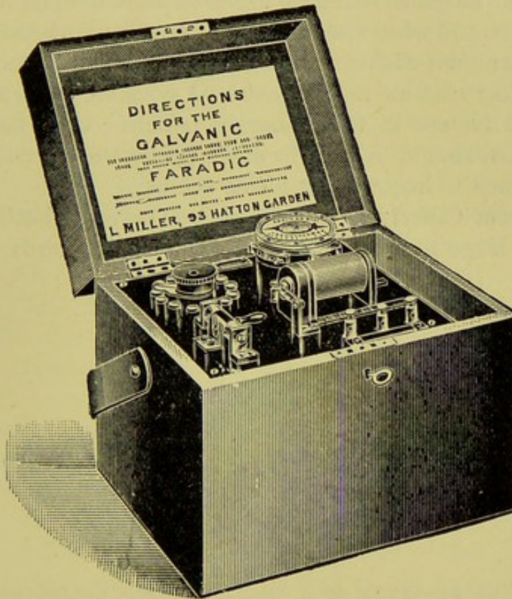
FIG. 23.—COMBINED MEDICAL BATTERY.
