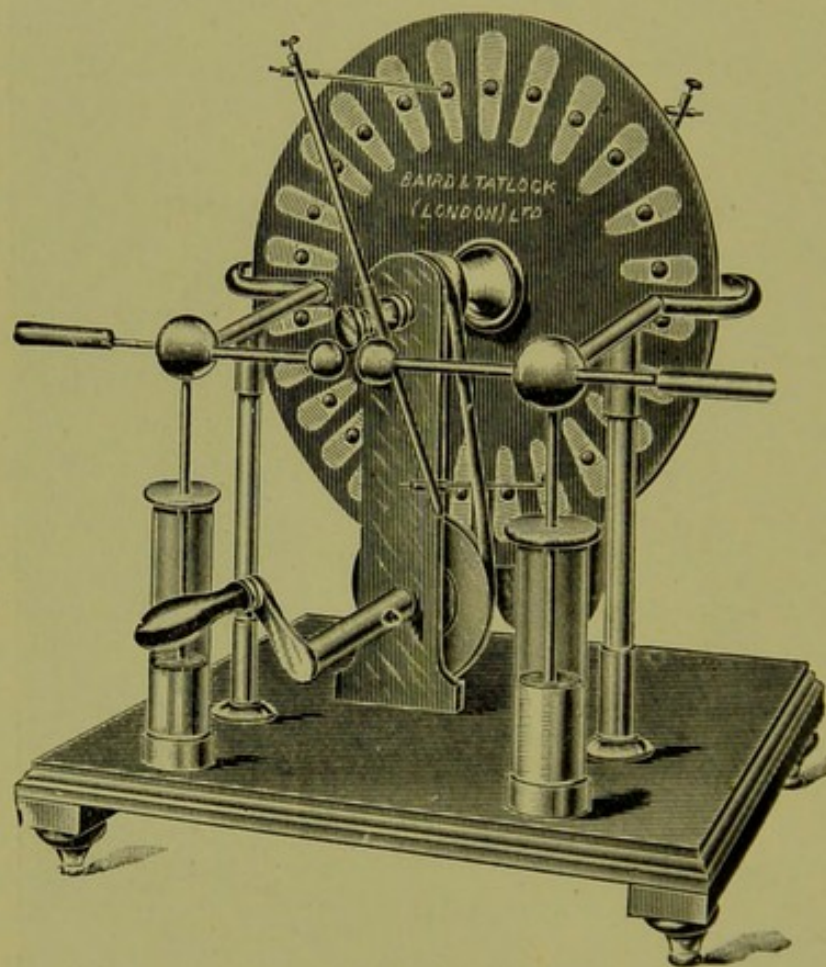
FIG. 117.—WIMSHURST MACHINE.
