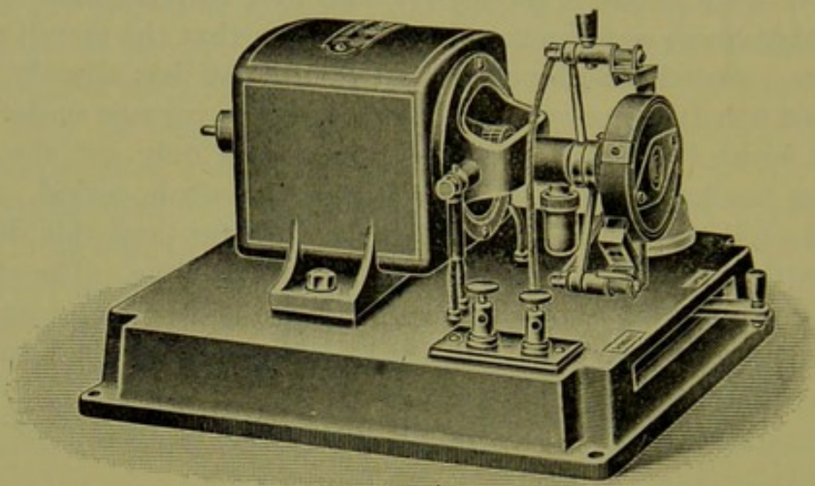
FIG. 40.—LEDUC'S MECHANICAL INTERRUPTER.
