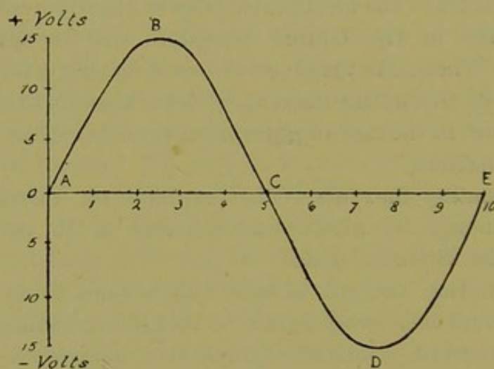
FIG. 20.—GRAPHIC REPRESENTATION OF A STEADILY-VARYING ELECTROMOTIVE FORCE.
