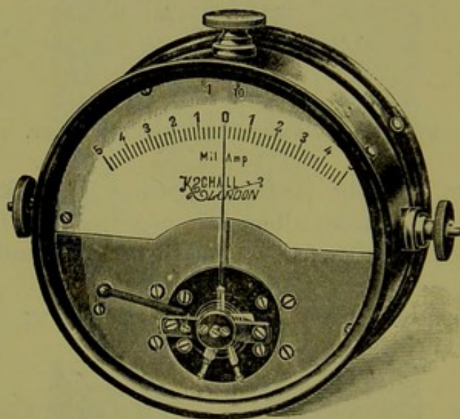
FIG. 28.—D'ARSONVAL MILLIAMPEREMETER.
