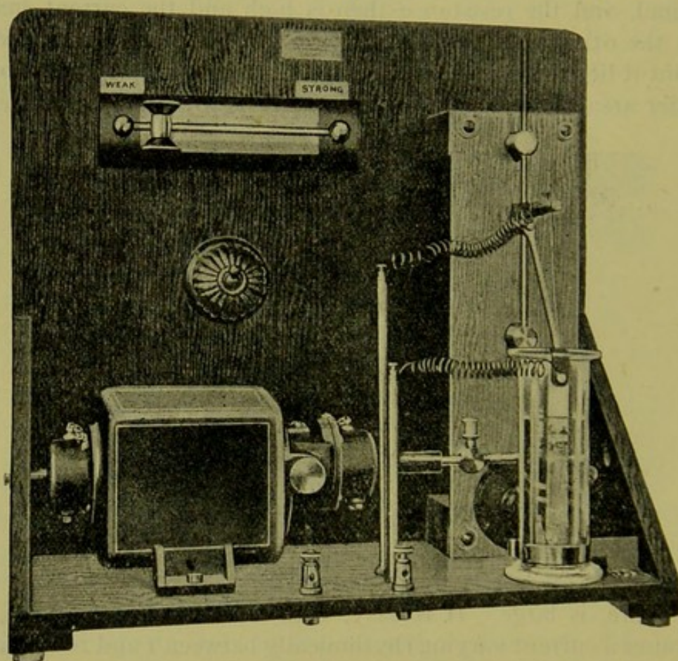
FIG. 58.—RHYTHMIC INTERRUPTER, MOTOR-DRIVEN.*
