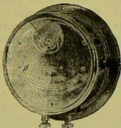
FIG. 132.—HOT-WIRE MILLIAMPÈREMETER FOR HIGH-FREQUENCY CURRENTS.
