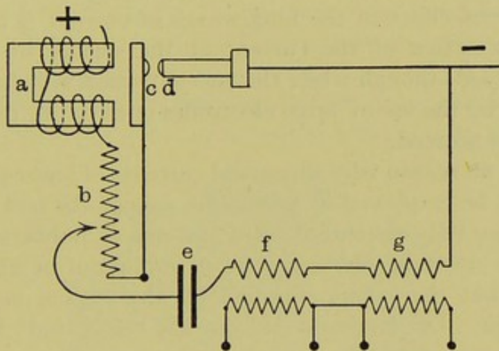
FIG. 84.—PLAN OF CONTINUOUS CURRENT TRANSFORMER.
