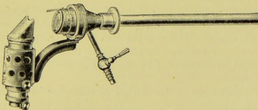
FIG. 72.—SIMPLE FORM OF INFLATING URETHROSCOPE.
