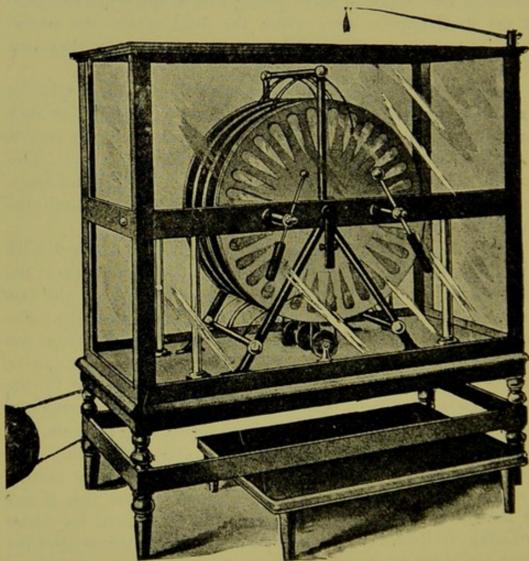
FIG. 118.—WIMSHURST MACHINE.
