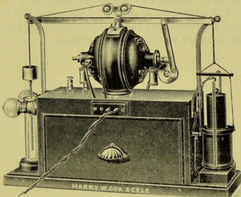
FIG. 59.—DR. HAMPSON'S RHYTHMIC INTERRUPTER.
