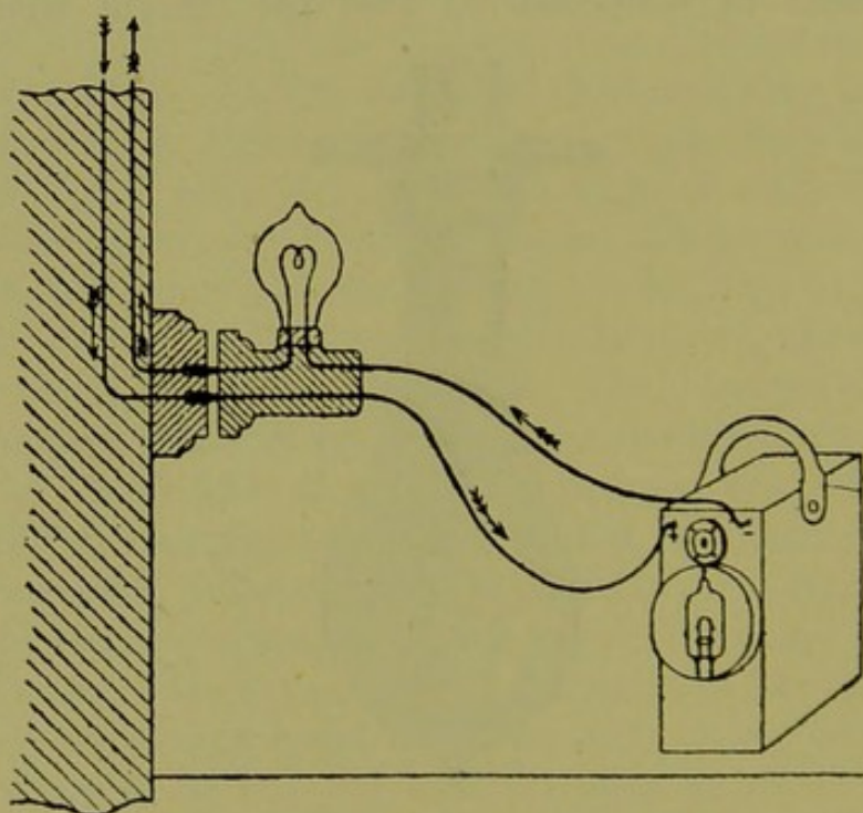
FIG. 89.—ARRANGEMENT OF WIRES IN CHARGING SOCKET.
