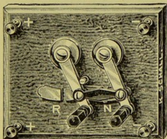
FIG. 27.—DE WATTEVILLE'S COMMUTATOR.
