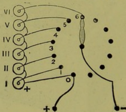
FIG. 24.—PLAN OF A SINGLE CURRENT COLLECTOR.
