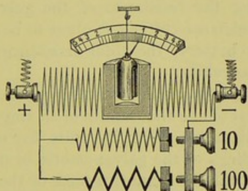
FIG. 29.—PLAN OF SHUNT CIRCUITS OF A GALVANOMETER.
