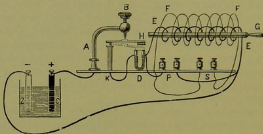
FIG. 16.—ARRANGEMENT OF WIRES IN AN INDUCTION COIL.
