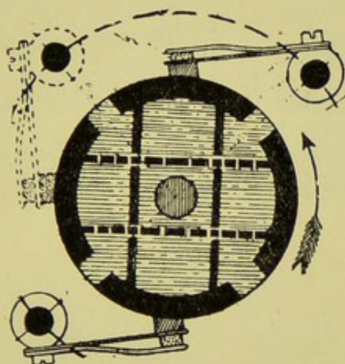
FIG. 39.—PLAN OF COMMUTATOR OF LEDUC.
