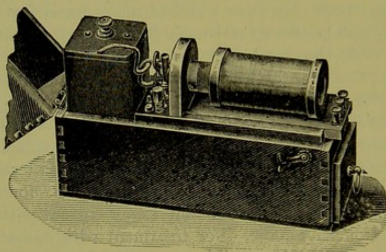
FIG. 31.—PORTABLE SLEDGE COIL, WITH SUBDIVIDED SECONDARY WINDING.
