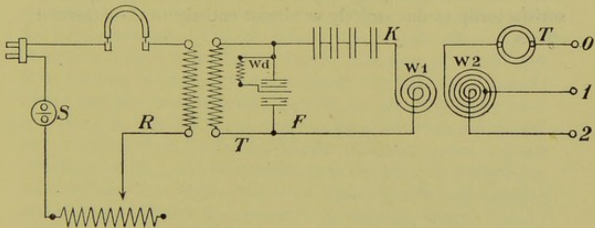
FIG. 135.—PLAN OF DIATHERMY APPARATUS.
