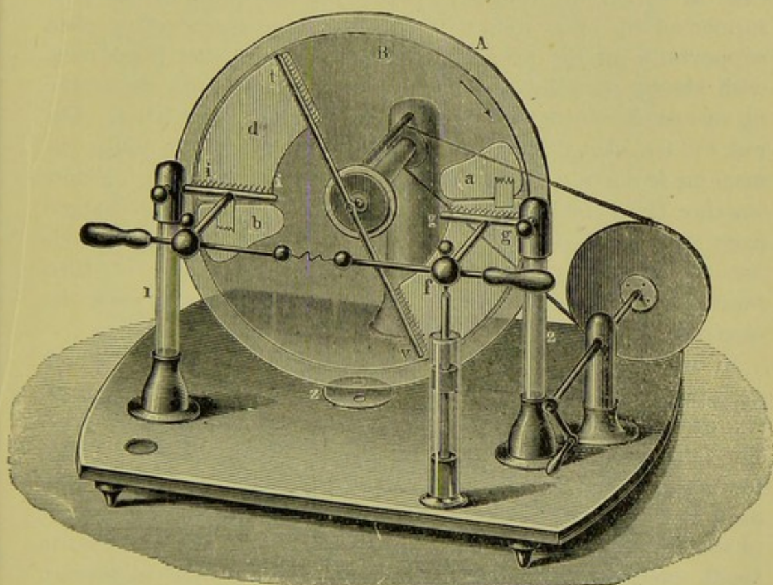
FIG. 115.—HOLTZ MACHINE.
