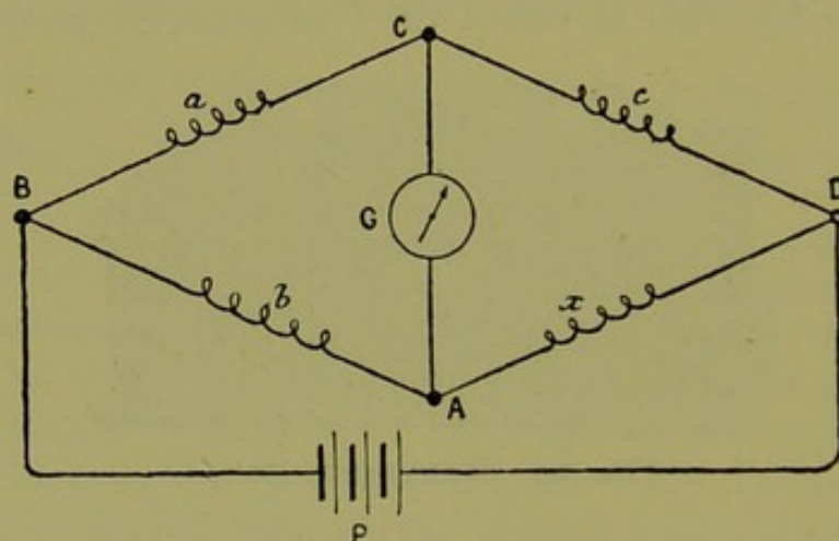
FIG. 15.—WHEATSTONE'S BRIDGE.
