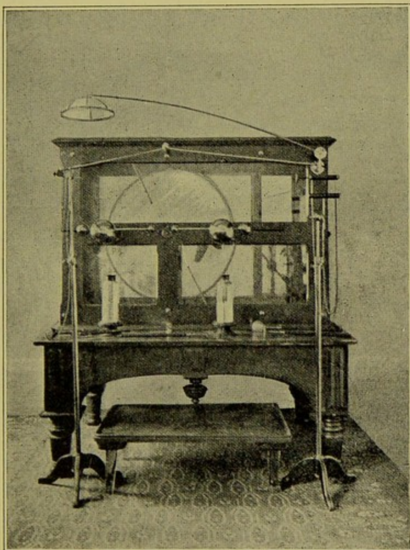
FIG. 116.—HOLTZ MACHINE FOR MEDICAL USE.
