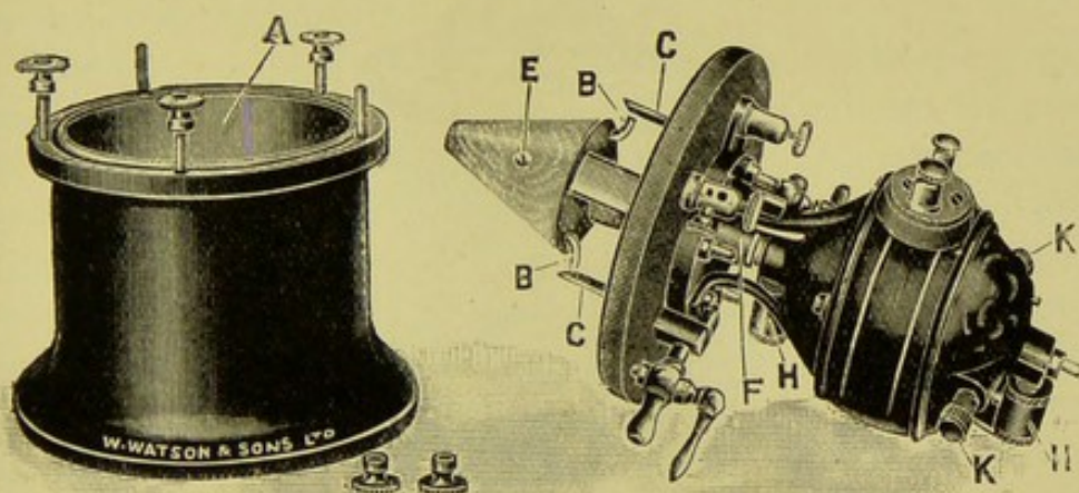
FIG. 104.—"DREADNOUGHT" INTERRUPTER.
