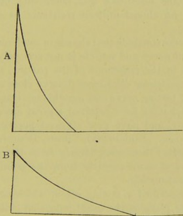
FIG. 157.—CURVES OF DISCHARGE OF A CHARGED CONDENSER.
