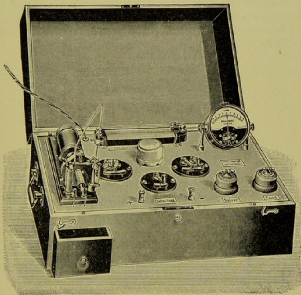
FIG. 82.—COMPLETE FITTING FOR UTILIZATION OF DIRECT CURRENT MAINS FOR MEDICAL USES.
