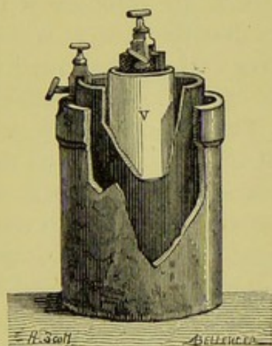
FIG. 6.—TWO-FLUID CELL.
