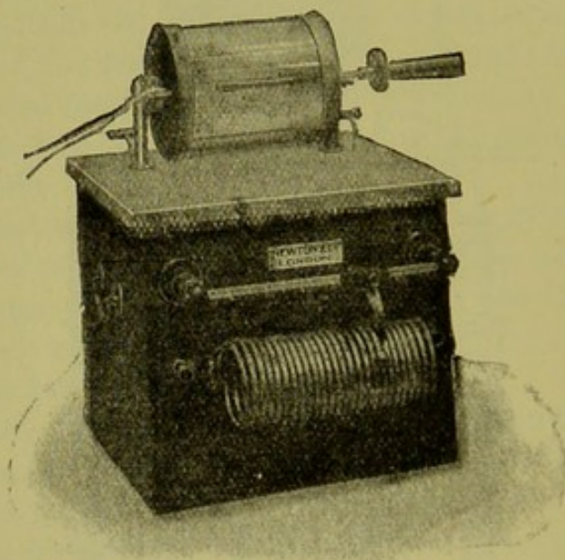
FIG. 130.—HIGH-FREQUENCY APPARATUS, WITH OIL-IMMERSED CONDENSERS.
