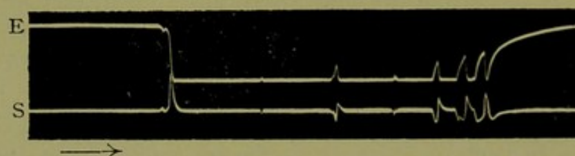
FIG. 33.—IRREGULAR DISCHARGES, DUE TO FAULTY ACTION OF INTERRUPTER.
