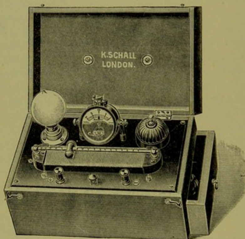
FIG. 81.—SHUNT RESISTANCE, FOR MEDICAL TREATMENT, WITH GALVANOMETER.
