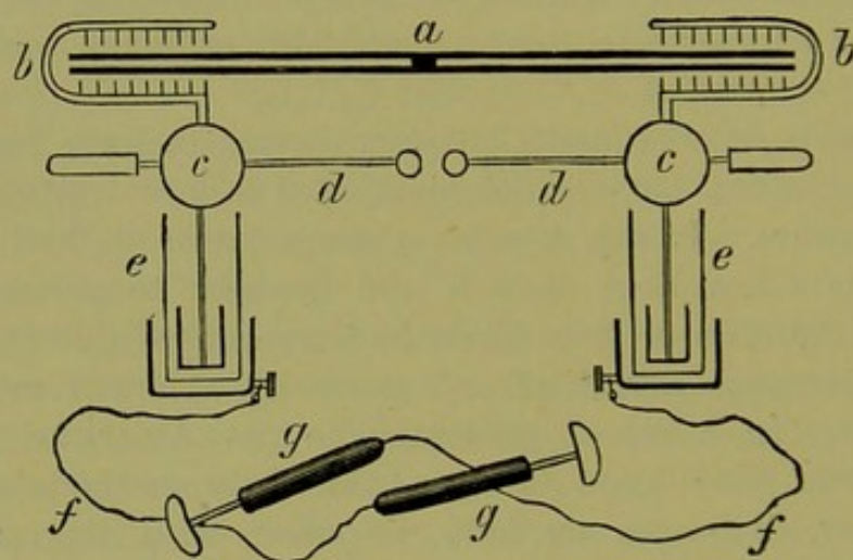
FIG. 123.—PLAN OF DR. MORTON'S METHOD.
