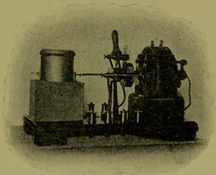
FIG. 41.—MOTOR-DRIVEN INTERRUPTER WITH SPEED-COUNTER AND ADJUSTABLE BRUSH-HOLDER.
