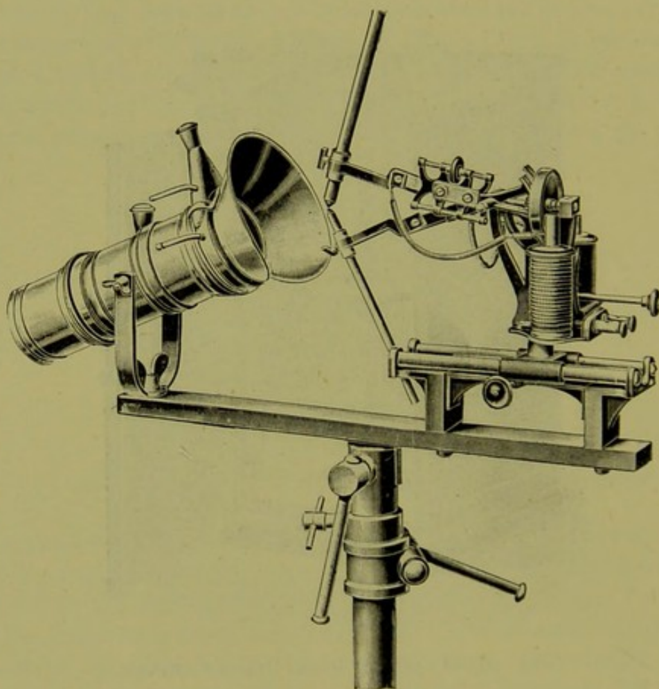
FIG. 97.—THE FINSEN-REYN FORM OF ARC LAMP.
