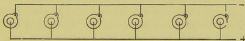
FIG. 5.—SIX CELLS ARRANGED IN PARALLEL.
