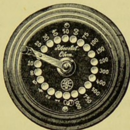
FIG. 44.—ADJUSTABLE RESISTANCE FOR MEDICAL USE.
