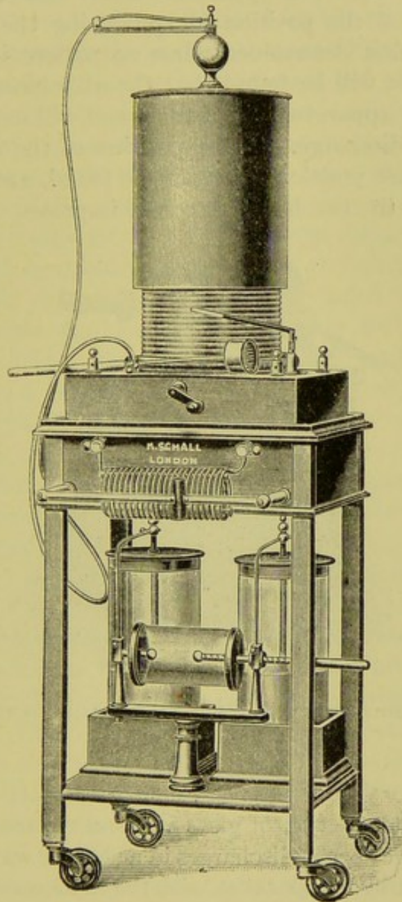
FIG. 129.—HIGH-FREQUENCY APPARATUS, WITH RESONATOR.
