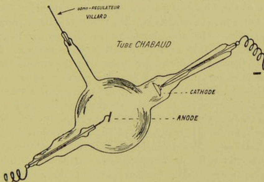
FIG. 140.—CHABAUD TUBE WITH OSMO-REGULATOR.
