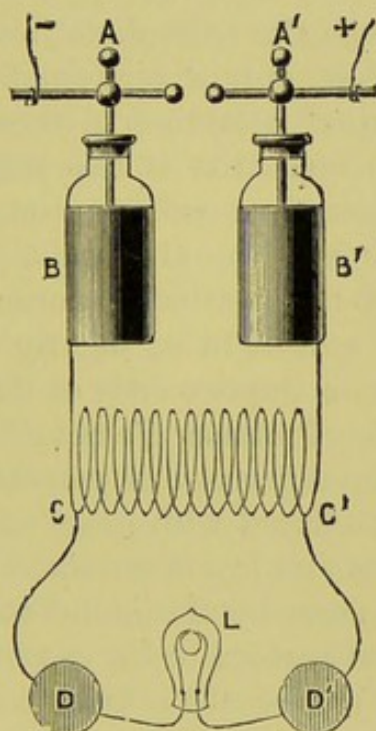
FIG. 124.—ARRANGEMENT OF APPARATUS FOR HIGH-FREQUENCY EXPERIMENTS.
