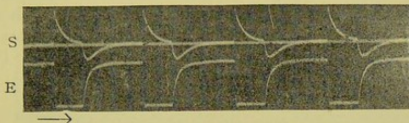
FIG. 34.—CURRENT CURVES OF COIL WITH LONG WINDINGS, BUT WITHOUT CORE (MECHANICAL INTERRUPTER).
