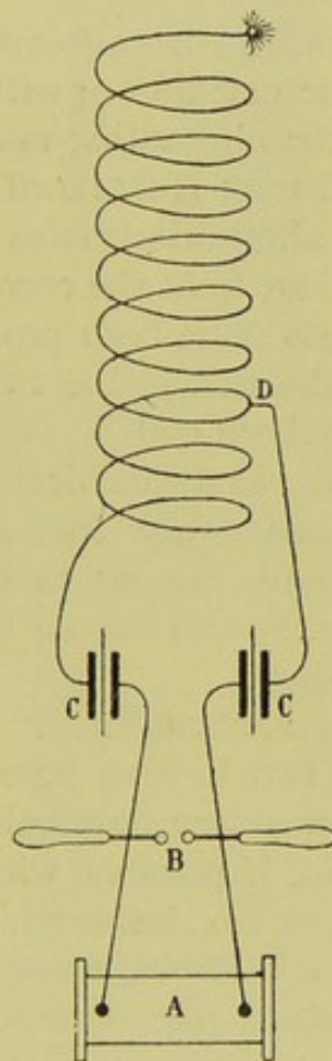
FIG. 128.—PLAN OF OUDIN'S RESONATOR.
