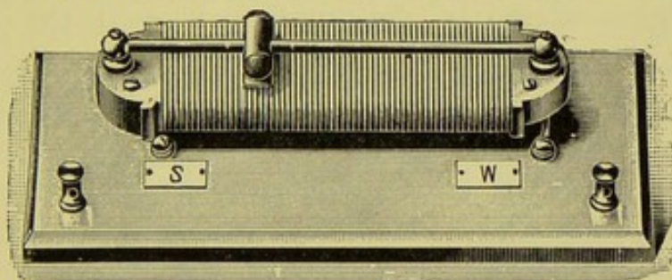
FIG. 45.—WIRE RESISTANCE WITH TRAVELLER. S, strong ; W, weak.
