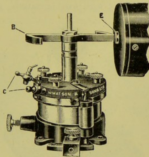
FIG. 102.—BÉCLÈRE'S GAS BREAK.
