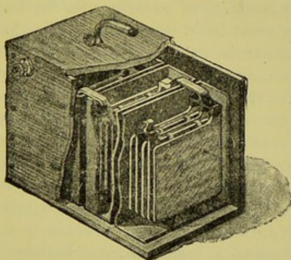
FIG. 10.—ACCUMULATOR CELL, SHOWING ARRANGEMENT OF PLATES.
