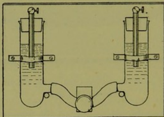
FIG. 48.—LIQUID RESISTANCE OF GUILLOZ.
