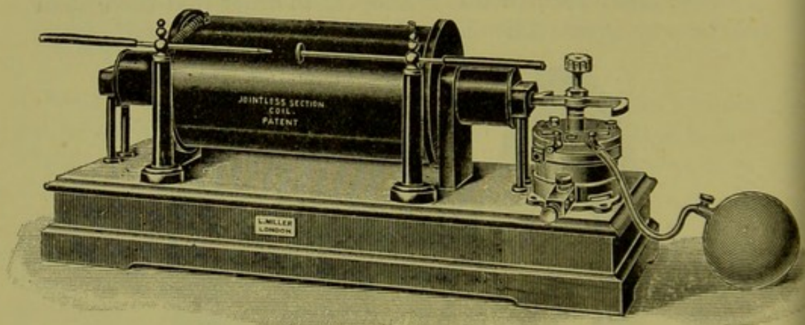
FIG. 101.—COIL FITTED WITH BÉCLÈRE GAS BREAK.
