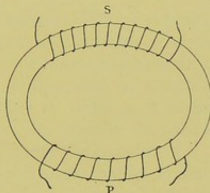
FIG. 21.—PLAN OF TRANSFORMER WITH CLOSED IRON CIRCUIT.
