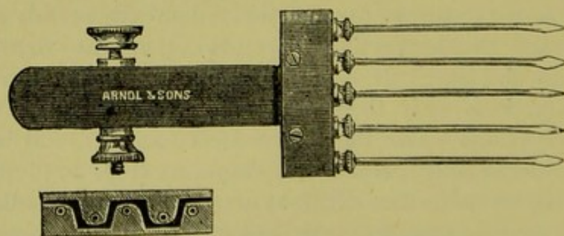
FIG. 174.—BIPOLAR FORK ELECTRODE.
