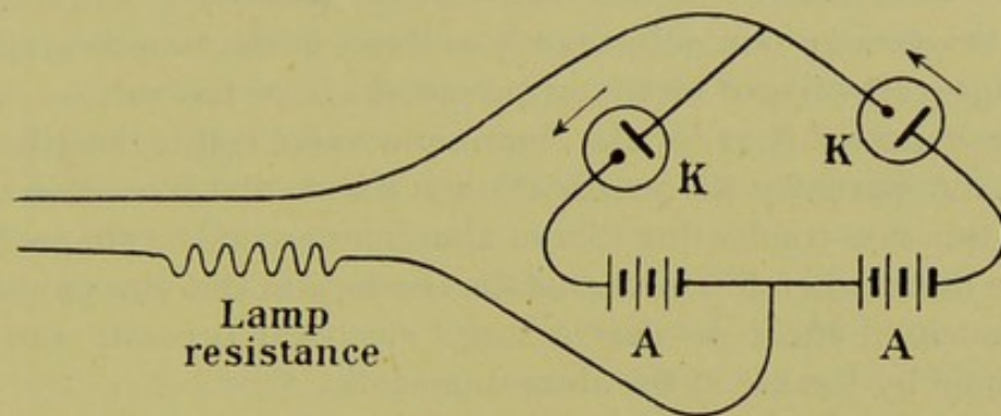
FIG. 91.—ACCUMULATOR CHARGING WITH TWO ALUMINIUM CELLS.
