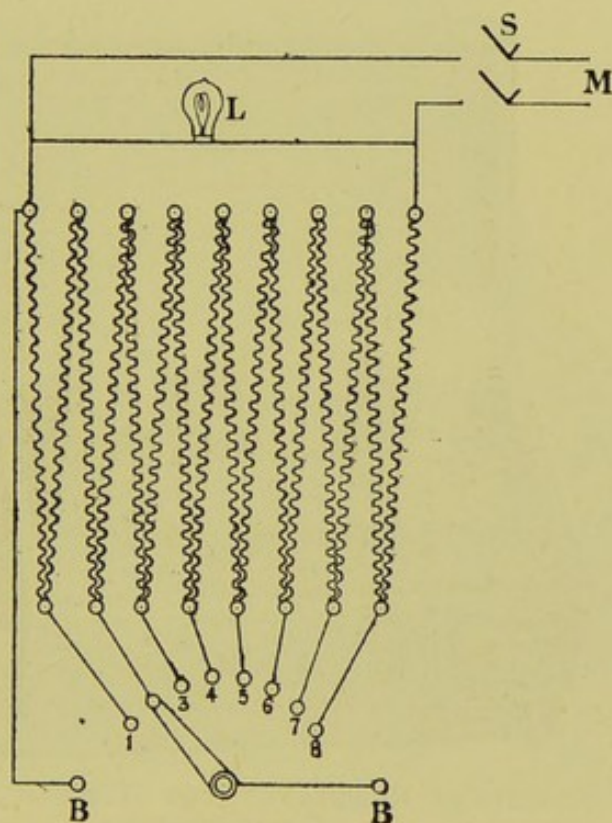
FIG. 80.—PLAN OF SHUNT RESISTANCE FOR LARGE CURRENTS.
