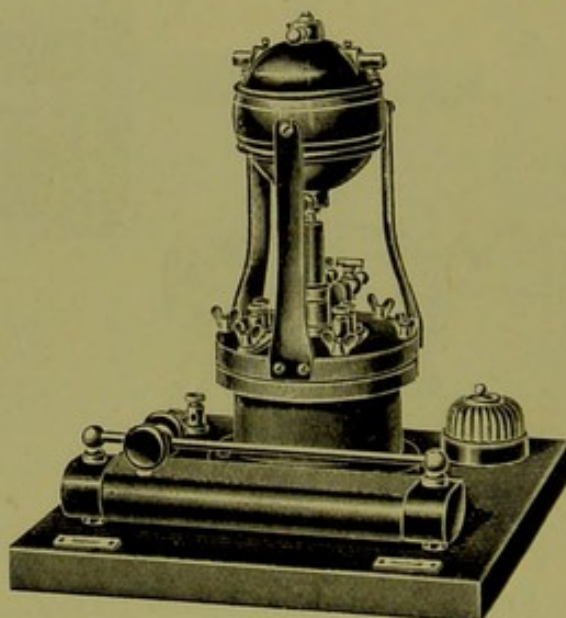
FIG. 103.—MOTOR-DRIVEN GAS BREAK.
