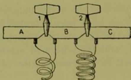
FIG. 13.—PLAN OF RESISTANCE COILS.
