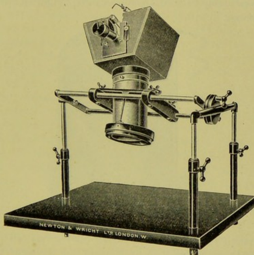
FIG. 151.—TUBE-HOLDER WITH COMPRESSOR DIAPHRAGM.
