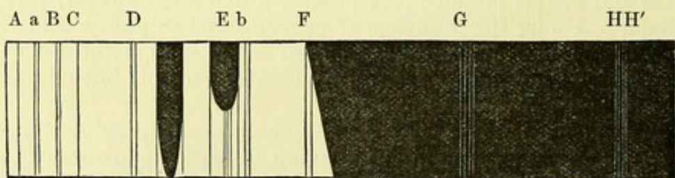
Diagram of Reduced Hematine Spectrum.
