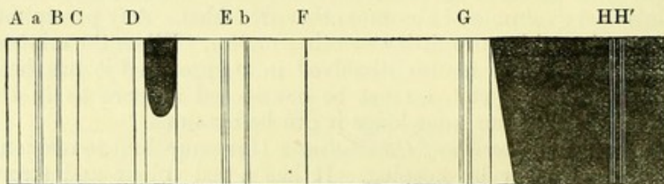
Spectrum of Omicholic Acid.
