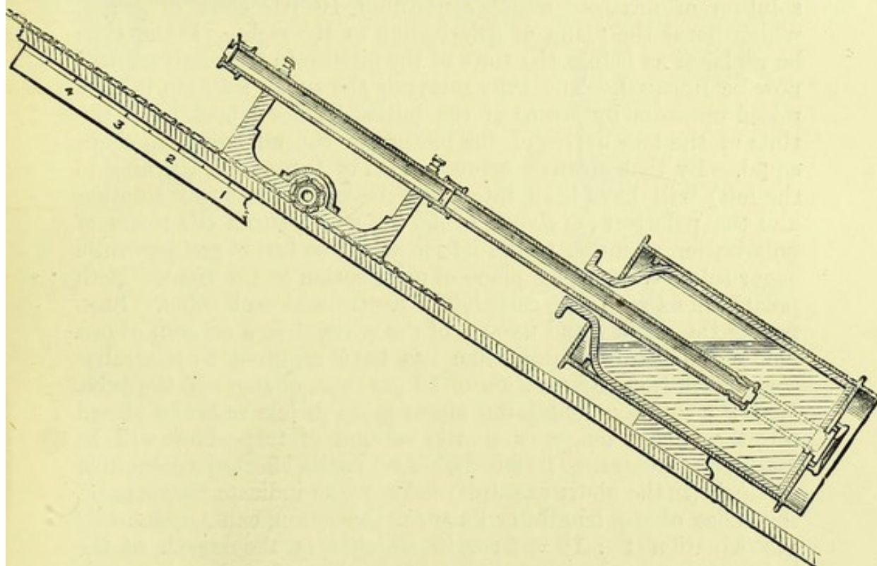
FIG. 6.—Jellett's Polariscope—Section.
