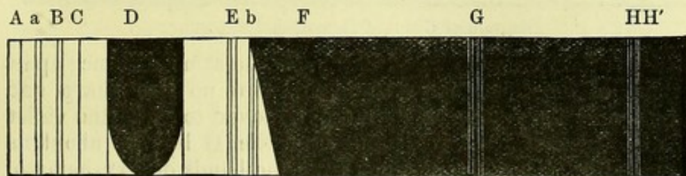
Diagram of Alkaline Hematine in Alcohol Spectrum.
