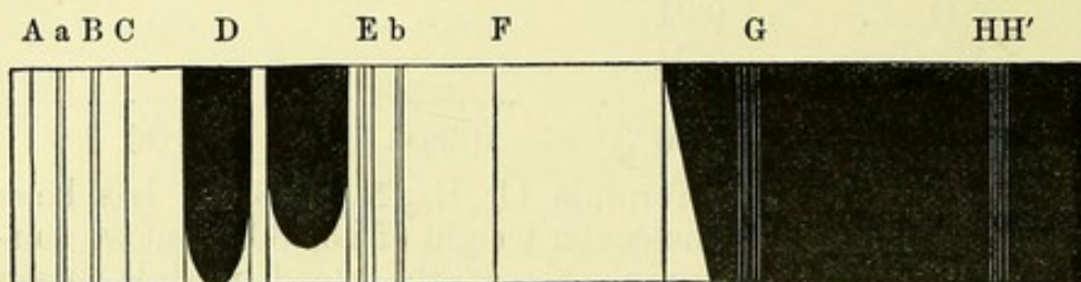
Intensity Diagram of Spectrum of Oxy-hematocrystalline.
