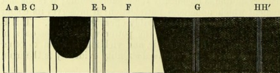
Intensity Diagram of Spectrum of Reduced Hematocrystalline.
