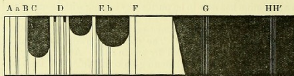
Diagram of Five-Banded Hematine Spectrum.
