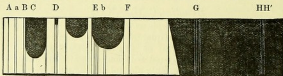
Diagram of Acid Four-Banded Hematine in Alcohol Spectrum.
