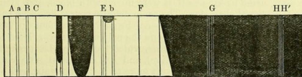
Diagram of Spectrum of Cruentine Sulphate.
