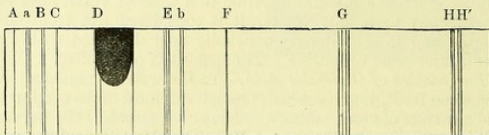
Spectrum of Omicholine.
