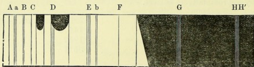
Spectrum of Sulphate of Paramelanine.
