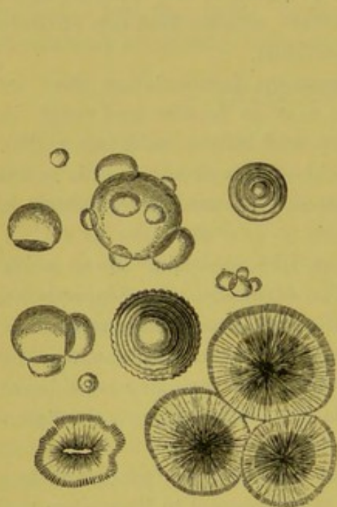
FIG. 22.—Leucine crystals.
