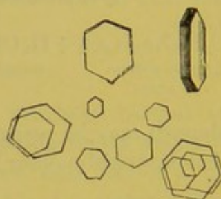
FIG. 50.—Cystin crystals.
