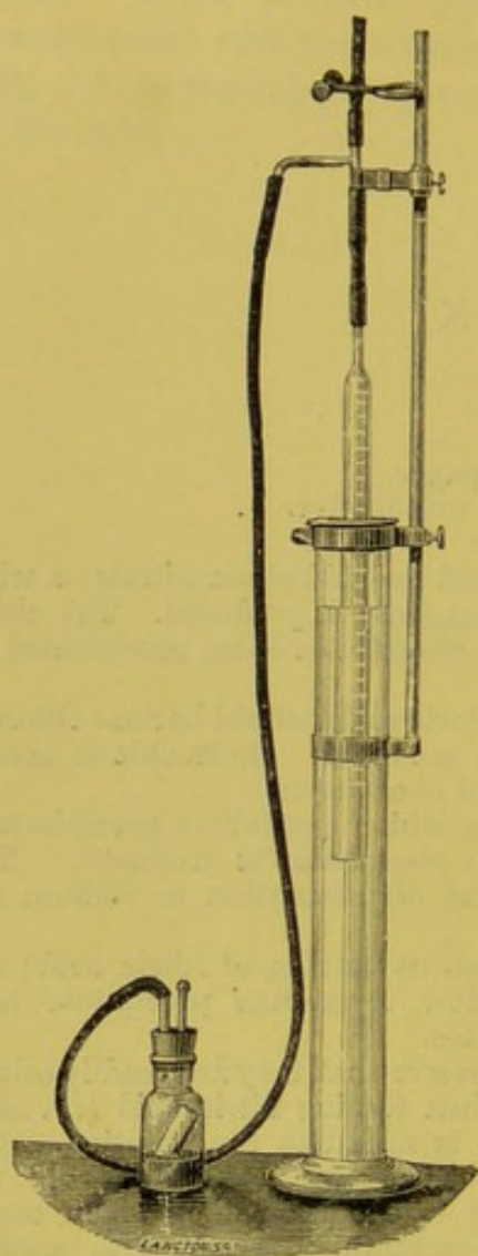
FIG. 41.—Dupre's urea apparatus.
