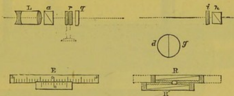
FIG. 75.—Diagram of optical arrangements in Soleil's saccharimeter.
