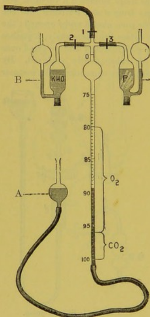
FIG. 81.—Waller's apparatus for gas analysis.
