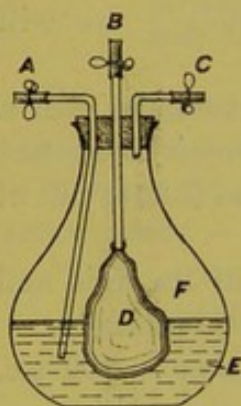
FIG. 38. Loewy's Aërotonometer.
