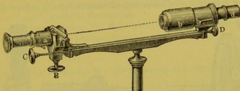
FIG. 74.—Soleil's saccharimeter.
