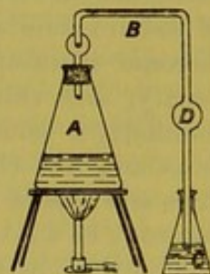
FIG. 82. — Kjeldahl's method: distilling apparatus.
