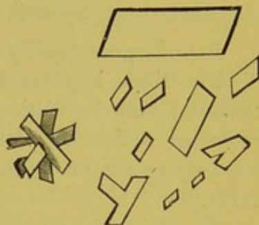
FIG. 3.—Milk-sugar crystals.
