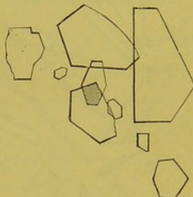
FIG. 1. —Dextrose crystals.
