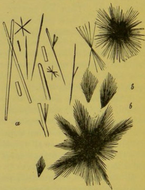
FIG. 23.—Tyrosine crystals.
