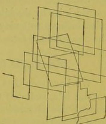
FIG. 25.—Cholesterin crystals.
