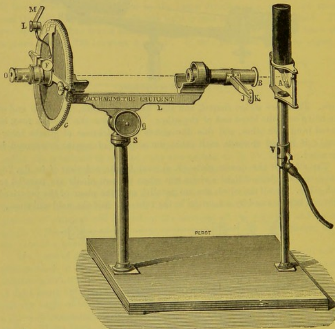
FIG. 76.—Laurent's polarimeter.
