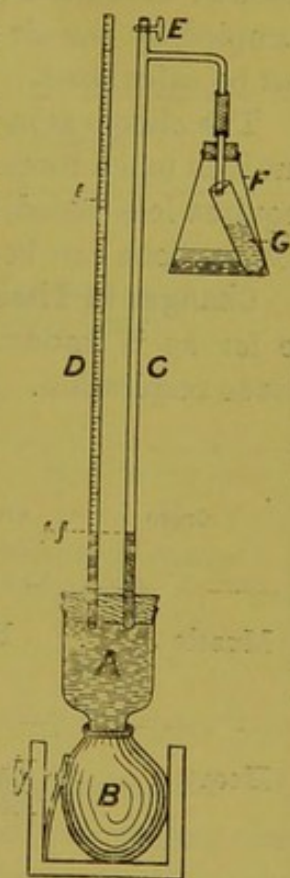
FIG. 40.—Barcroft's apparatus for obtaining the blood gases.
