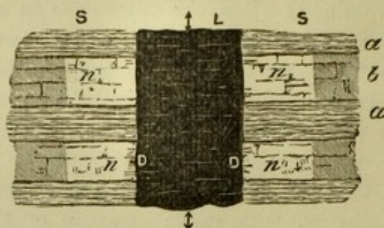
FIG. 6.—Lava column in a state of rest.
