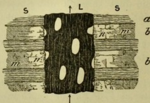
FIG. 7.—Lava column during flow.
