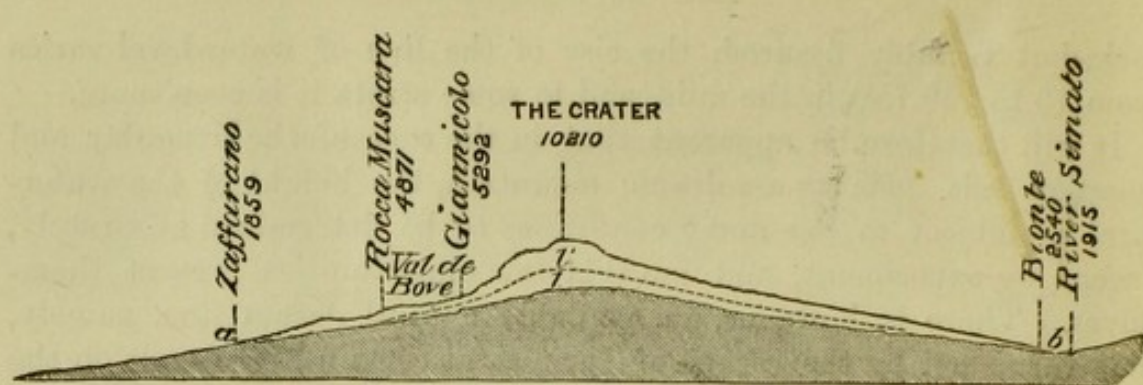
FIG. 3.—Diagram section of Etna.
