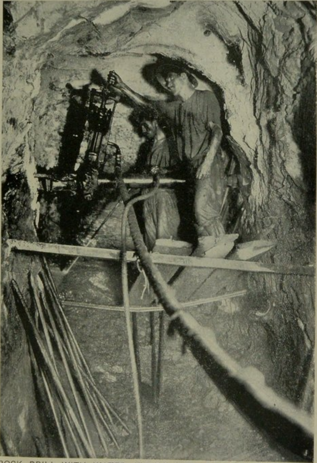
ROCK DRILL WITH WATER JET AT NORTH JOHNSTON Q.M. CO. BEGINNING OF A CROSSCUT.
