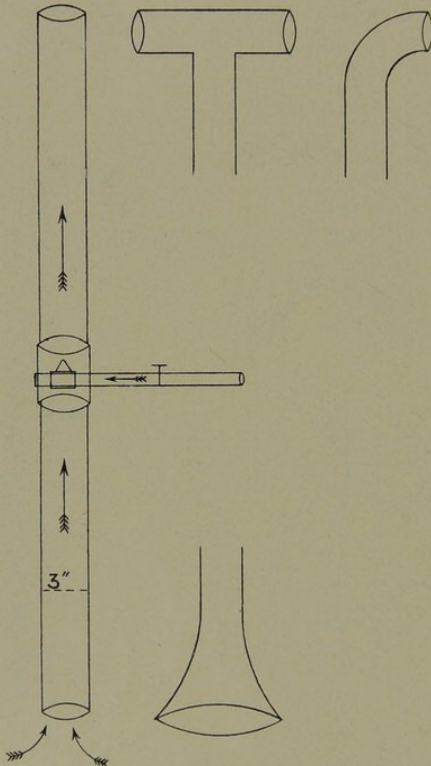
Compressed air ejector or "vacuum air-blower." Compressed air pipe entering vertical pipe at right angles and smaller air jet is directed along the long axis of this vertical pipe, the diameter of which is 3 inches. (Used in Suffolk United Mine.)
