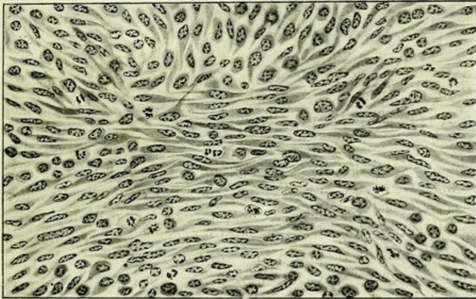
FIG. 14. — Sarcome transplantable.
