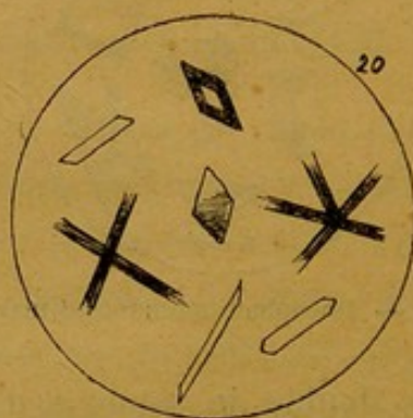
Fig. 20. — Oxalate manganeux ammoniacal.
