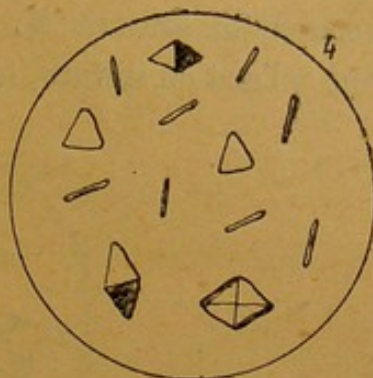
Fig. 4. — Fluoaluminate d'ammonium.
