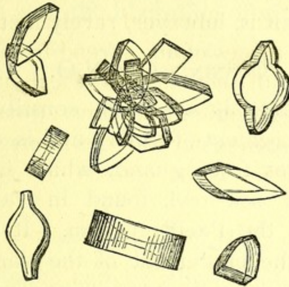
Fig. 4. Uric Acid.
