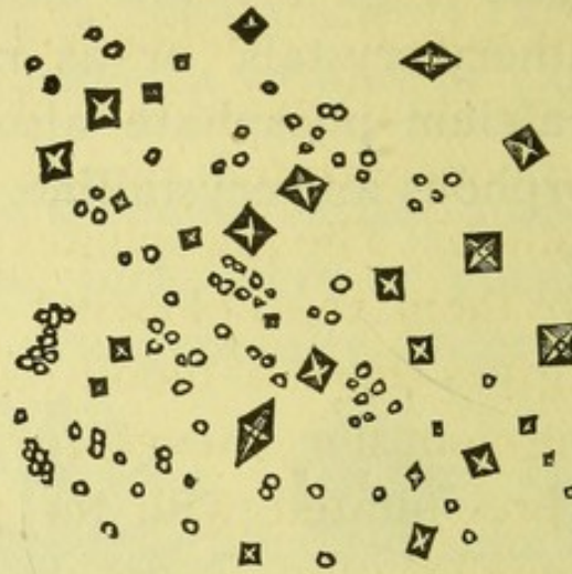
Fig. 13. Calcium Oxalate.
