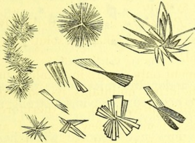
Fig. 12. Crystallized Phosphate of Lime.
