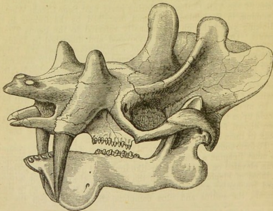
Restored skull of Uintatherium ( Dinoceras , Marsh).
