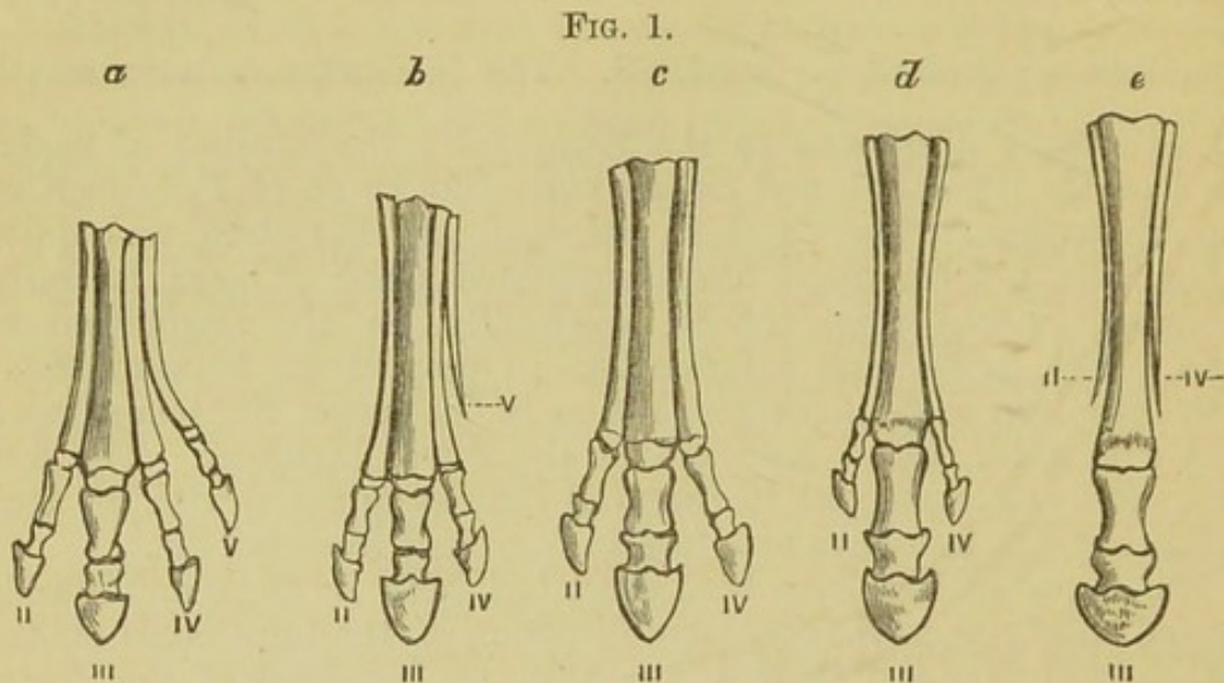
Diagram of several stages of modification of the feet of extinct forms of American horse-like animals (chiefly from Marsh), showing gradual reduction of the outer, and enlargement of the middle toe (III).
