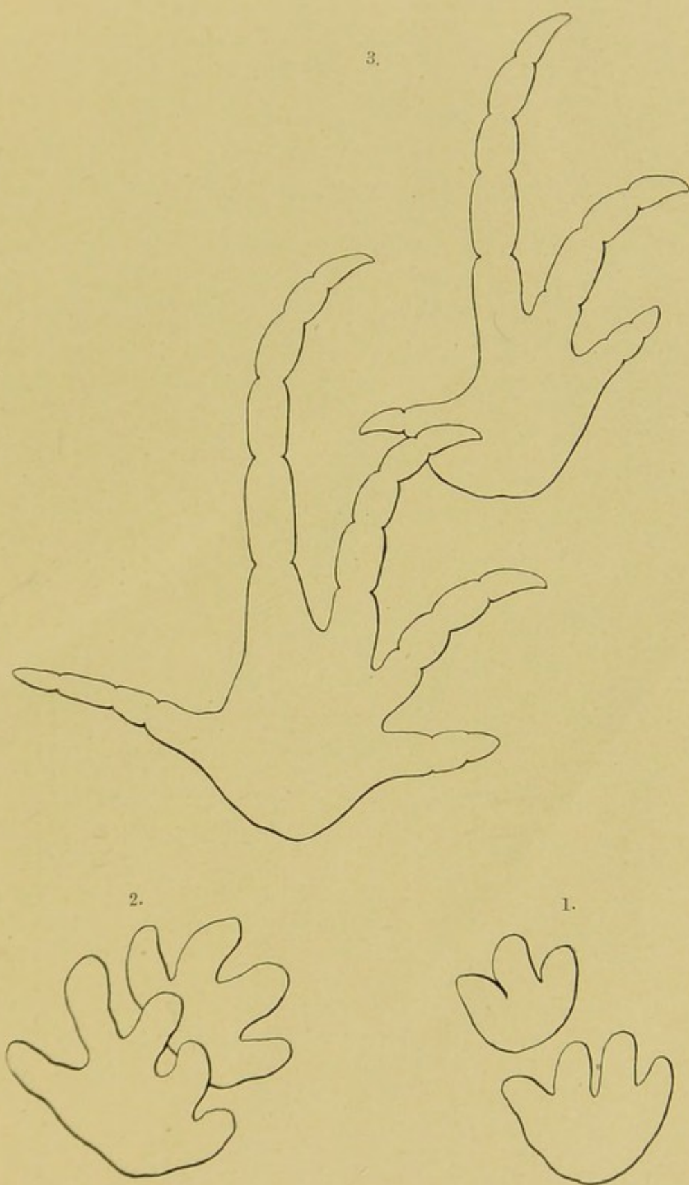
FOOTPRINTS FROM KANSAS COAL MEASURES. Natural size.
