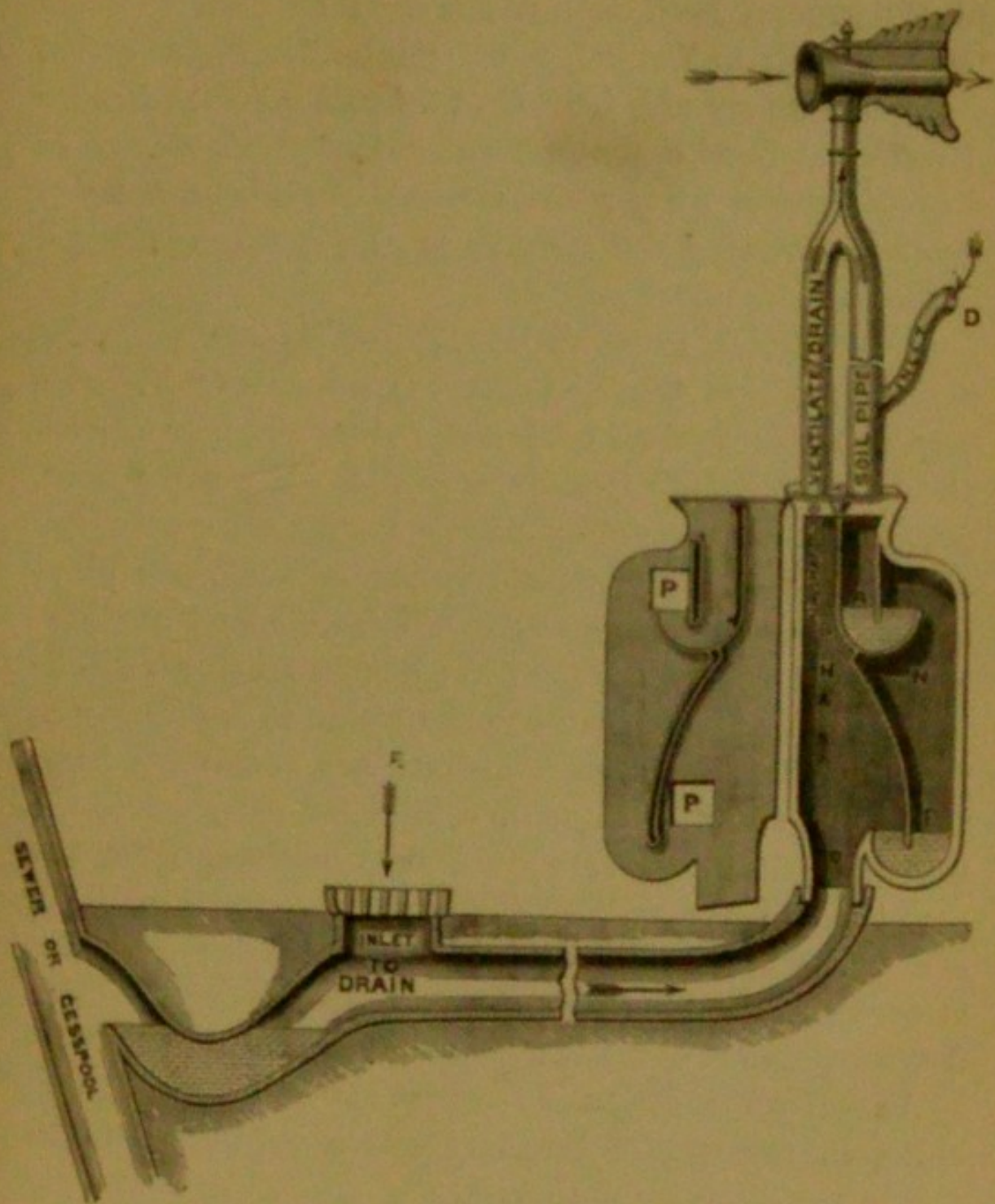
The above is a simpler mode of effecting the same object as shown in Plate 2. Patent dated 2nd July, 1875, No. 2401.
