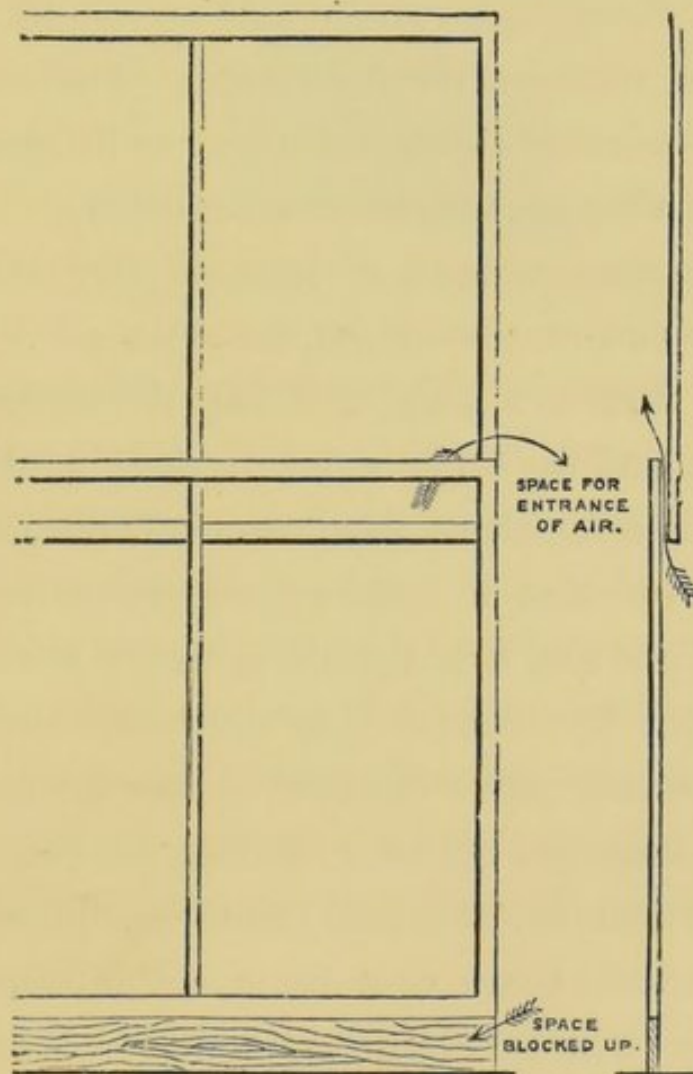
Plan of "Costless Ventillation."
