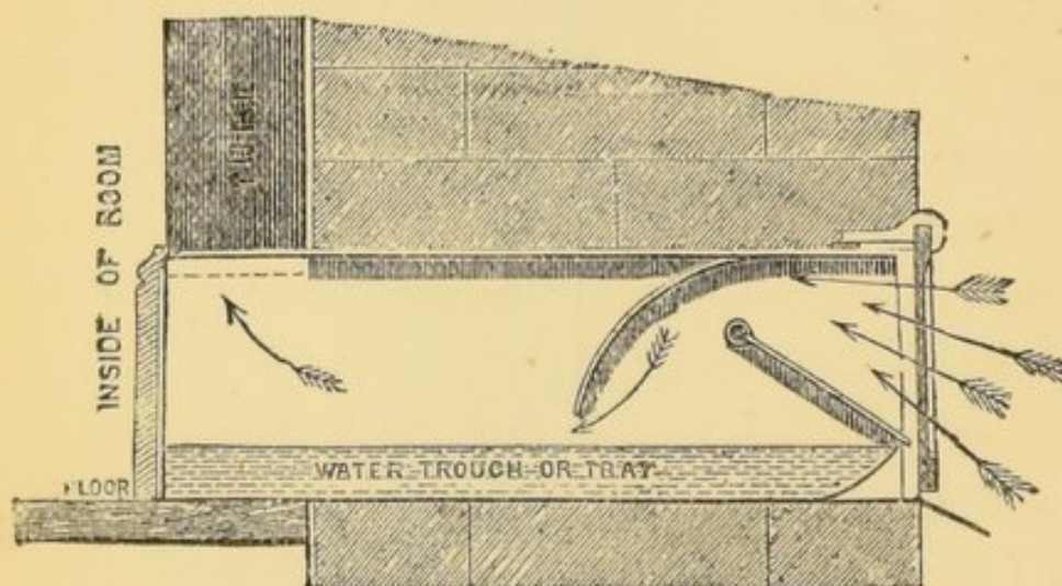
Water Tray for Vertical Tube Ventilator.
