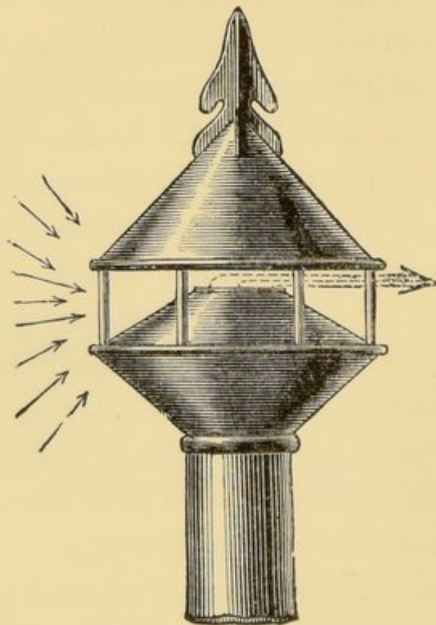
Fixed Cowl.
