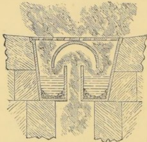
Bell Trap.
