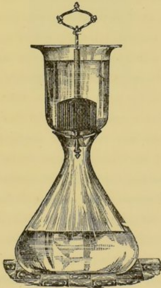
Decanter Filter.
