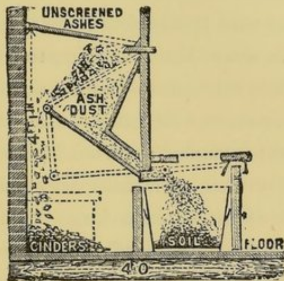
Cinder Sifting Ash Closet.
