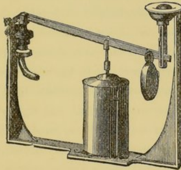
Water Closet Supply Valve with Bellows Regulator.
