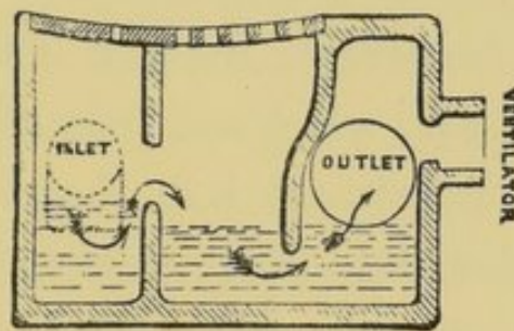
Mansergh Trap.
