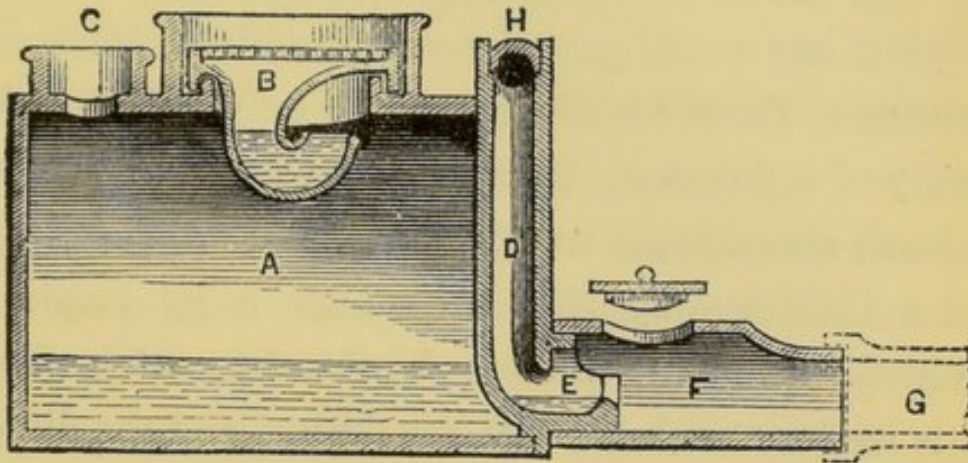
Field's Flush Tank.
