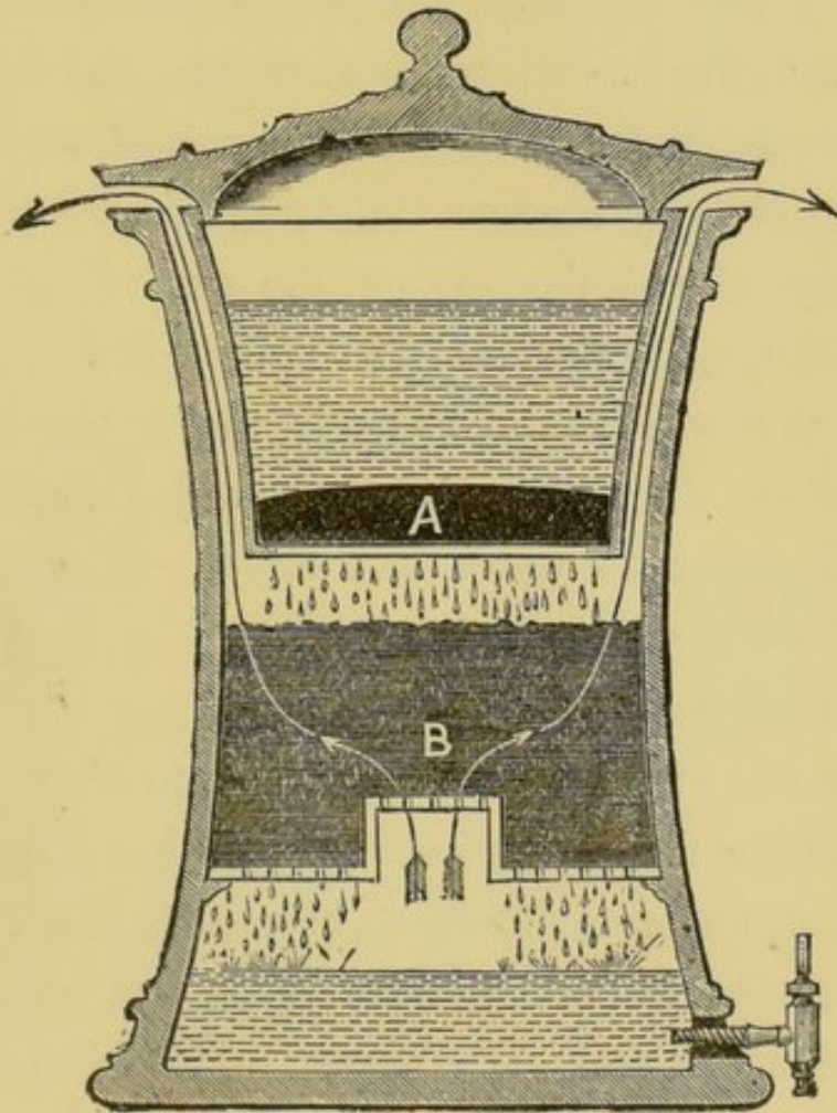
Aërating Filter.
