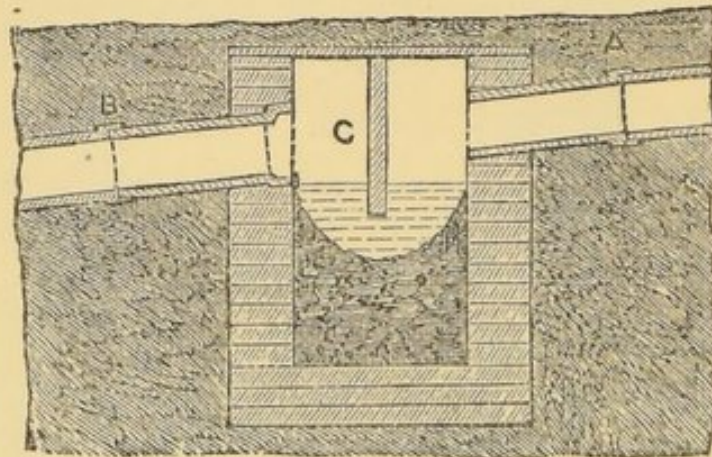
DIPSTONE TRAP.
