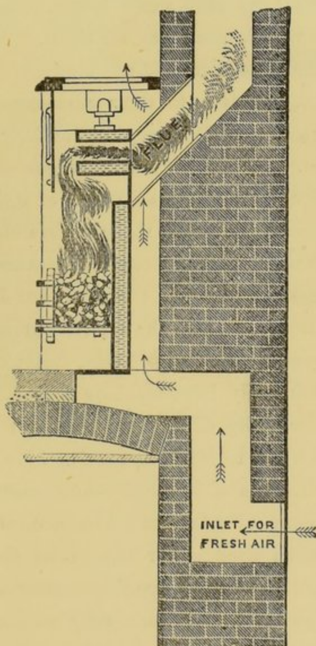
Thermhydic Grate (Section).
