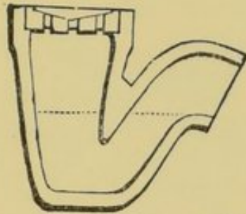
Stoneware Siphon Gully.
