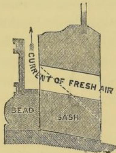
Currall Ventilator (as fixed to Window).
