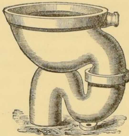
"Wash-out" Water Closet.
