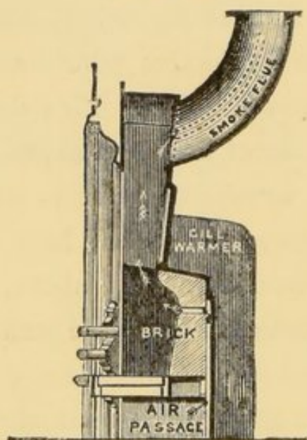
The Galton Ventilating Grate.
