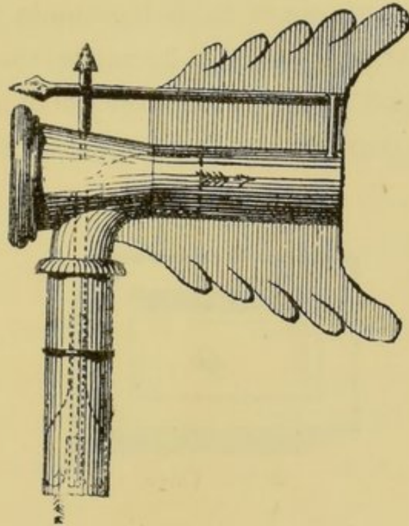
Rotating Cowl.
