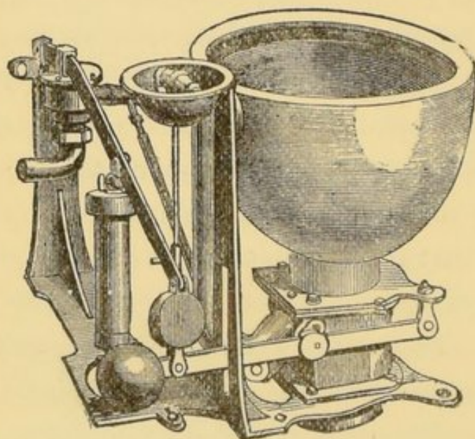
Valve Water Closet.
