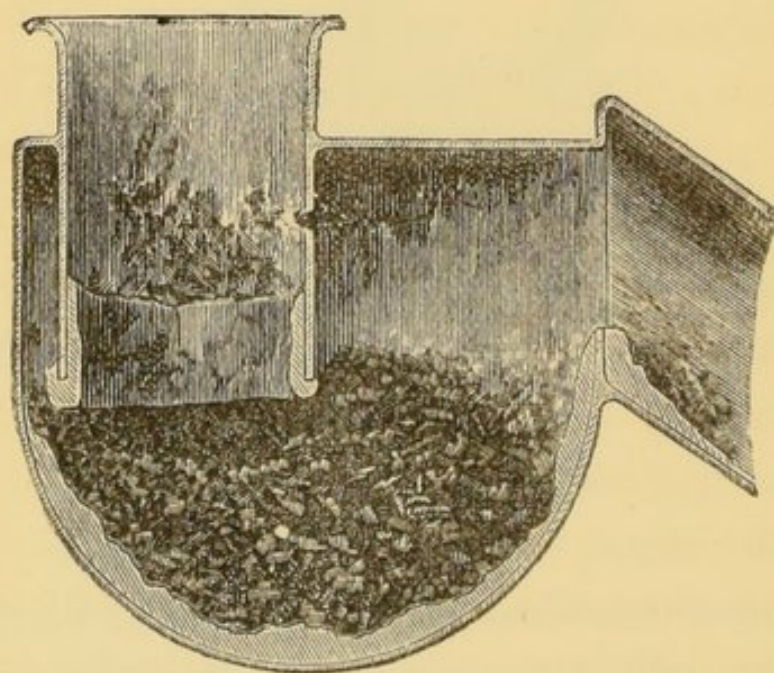
D-trap with foul deposit in it.
