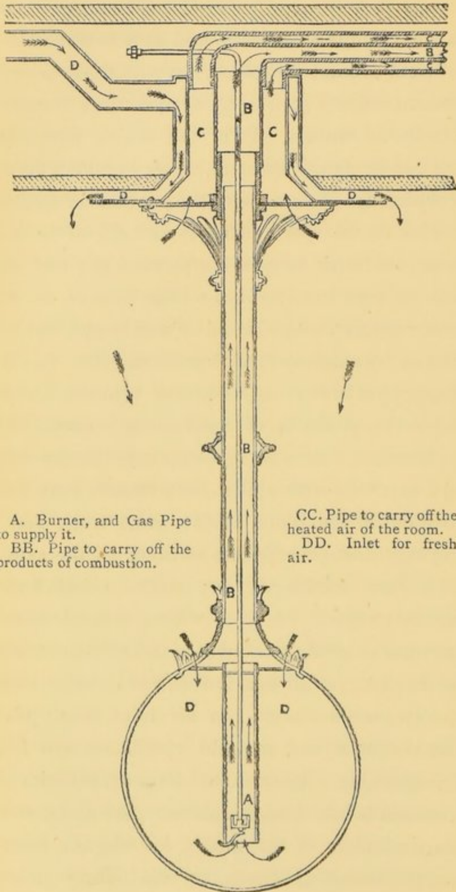
Ventilating Globe-Light.
