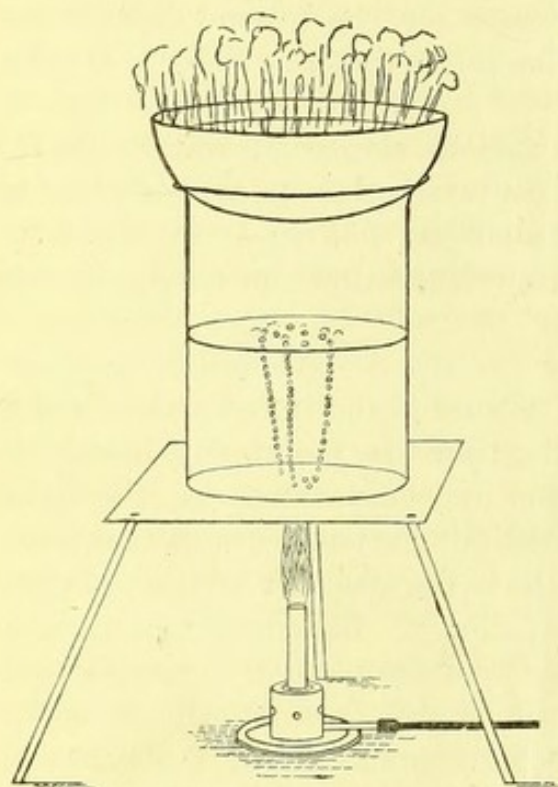
Process (a). Platinum Dish in Water Bath
