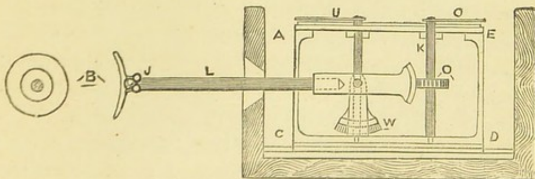
FIG. 16.—Sectional side elevation.
