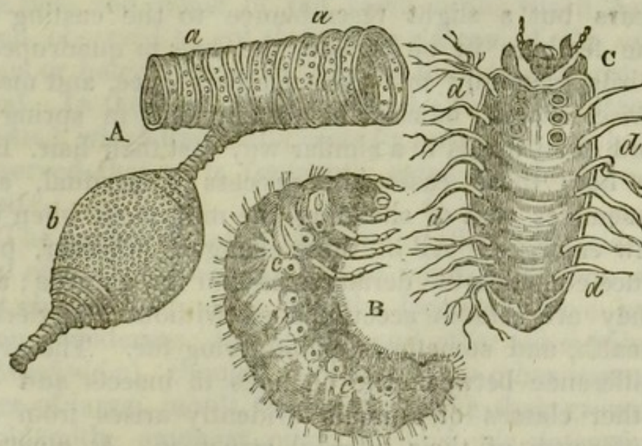
Exuvia and pulmonary vessels of the rhinoceros beetle ( Oryctes nasicornis ). A, magnified view of a pulmonary branch and vesicle; a a , pulmonary branch, composed of a membranous sheath and cartilaginous rings; b , vesicle. B, larva; c c , nine reddish breathing-holes. C, exuvia, or cast skin of the larva; d d d d , skins of the pulmonary tubes.
